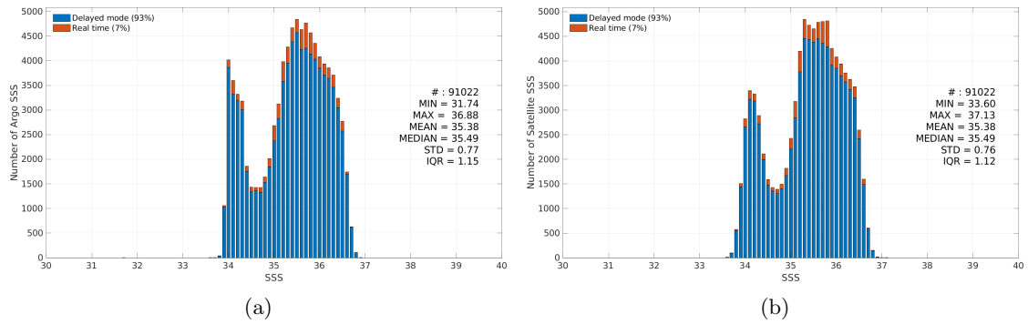
Figure 2: Histograms of SSS from Argo (a) and SMOS SSS L3 v9 - 18 Days (CATDS-CEC-LOCEAN) (b) considering all match-up pairs per bins of 0.1 over the OTT zone Pi-MEP region and for the full satellite product period.
