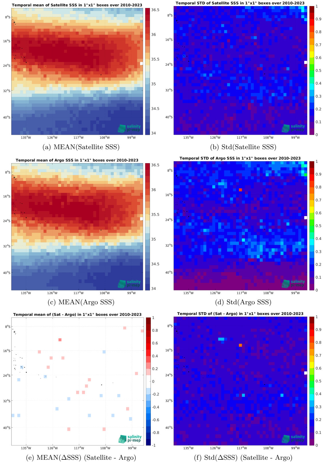
Figure 6: Temporal mean (left) and Std (right) of SSS from SMOS SSS L3 v9 - 18 Days (CATDS-CEC-LOCEAN) (top), Argo (middle), and of \Delta SSS (Satellite - Argo). Only match-up pairs are used to generate these maps.
