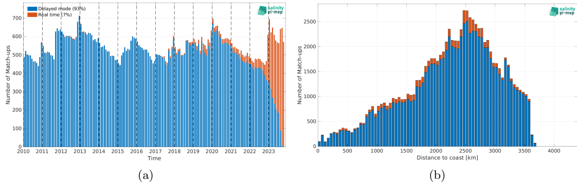
Figure 1: Number of match-ups between Argo and SMOS SSS L3 v9 - 18 Days (CATDS-CEC-LOCEAN) SSS as a function of time (a) and as function of the distance to coast (b) over the OTT zone Pi-MEP region and for the full satellite product period.
