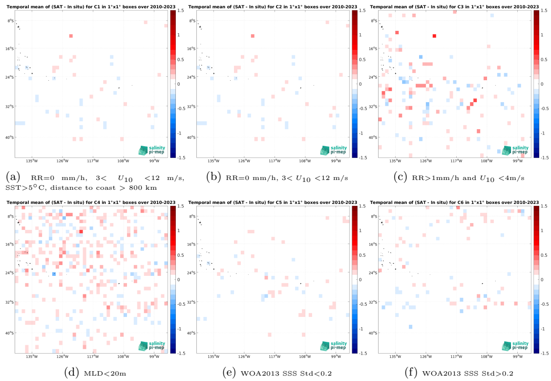
Figure 12: Temporal mean gridded over spatial boxes of size 1^\circ \times 1^\circ of \Delta SSS (SMOS SSS L3 v9 - 18 Days (CATDS-CEC-LOCEAN) - Argo) for 6 different subdatasets corresponding to:RR=0 mm/h, 3 < U_{10} < 12 m/s, SST >5^\circ C, distance to coast > 800 km (a), RR=0 mm/h, 3 < U_{10} < 12 m/s (b), RR >1 mm/h and U_{10} < 4 m/s (c),MLD <20 m (d),WOA2013 SSS Std <0.2 (e),WOA2013 SSS Std >0.2 (f).
