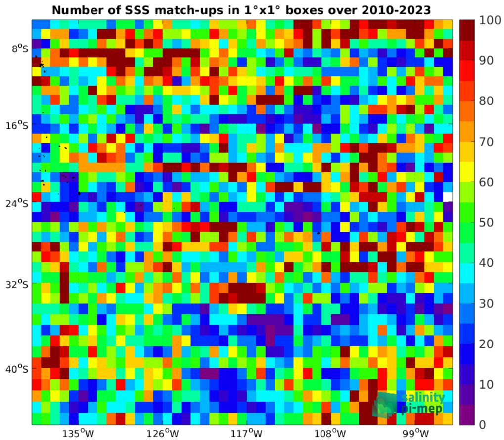
Figure 4: Number of SSS match-ups between Argo SSS and the SMOS SSS L3 v9 - 18 Days (CATDS-CEC-LOCEAN) SSS product for the OTT zone Pi-MEP region over 1°x1° boxes and for the full satellite product period.
