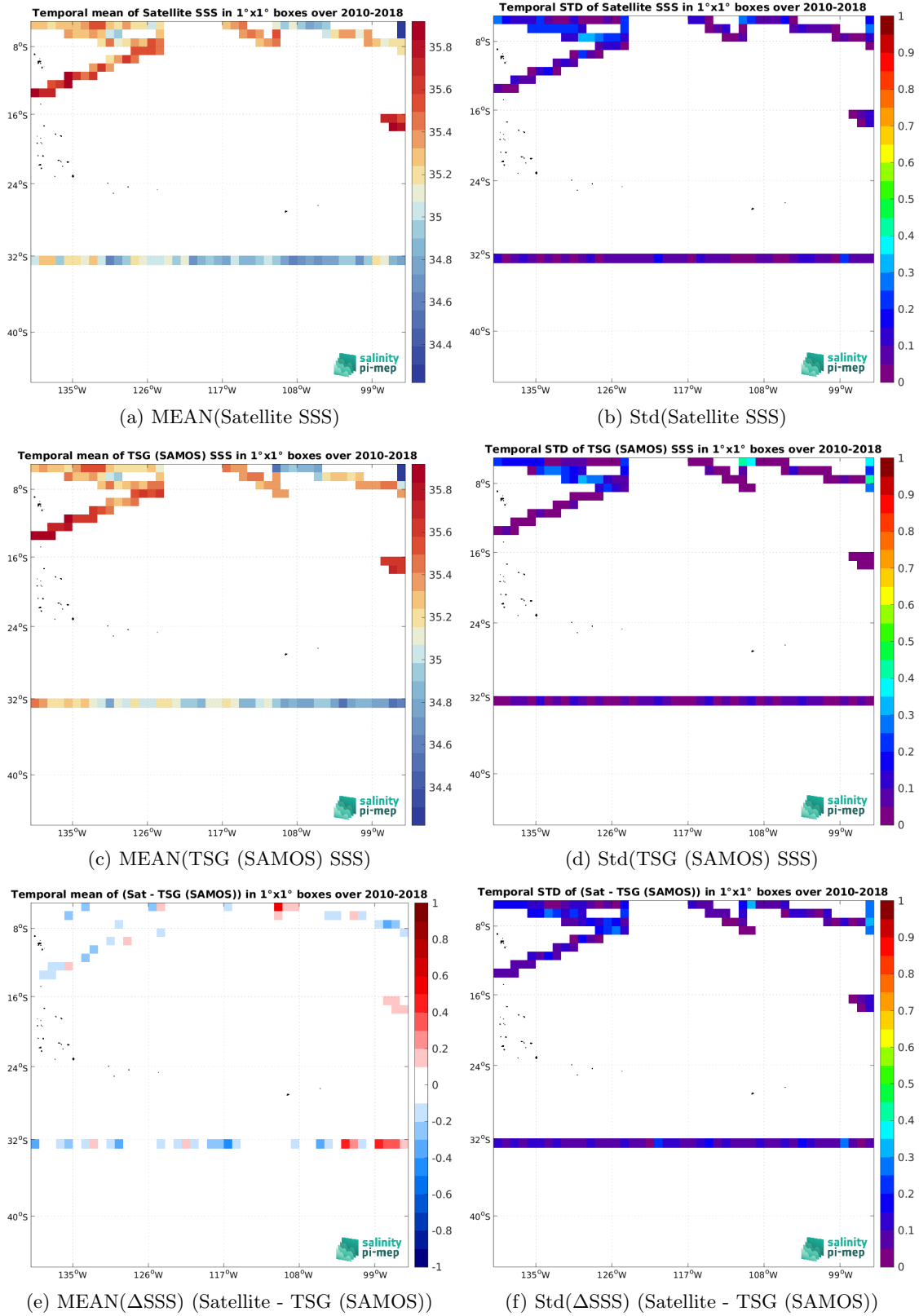
Figure 6: Temporal mean (left) and Std (right) of SSS from SMOS SSS L3 v8 - 9 Days (CATDS-CEC-LOCEAN) (top), TSG (SAMOS) (middle), and of \Delta SSS (Satellite - TSG (SAMOS)). Only match-up pairs are used to generate these maps.
