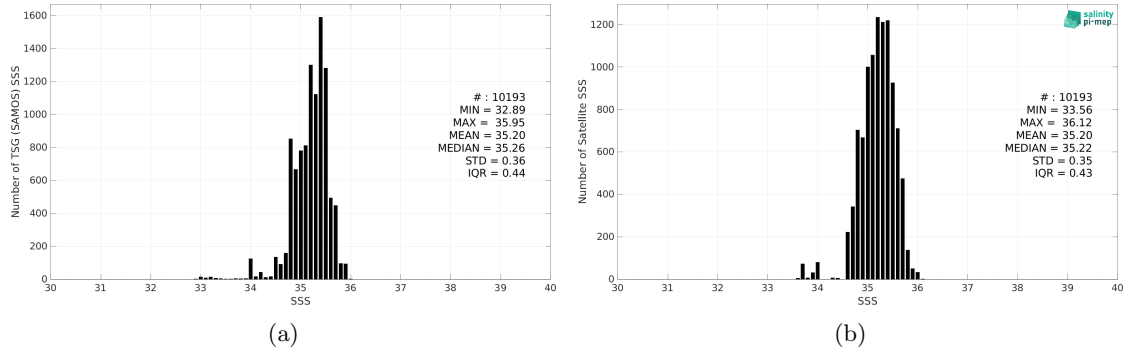
Figure 2: Histograms of SSS from TSG (SAMOS) (a) and SMOS SSS L3 v8 - 9 Days (CATDS-CEC-LOCEAN) (b) considering all match-up pairs per bins of 0.1 over the OTT zone Pi-MEP region and for the full satellite product period.
