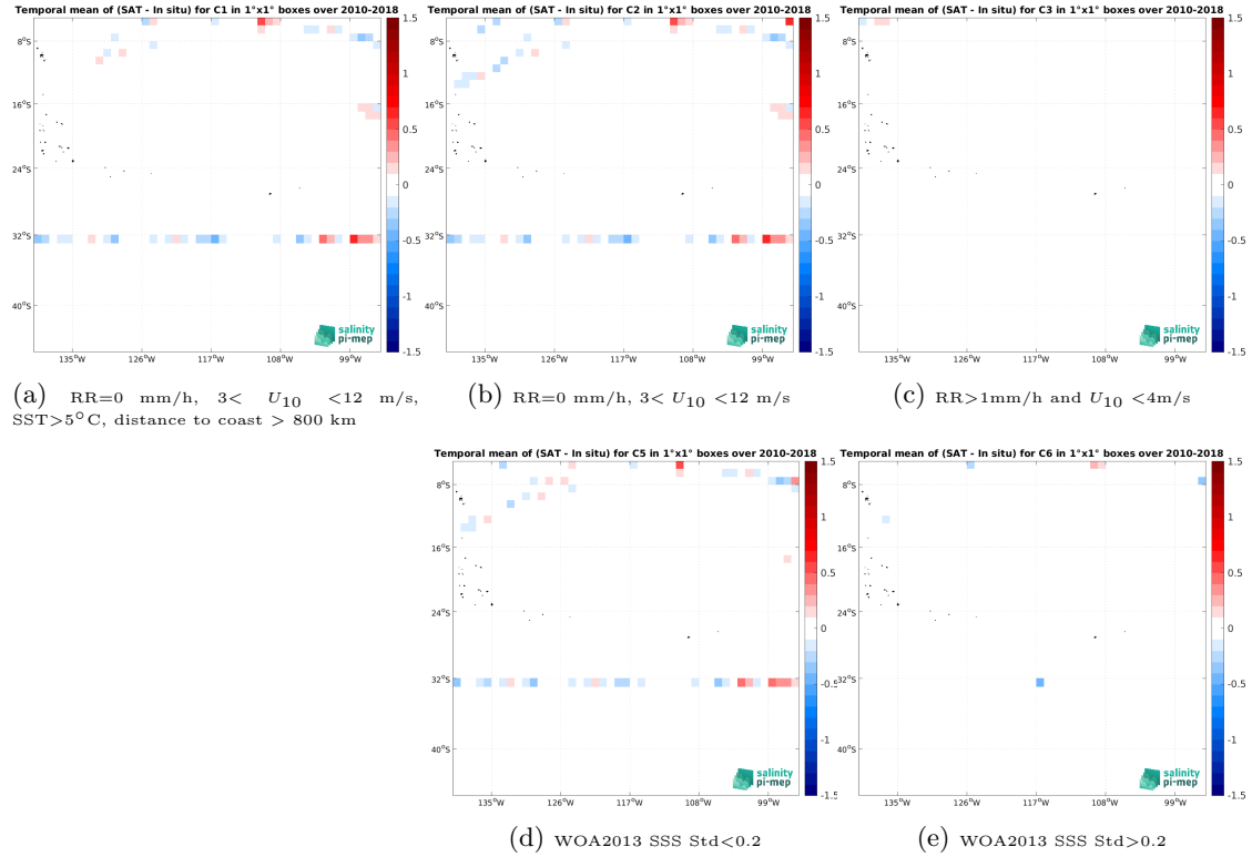
Figure 12: Temporal mean gridded over spatial boxes of size 1^{\circ}\times 1^{\circ} of \Delta\text{SSS} (SMOS SSS L3 v8 - 9 Days (CATDS-CEC-LOCEAN) - TSG (SAMOS)) for 5 different subdatasets corresponding to:RR=0 mm/h, 3 < U_{10} < 12 m/s, SST >5^{\circ}\text{C} , distance to coast > 800 km (a), RR=0 mm/h, 3 < U_{10} < 12 m/s (b), RR >1 mm/h and U_{10} < 4 m/s (c), WOA2013 SSS Std <0.2 (d), WOA2013 SSS Std >0.2 (e).
