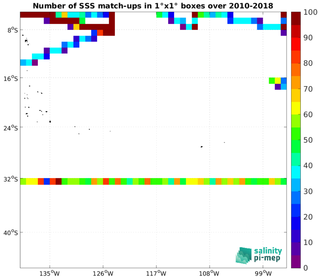
Figure 4: Number of SSS match-ups between TSG (SAMOS) SSS and the SMOS SSS L3 v8 - 9 Days (CATDS-CEC-LOCEAN) SSS product for the OTT zone Pi-MEP region over 1^\circ \times 1^\circ boxes and for the full satellite product period.
