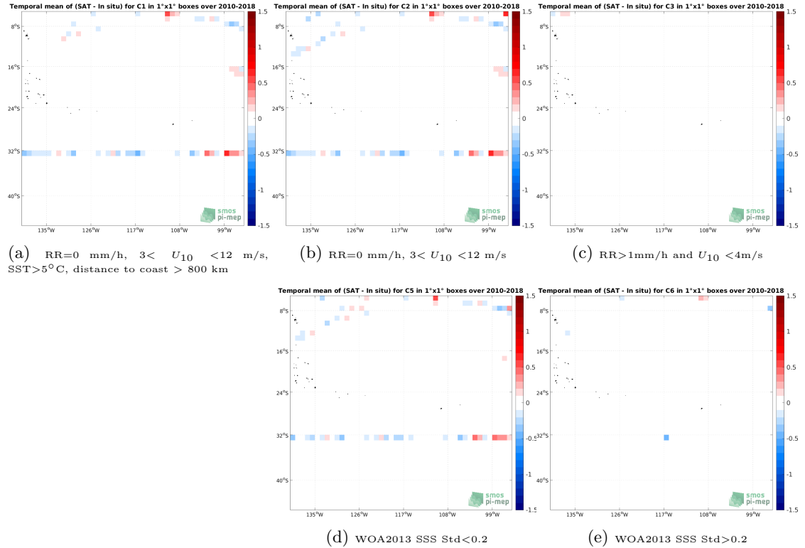
Figure 12: Temporal mean gridded over spatial boxes of size 1^{\circ}\times 1^{\circ} of \Delta\text{SSS} (SMOS SSS L3 v8 - 9 Days (CATDS-CECOS-LOCEAN) - TSG (SAMOS)) for 5 different subdatasets corresponding to: \text{RR}=0 mm/h, 3 < U_{10} < 12 m/s, \text{SST}>5^{\circ}\text{C} , distance to coast > 800 km (a), \text{RR}=0 mm/h, 3 < U_{10} < 12 m/s (b), \text{RR}>1\text{mm/h} and U_{10} < 4\text{m/s} (c), WOA2013 SSS Std < 0.2 (d), WOA2013 SSS Std > 0.2 (e).
