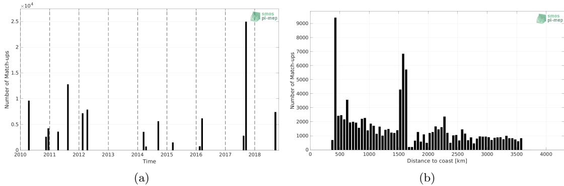
Figure 1: Number of match-ups between TSG (SAMOS) and SMOS SSS L3 v8 - 9 Days (CATDS-CECOS-LOCEAN) SSS as a function of time (a) and as function of the distance to coast (b) over the OTT zone Pi-MEP region and for the full satellite product period.
