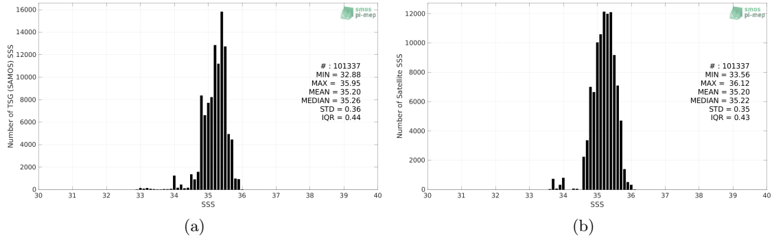
Figure 2: Histograms of SSS from TSG (SAMOS) (a) and SMOS SSS L3 v8 - 9 Days (CATDS-CECOS-LOCEAN) (b) considering all match-up pairs per bins of 0.1 over the OTT zone Pi-MEP region and for the full satellite product period.
