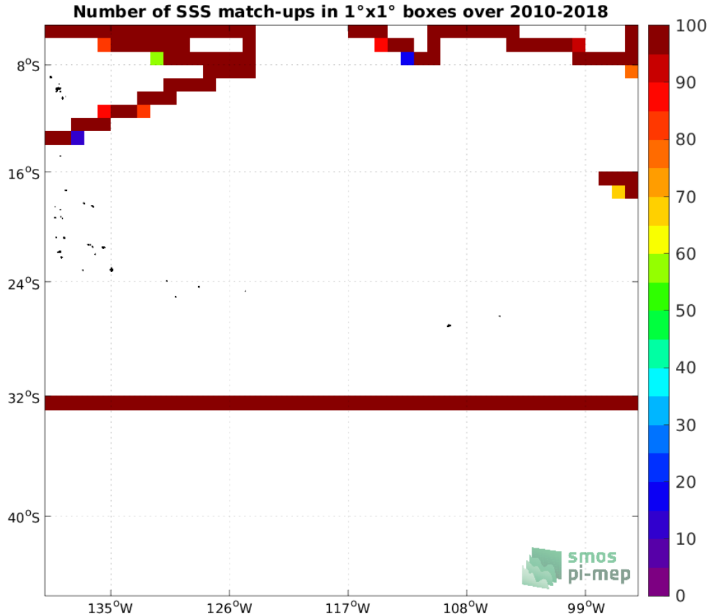
Figure 4: Number of SSS match-ups between TSG (SAMOS) SSS and the SMOS SSS L3 v8 - 9 Days (CATDS-CECOS-LOCEAN) SSS product for the OTT zone Pi-MEP region over 1^\circ \times 1^\circ boxes and for the full satellite product period.
