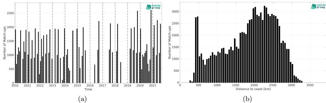
Figure 1: Number of match-ups between TSG (LEGOS-DM) and SMOS SSS L3 v8 - 9 Days (CATDS-CEC-LOCEAN) SSS as a function of time (a) and as function of the distance to coast (b) over the OTT zone Pi-MEP region and for the full satellite product period.
