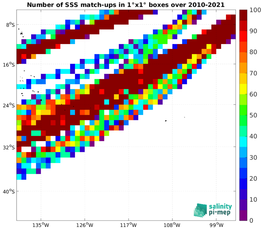
Figure 4: Number of SSS match-ups between TSG (LEGOS-DM) SSS and the SMOS SSS L3 v8 - 9 Days (CATDS-CEC-LOCEAN) SSS product for the OTT zone Pi-MEP region over 1^\circ \times 1^\circ boxes and for the full satellite product period.
