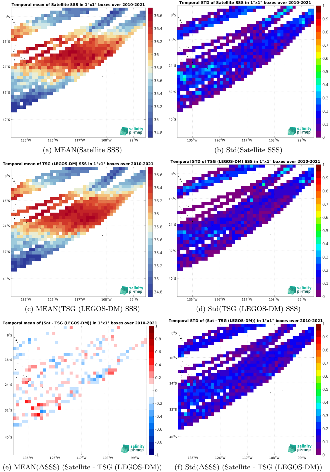
Figure 6: Temporal mean (left) and Std (right) of SSS from SMOS SSS L3 v8 - 9 Days (CATDS-CEC-LOCEAN) (top), TSG (LEGOS-DM) (middle), and of \Delta SSS (Satellite - TSG (LEGOS-DM)). Only match-up pairs are used to generate these maps.
