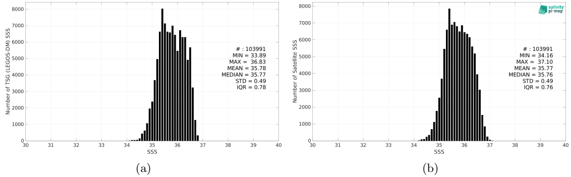
Figure 2: Histograms of SSS from TSG (LEGOS-DM) (a) and SMOS SSS L3 v8 - 9 Days (CATDS-CEC-LOCEAN) (b) considering all match-up pairs per bins of 0.1 over the OTT zone Pi-MEP region and for the full satellite product period.
