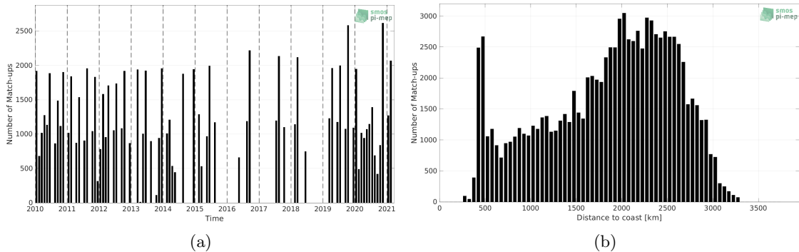
Figure 1: Number of match-ups between TSG (LEGOS-DM) and SMOS SSS L3 v8 - 9 Days (CATDS-CECOS-LOCEAN) SSS as a function of time (a) and as function of the distance to coast (b) over the OTT zone Pi-MEP region and for the full satellite product period.
