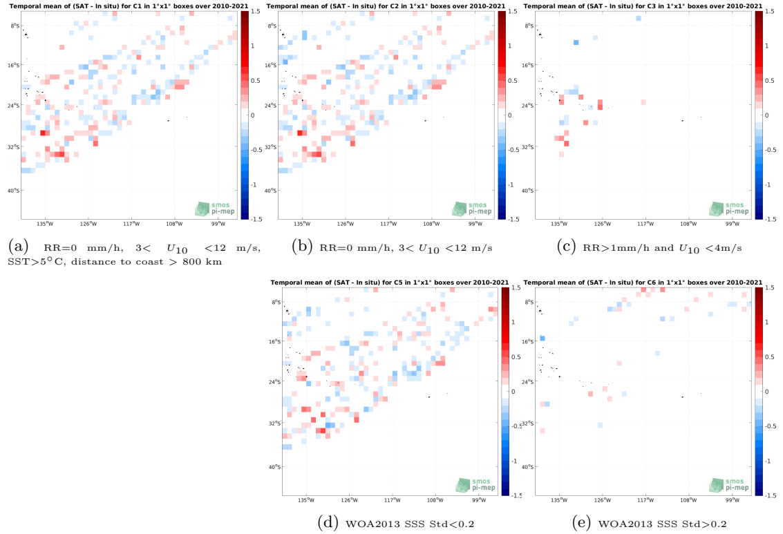
Figure 12: Temporal mean gridded over spatial boxes of size 1^{\circ}\times 1^{\circ} of \Delta\text{SSS} (SMOS SSS L3 v8 - 9 Days (CATDS-CECOS-LOCEAN) - TSG (LEGOS-DM)) for 5 different subdatasets corresponding to:RR=0 mm/h, 3 < U_{10} < 12 m/s, SST >5^{\circ}\text{C} , distance to coast > 800 km (a), RR=0 mm/h, 3 < U_{10} < 12 m/s (b), RR >1 mm/h and U_{10} < 4 m/s (c), WOA2013 SSS Std <0.2 (d), WOA2013 SSS Std >0.2 (e).
