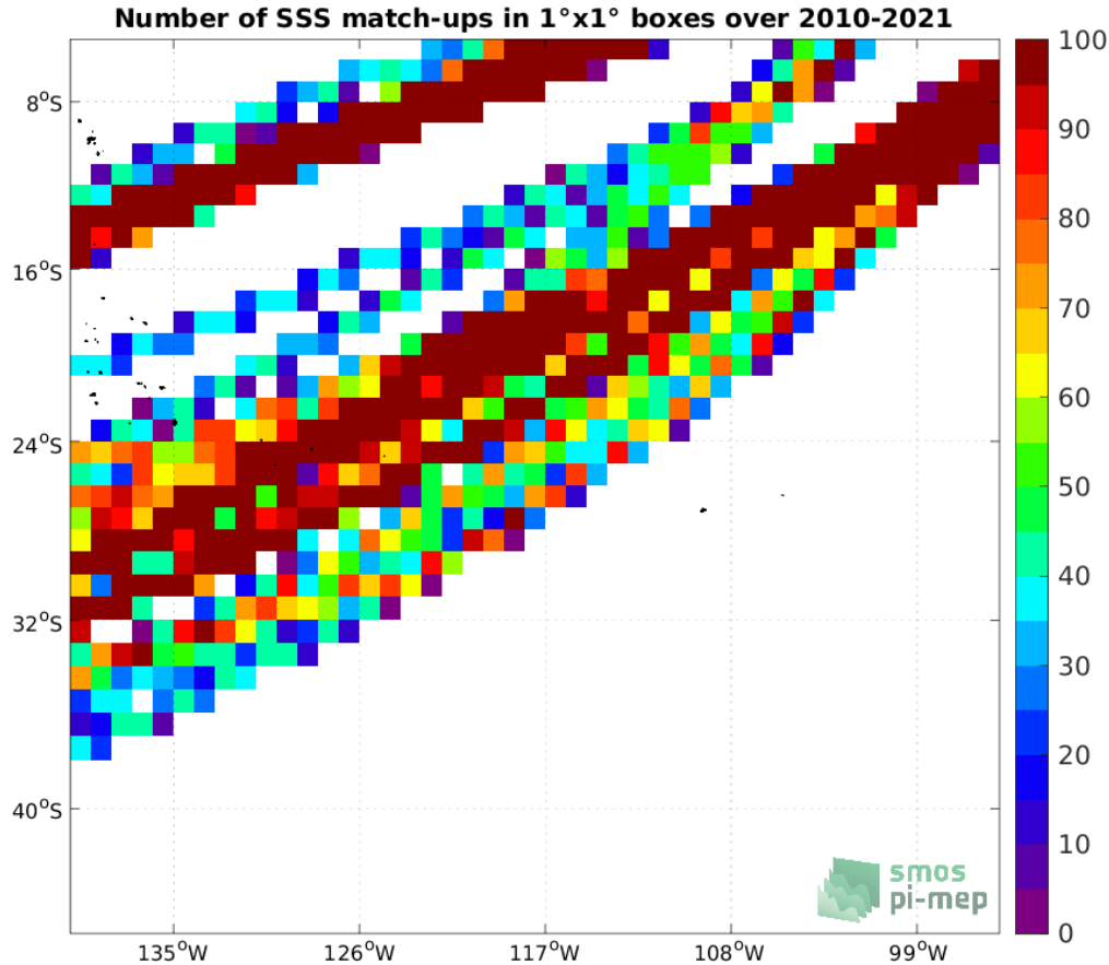
Figure 4: Number of SSS match-ups between TSG (LEGOS-DM) SSS and the SMOS SSS L3 v8 - 9 Days (CATDS-CECOS-LOCEAN) SSS product for the OTT zone Pi-MEP region over 1^\circ \times 1^\circ boxes and for the full satellite product period.
