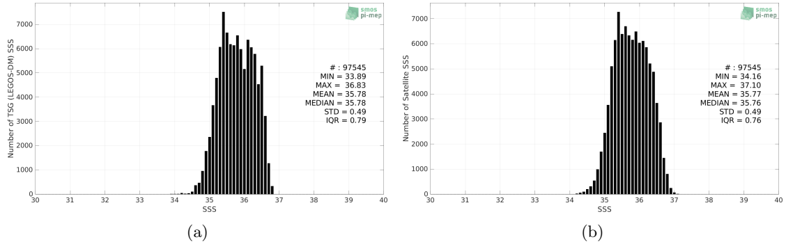
Figure 2: Histograms of SSS from TSG (LEGOS-DM) (a) and SMOS SSS L3 v8 - 9 Days (CATDS-CECOS-LOCEAN) (b) considering all match-up pairs per bins of 0.1 over the OTT zone Pi-MEP region and for the full satellite product period.
