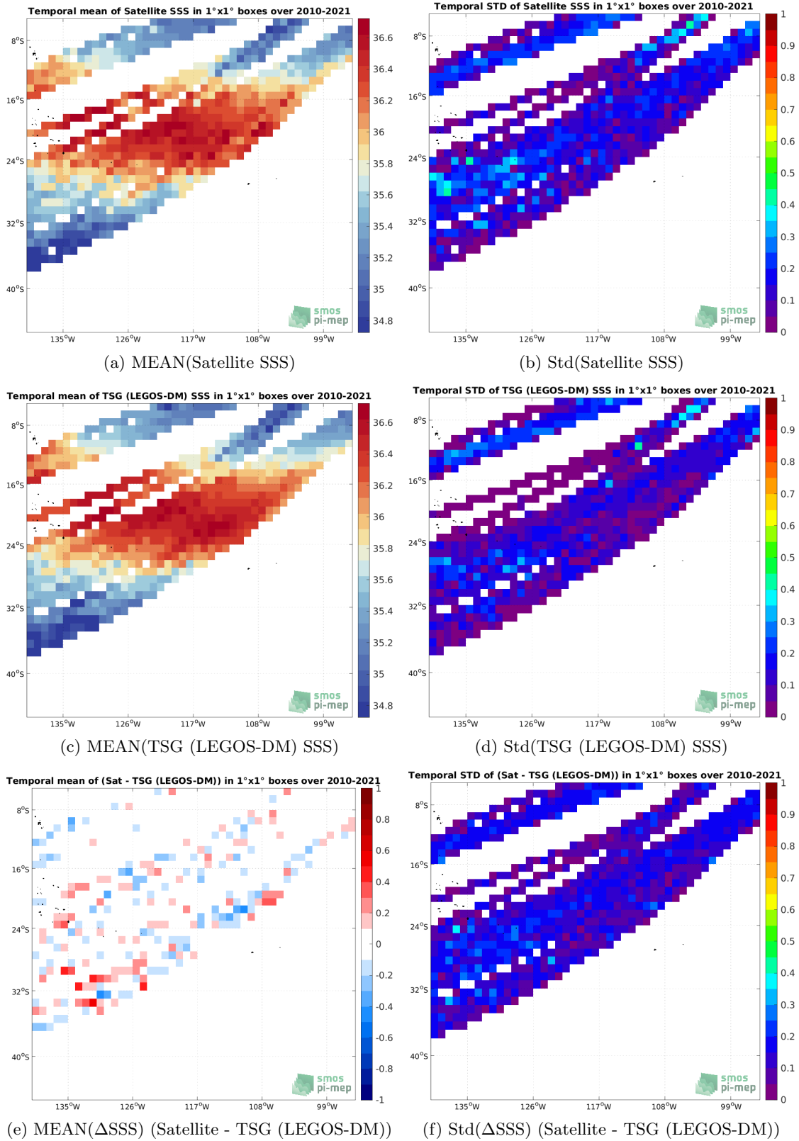
Figure 6: Temporal mean (left) and Std (right) of SSS from SMOS SSS L3 v8 - 9 Days (CATDS-CECOS-LOCEAN) (top), TSG (LEGOS-DM) (middle), and of \Delta SSS (Satellite - TSG (LEGOS-DM)). Only match-up pairs are used to generate these maps.
