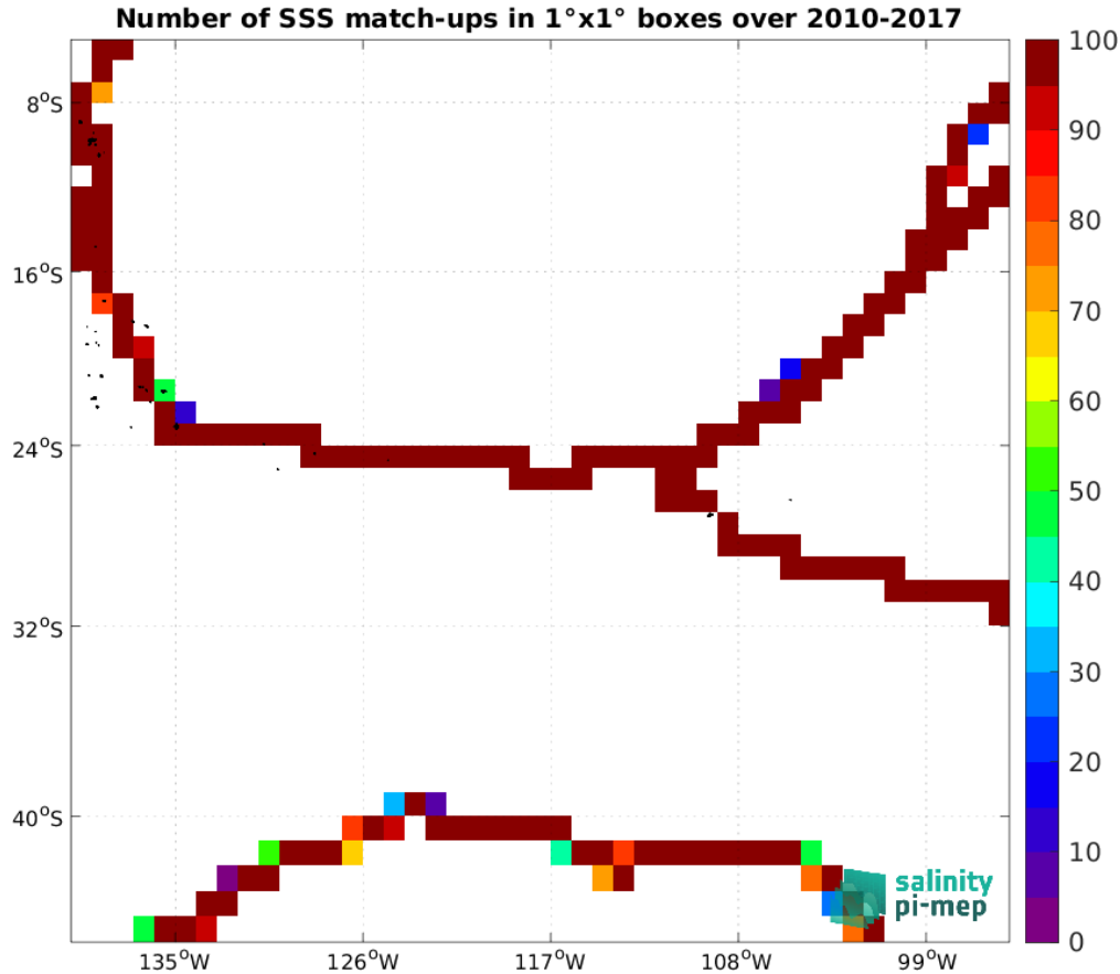
Figure 4: Number of SSS match-ups between TSG (GOSUD-Sailing-ship) SSS and the SMOS SSS L3 v8 - 9 Days (CATDS-CEC-LOCEAN) SSS product for the OTT zone Pi-MEP region over 1^\circ \times 1^\circ boxes and for the full satellite product period.
