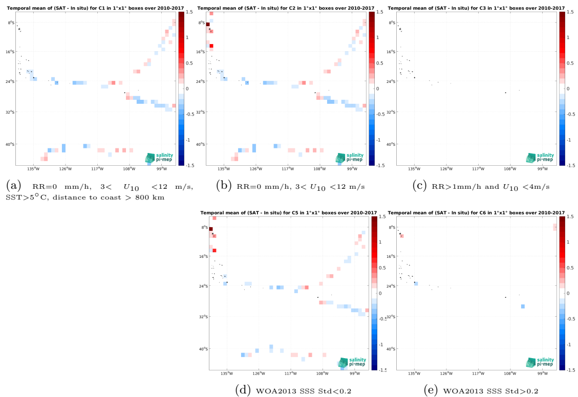
Figure 12: Temporal mean gridded over spatial boxes of size 1^\circ \times 1^\circ of \Delta SSS (SMOS SSS L3 v8 - 9 Days (CATDS-CEC-LOCEAN) - TSG (GOSUD-Sailing-ship)) for 5 different subdatasets corresponding to:RR=0 mm/h, 3 < U_{10} < 12 m/s, SST >5^\circ\text{C} , distance to coast > 800 km (a), RR=0 mm/h, 3 < U_{10} < 12 m/s (b), RR >1 mm/h and U_{10} < 4 m/s (c), WOA2013 SSS Std <0.2 (d), WOA2013 SSS Std >0.2 (e).
