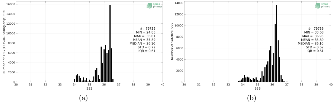
Figure 2: Histograms of SSS from TSG (GOSUD-Sailing-ship) (a) and SMOS SSS L3 v8 - 9 Days (CATDS-CECOS-LOCEAN) (b) considering all match-up pairs per bins of 0.1 over the OTT zone Pi-MEP region and for the full satellite product period.
