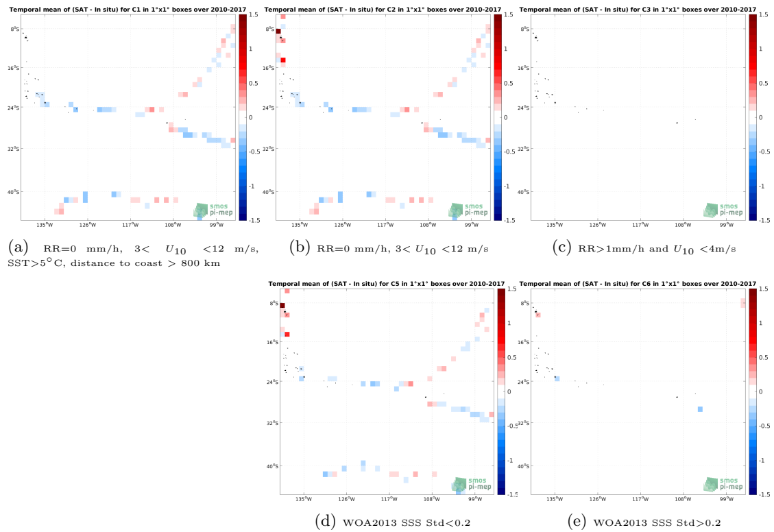
Figure 12: Temporal mean gridded over spatial boxes of size 1^\circ \times 1^\circ of \Delta SSS (SMOS SSS L3 v8 - 9 Days (CATDS-CECOS-LOCEAN) - TSG (GOSUD-Sailing-ship)) for 5 different subdatasets corresponding to:RR=0 mm/h, 3 < U_{10} < 12 m/s, SST >5^\circ\text{C} , distance to coast > 800 km (a), RR=0 mm/h, 3 < U_{10} < 12 m/s (b), RR >1 mm/h and U_{10} < 4 m/s (c), WOA2013 SSS Std <0.2 (d), WOA2013 SSS Std >0.2 (e).
