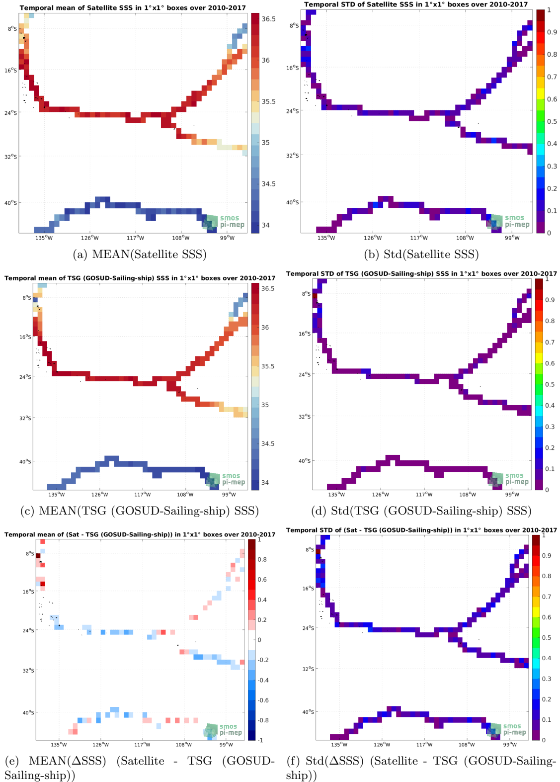
Figure 6: Temporal mean (left) and Std (right) of SSS from SMOS SSS L3 v8 - 9 Days (CATDS-CECOS-LOCEAN) (top), TSG (GOSUD-Sailing-ship) (middle), and of \Delta SSS (Satellite - TSG (GOSUD-Sailing-ship)). Only match-up pairs are used to generate these maps.
