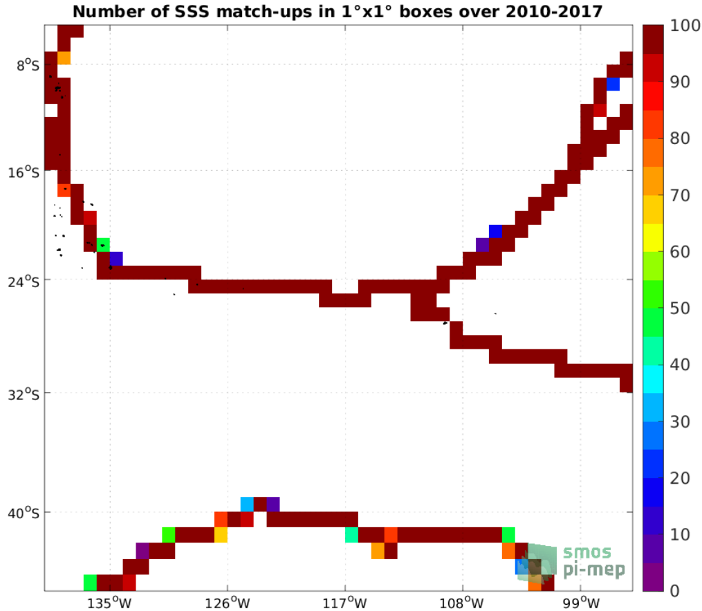
Figure 4: Number of SSS match-ups between TSG (GOSUD-Sailing-ship) SSS and the SMOS SSS L3 v8 - 9 Days (CATDS-CECOS-LOCEAN) SSS product for the OTT zone Pi-MEP region over 1^\circ \times 1^\circ boxes and for the full satellite product period.
