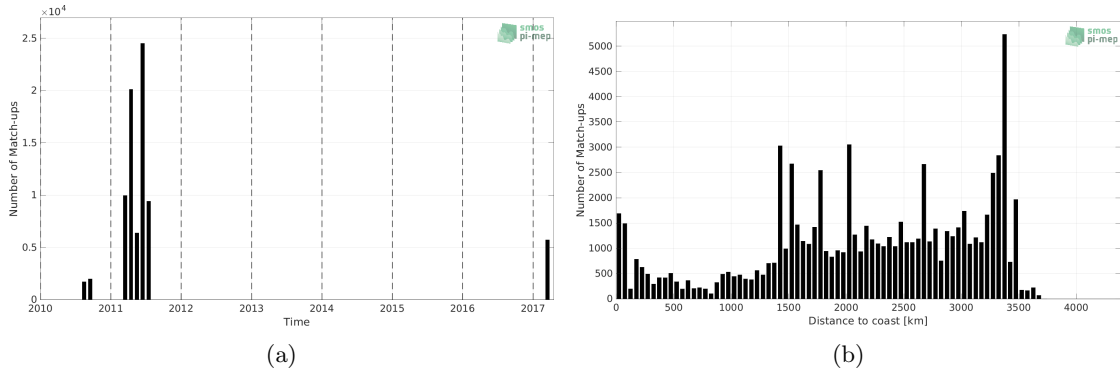
Figure 1: Number of match-ups between TSG (GOSUD-Sailing-ship) and SMOS SSS L3 v8 - 9 Days (CATDS-CECOS-LOCEAN) SSS as a function of time (a) and as function of the distance to coast (b) over the OTT zone Pi-MEP region and for the full satellite product period.
