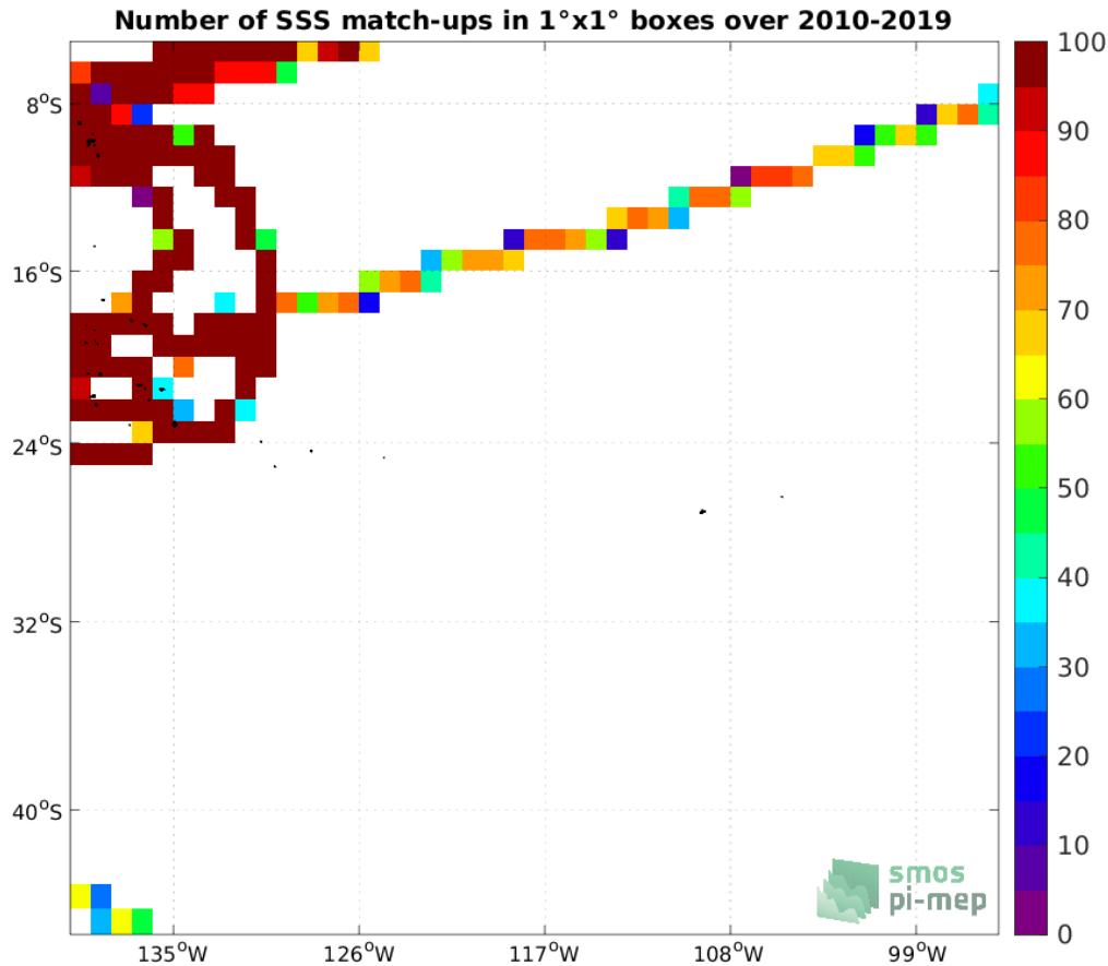
Figure 4: Number of SSS match-ups between TSG (GOSUD-Research-vessel) SSS and the SMOS SSS L3 v8 - 9 Days (CATDS-CECOS-LOCEAN) SSS product for the OTT zone Pi-MEP region over 1^\circ \times 1^\circ boxes and for the full satellite product period.
