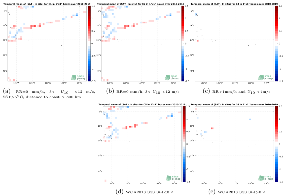
Figure 12: Temporal mean gridded over spatial boxes of size 1^\circ \times 1^\circ of \Delta\text{SSS} (SMOS SSS L3 v8 - 9 Days (CATDS-CECOS-LOCEAN) - TSG (GOSUD-Research-vessel)) for 5 different subdatasets corresponding to:RR=0 mm/h, 3 < U_{10} < 12 m/s, \text{SST} > 5^\circ\text{C} , distance to coast > 800 km (a), RR=0 mm/h, 3 < U_{10} < 12 m/s (b), RR >1 mm/h and U_{10} < 4 m/s (c), WOA2013 SSS Std <0.2 (d), WOA2013 SSS Std >0.2 (e).
