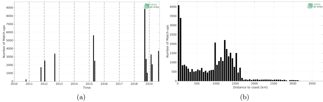
Figure 1: Number of match-ups between TSG (GOSUD-Research-vessel) and SMOS SSS L3 v8 - 9 Days (CATDS-CECOS-LOCEAN) SSS as a function of time (a) and as function of the distance to coast (b) over the OTT zone Pi-MEP region and for the full satellite product period.
