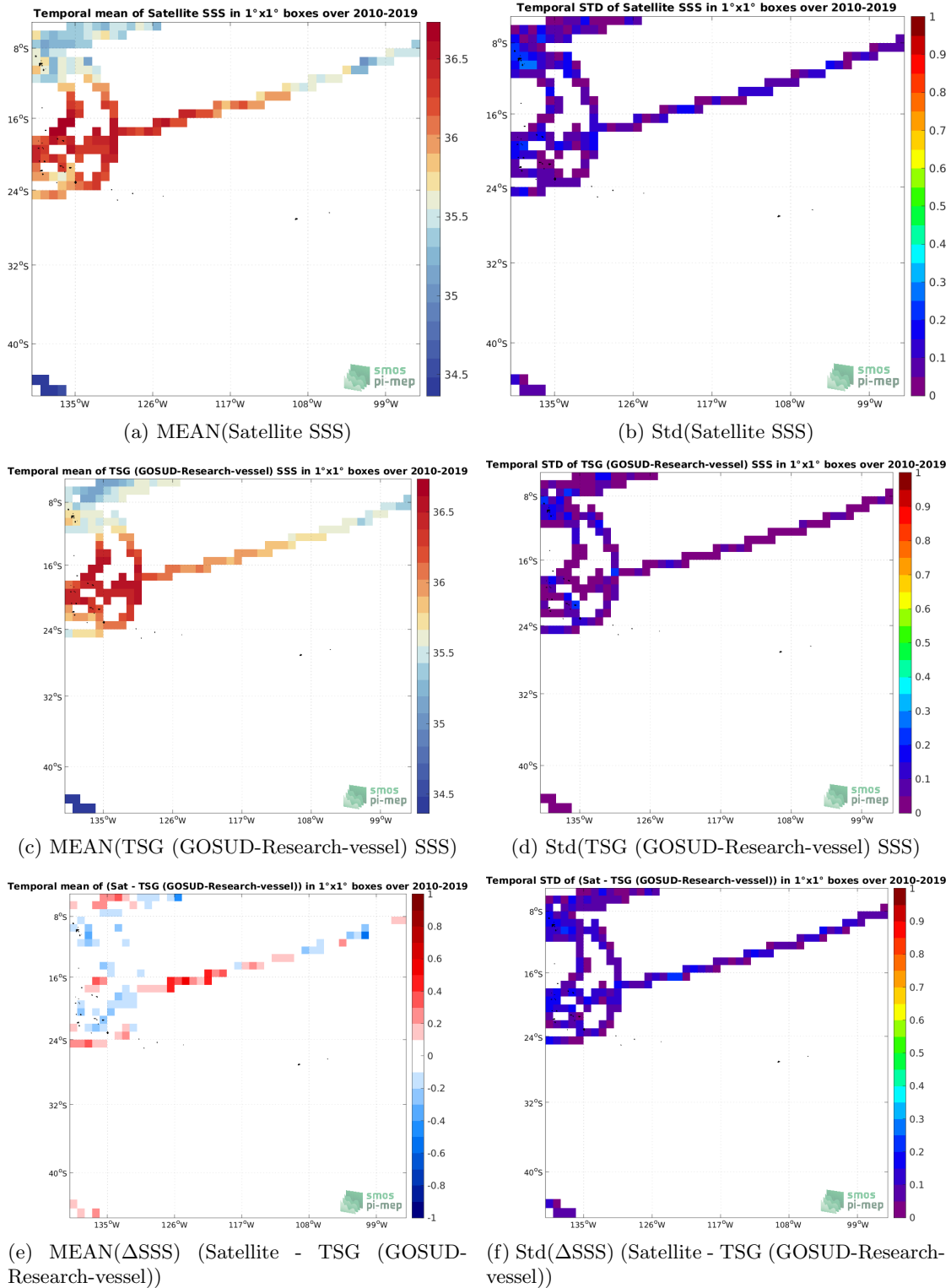
Figure 6: Temporal mean (left) and Std (right) of SSS from SMOS SSS L3 v8 - 9 Days (CATDS-CECOS-LOCEAN) (top), TSG (GOSUD-Research-vessel) (middle), and of \Delta SSS (Satellite - TSG (GOSUD-Research-vessel)). Only match-up pairs are used to generate these maps.
