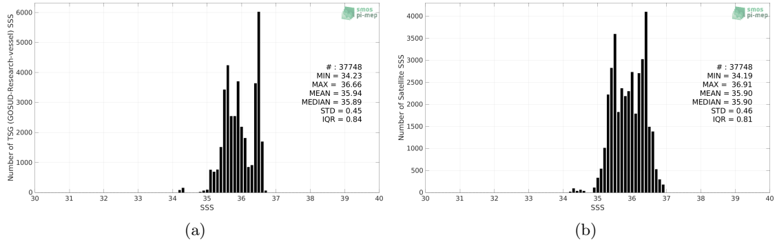
Figure 2: Histograms of SSS from TSG (GOSUD-Research-vessel) (a) and SMOS SSS L3 v8 - 9 Days (CATDS-CECOS-LOCEAN) (b) considering all match-up pairs per bins of 0.1 over the OTT zone Pi-MEP region and for the full satellite product period.
