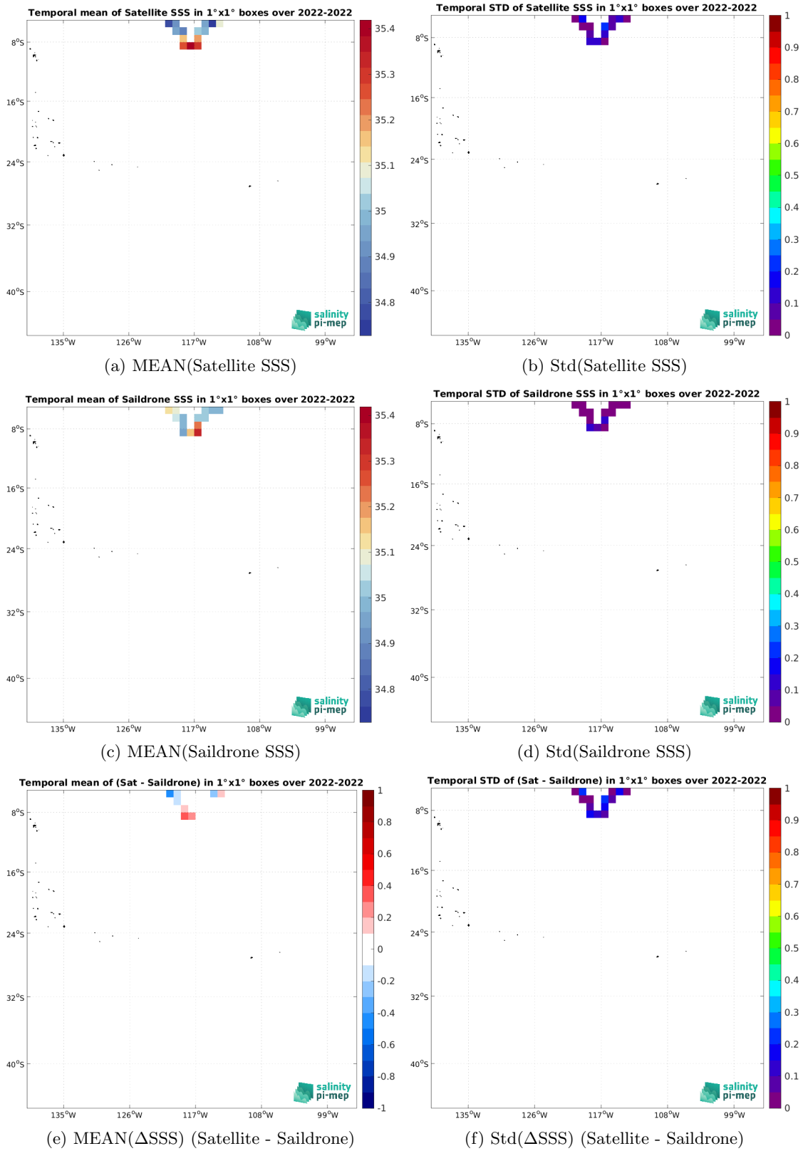
Figure 6: Temporal mean (left) and Std (right) of SSS from SMOS SSS L3 v8 - 9 Days (CATDS-CEC-LOCEAN) (top), Saildrone (middle), and of \Delta SSS (Satellite - Saildrone). Only match-up pairs are used to generate these maps.
