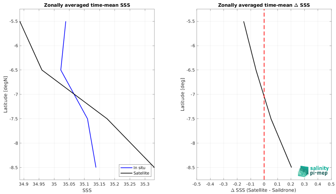
Figure 8: Left panel: Zonal mean SSS from SMOS SSS L3 v8 - 9 Days (CATDS-CEC-LOCEAN) satellite product (black) and from Sairdrone (blue). Right panel: Zonal mean of \Delta SSS (Satellite - Sairdrone) for all the collected Pi-MEP match-up pairs estimated over the full satellite product period.
