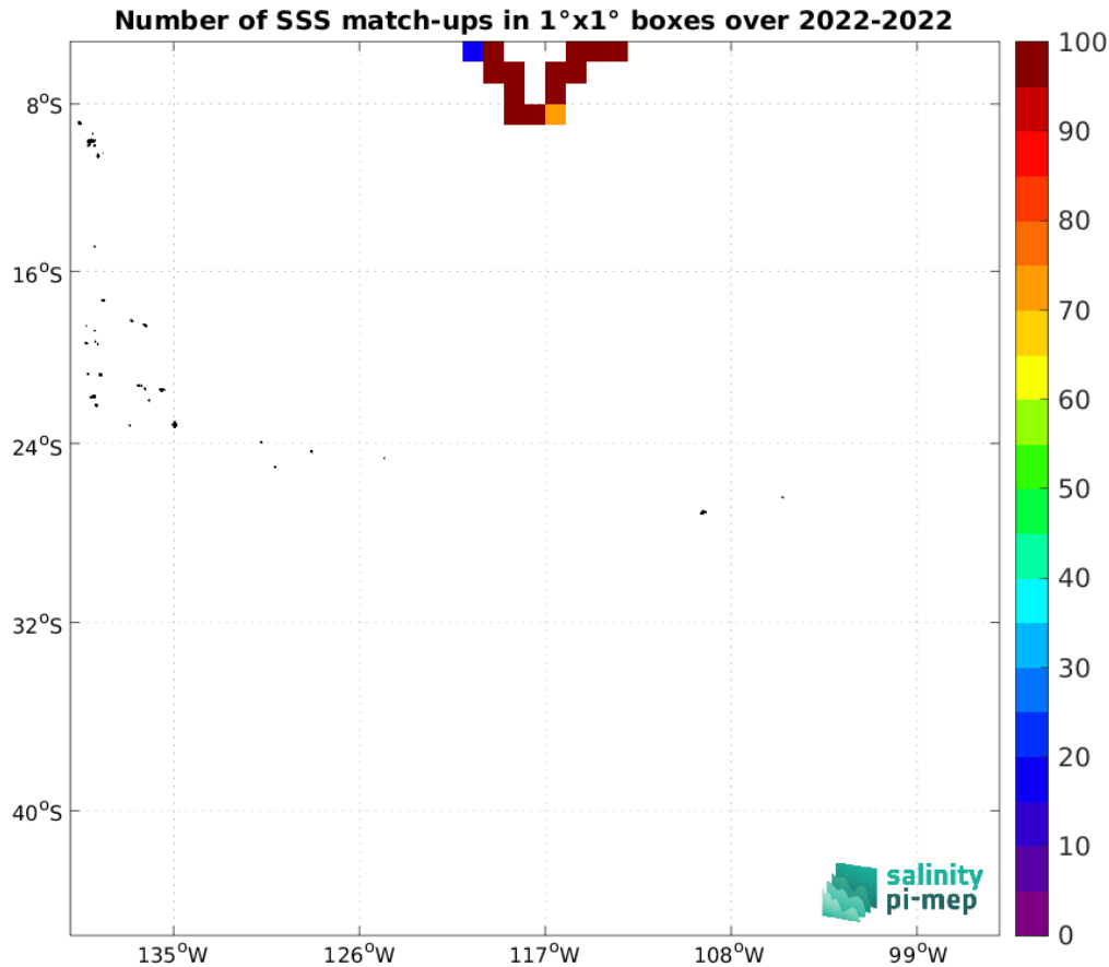
Figure 4: Number of SSS match-ups between Saildrone SSS and the SMOS SSS L3 v8 - 9 Days (CATDS-CEC-LOCEAN) SSS product for the OTT zone Pi-MEP region over 1^\circ \times 1^\circ boxes and for the full satellite product period.
