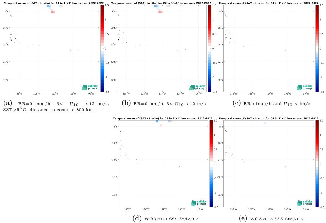
Figure 12: Temporal mean gridded over spatial boxes of size 1^\circ \times 1^\circ of \Delta SSS (SMOS SSS L3 v8 - 9 Days (CATDS-CEC-LOCEAN) - Saildrone) for 5 different subdatasets corresponding to:RR=0 mm/h, 3 < U_{10} < 12 m/s, SST >5^\circ C, distance to coast > 800 km (a), RR=0 mm/h, 3 < U_{10} < 12 m/s (b), RR >1 mm/h and U_{10} < 4 m/s (c), WOA2013 SSS Std <0.2 (d), WOA2013 SSS Std >0.2 (e).
