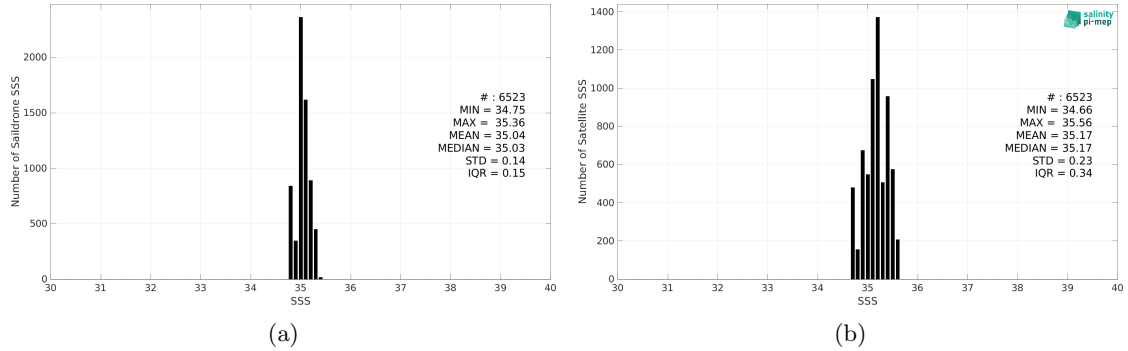
Figure 2: Histograms of SSS from Saildrone (a) and SMOS SSS L3 v8 - 9 Days (CATDS-CEC-LOCEAN) (b) considering all match-up pairs per bins of 0.1 over the OTT zone Pi-MEP region and for the full satellite product period.
