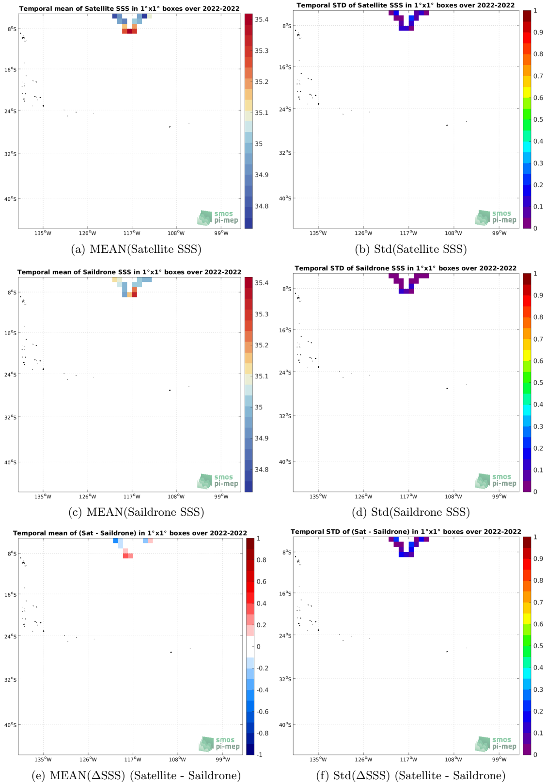
Figure 6: Temporal mean (left) and Std (right) of SSS from SMOS SSS L3 v8 - 9 Days (CATDS-CECOS-LOCEAN) (top), Saildrone (middle), and of \Delta SSS (Satellite - Saildrone). Only match-pairs are used to generate these maps.
