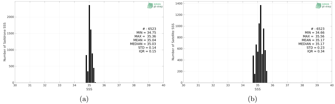
Figure 2: Histograms of SSS from Saildrone (a) and SMOS SSS L3 v8 - 9 Days (CATDS-CECOS-LOCEAN) (b) considering all match-up pairs per bins of 0.1 over the OTT zone Pi-MEP region and for the full satellite product period.
