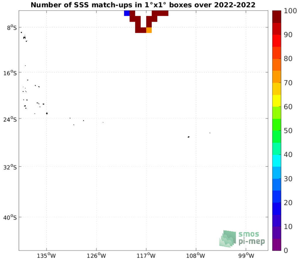
Figure 4: Number of SSS match-ups between Saildrone SSS and the SMOS SSS L3 v8 - 9 Days (CATDS-CECOS-LOCEAN) SSS product for the OTT zone Pi-MEP region over 1^\circ \times 1^\circ boxes and for the full satellite product period.
