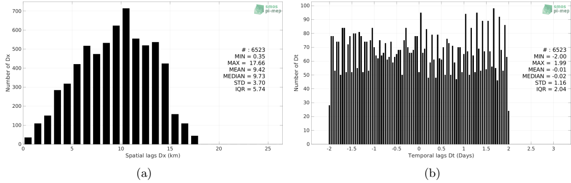
Figure 5: Histograms of the spatial (a) and temporal (b) lags between the location/time of the Sairdrone measurement and the date of the corresponding SMOS SSS L3 v8 - 9 Days (CATDS-CECOS-LOCEAN) SSS pixel.
