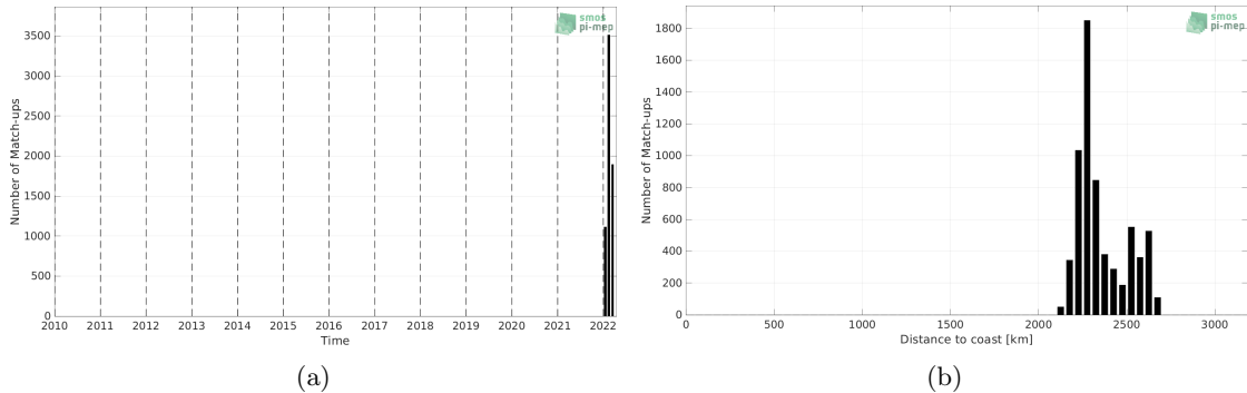
Figure 1: Number of match-ups between Saildrone and SMOS SSS L3 v8 - 9 Days (CATDS-CECOS-LOCEAN) SSS as a function of time (a) and as function of the distance to coast (b) over the OTT zone Pi-MEP region and for the full satellite product period.
