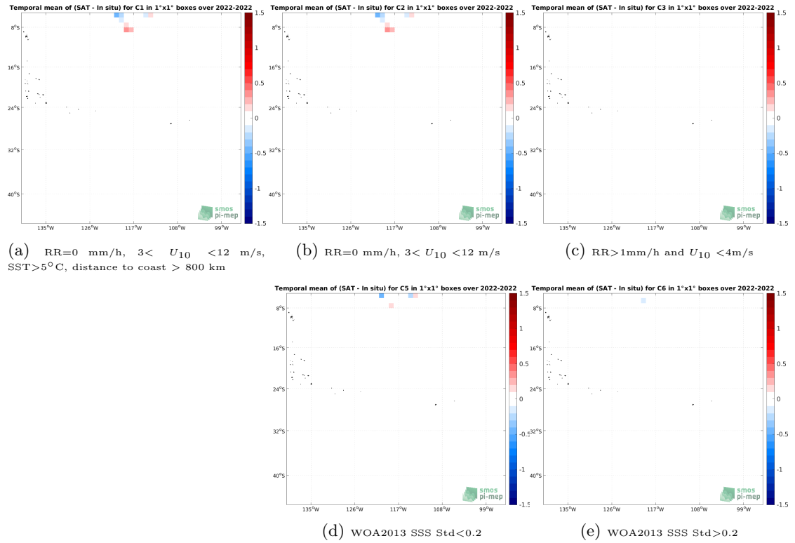
Figure 12: Temporal mean gridded over spatial boxes of size 1^\circ \times 1^\circ of \Delta SSS (SMOS SSS L3 v8 - 9 Days (CATDS-CECOS-LOCEAN) - Saildrone) for 5 different subdatasets corresponding to:RR=0 mm/h, 3 < U_{10} < 12 m/s, SST >5^\circ C, distance to coast > 800 km (a), RR=0 mm/h, 3 < U_{10} < 12 m/s (b), RR >1 mm/h and U_{10} < 4 m/s (c), WOA2013 SSS Std <0.2 (d), WOA2013 SSS Std >0.2 (e).
