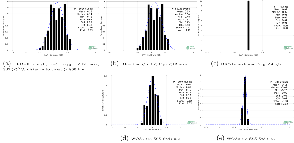
Figure 13: Normalized histogram of \Delta SSS (SMOS SSS L3 v8 - 9 Days (CATDS-CECOS-LOCEAN) - Saildrone) for 5 different subdatasets corresponding to: RR=0 mm/h, 3 < U_{10} < 12 m/s, SST > 5°C, distance to coast > 800 km (a), RR=0 mm/h, 3 < U_{10} < 12 m/s (b), RR > 1mm/h and U_{10} < 4 m/s (c), WOA2013 SSS Std < 0.2 (d), WOA2013 SSS Std > 0.2 (e).
