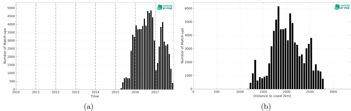
Figure 1: Number of match-ups between Surface drifters and SMOS SSS L3 v8 - 9 Days (CATDS-CEC-LOCEAN) SSS as a function of time (a) and as function of the distance to coast (b) over the OTT zone Pi-MEP region and for the full satellite product period.
