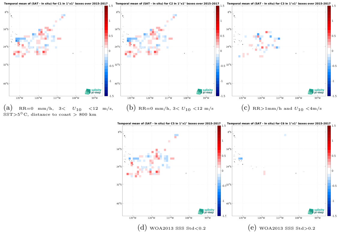
Figure 11: Temporal mean gridded over spatial boxes of size 1^{\circ}\times 1^{\circ} of \Delta\text{SSS} (SMOS SSS L3 v8 - 9 Days (CATDS-CEC-LOCEAN) - Surface drifters) for 5 different subdatasets corresponding to:RR=0 mm/h, 3 < U_{10} < 12 m/s, SST >5^{\circ}\text{C} , distance to coast > 800 km (a), RR=0 mm/h, 3 < U_{10} < 12 m/s (b), RR >1 mm/h and U_{10} < 4 m/s (c), WOA2013 SSS Std <0.2 (d), WOA2013 SSS Std >0.2 (e).
