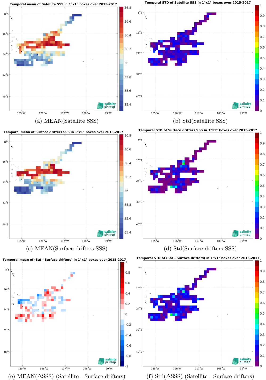
Figure 5: Temporal mean (left) and Std (right) of SSS from SMOS SSS L3 v8 - 9 Days (CATDS-CEC-LOCEAN) (top), Surface drifters (middle), and of \Delta SSS (Satellite - Surface drifters). Only match-up pairs are used to generate these maps.
