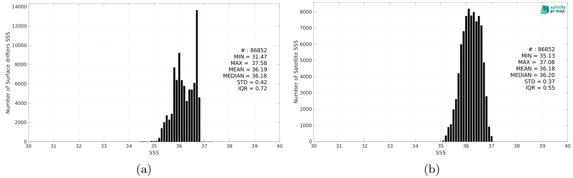
Figure 2: Histograms of SSS from Surface drifters (a) and SMOS SSS L3 v8 - 9 Days (CATDS-CEC-LOCEAN) (b) considering all match-up pairs per bins of 0.1 over the OTT zone Pi-MEP region and for the full satellite product period.
