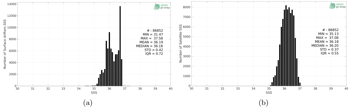
Figure 2: Histograms of SSS from Surface drifters (a) and SMOS SSS L3 v8 - 9 Days (CATDS-CECOS-LOCEAN) (b) considering all match-up pairs per bins of 0.1 over the OTT zone Pi-MEP region and for the full satellite product period.
