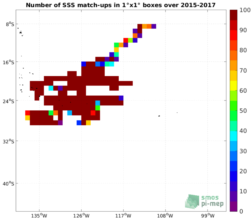
Figure 3: Number of SSS match-ups between Surface drifters SSS and the SMOS SSS L3 v8 - 9 Days (CATDS-CECOS-LOCEAN) SSS product for the OTT zone Pi-MEP region over 1°x1° boxes and for the full satellite product period.
