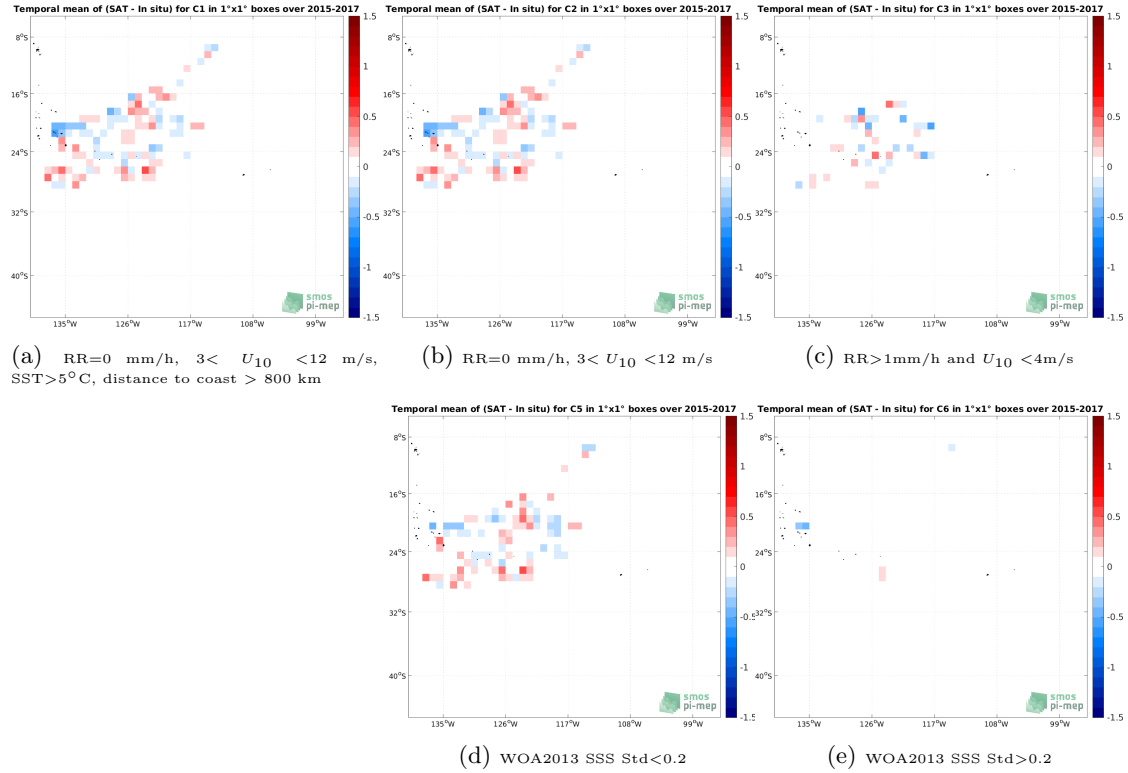
Figure 11: Temporal mean gridded over spatial boxes of size 1^{\circ}\times 1^{\circ} of \Delta\text{SSS} (SMOS SSS L3 v8 - 9 Days (CATDS-CECOS-LOCEAN) - Surface drifters) for 5 different subdatasets corresponding to:RR=0 mm/h, 3 < U_{10} < 12 m/s, SST >5^{\circ}\text{C} , distance to coast > 800 km (a), RR=0 mm/h, 3 < U_{10} < 12 m/s (b), RR >1 mm/h and U_{10} < 4 m/s (c), WOA2013 SSS Std <0.2 (d), WOA2013 SSS Std >0.2 (e).
