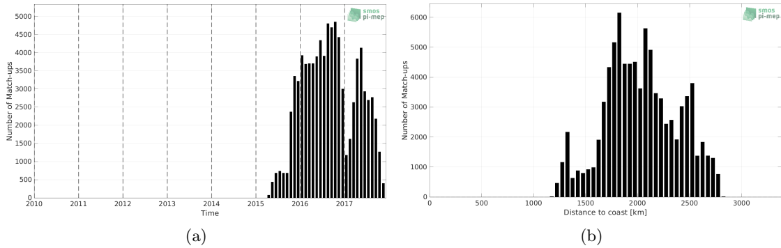
Figure 1: Number of match-ups between Surface drifters and SMOS SSS L3 v8 - 9 Days (CATDS-CECOS-LOCEAN) SSS as a function of time (a) and as function of the distance to coast (b) over the OTT zone Pi-MEP region and for the full satellite product period.
