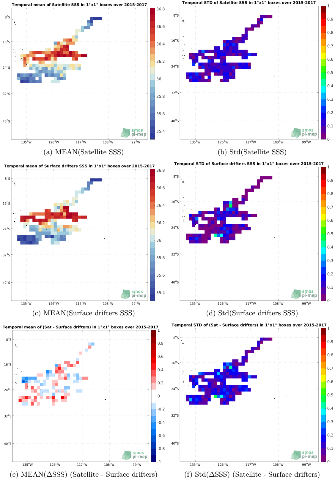
Figure 5: Temporal mean (left) and Std (right) of SSS from SMOS SSS L3 v8 - 9 Days (CATDS-CECOS-LOCEAN) (top), Surface drifters (middle), and of \Delta SSS (Satellite - Surface drifters). Only match-up pairs are used to generate these maps.
