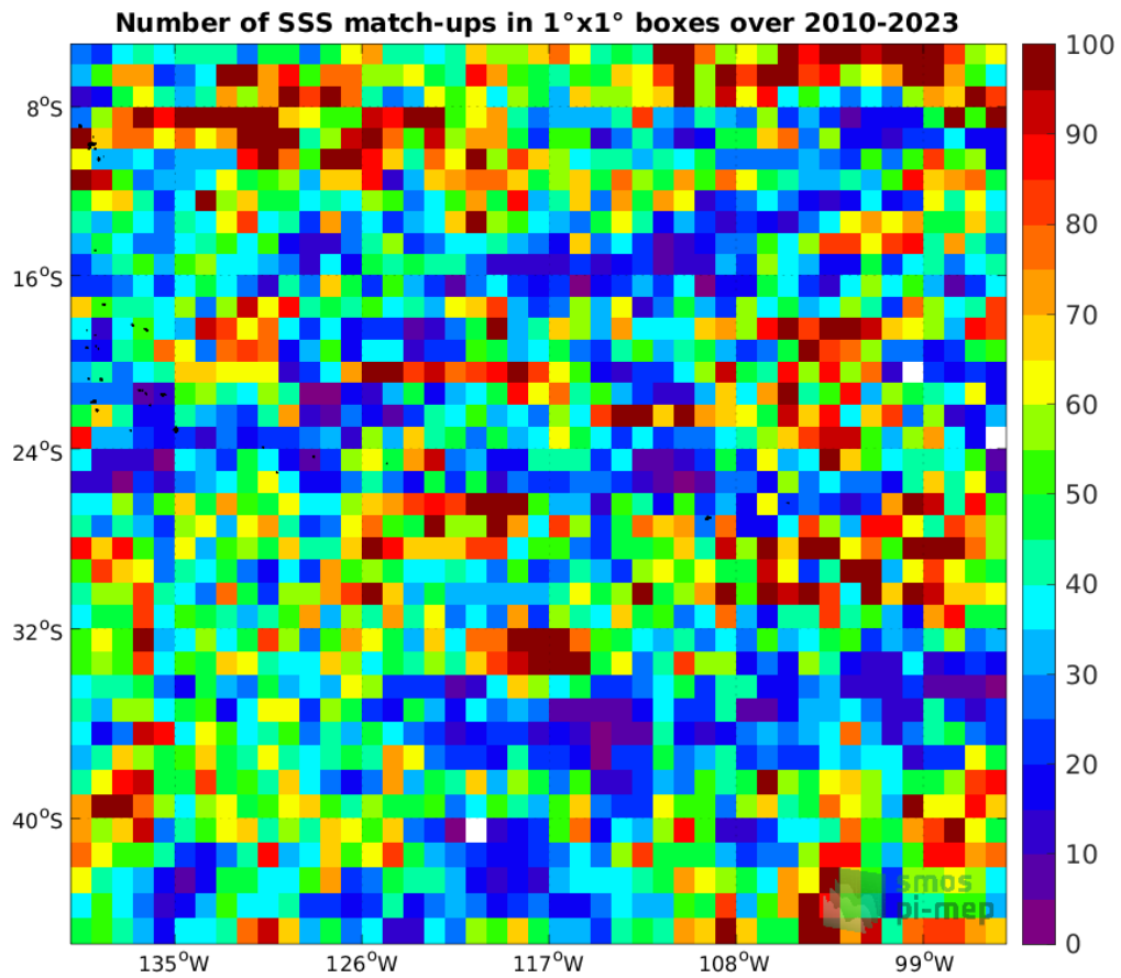
Figure 4: Number of SSS match-ups between Argo SSS and the SMOS SSS L3 v8 - 9 Days (CATDS-CECOS-LOCEAN) SSS product for the OTT zone Pi-MEP region over 1°x1° boxes and for the full satellite product period.
