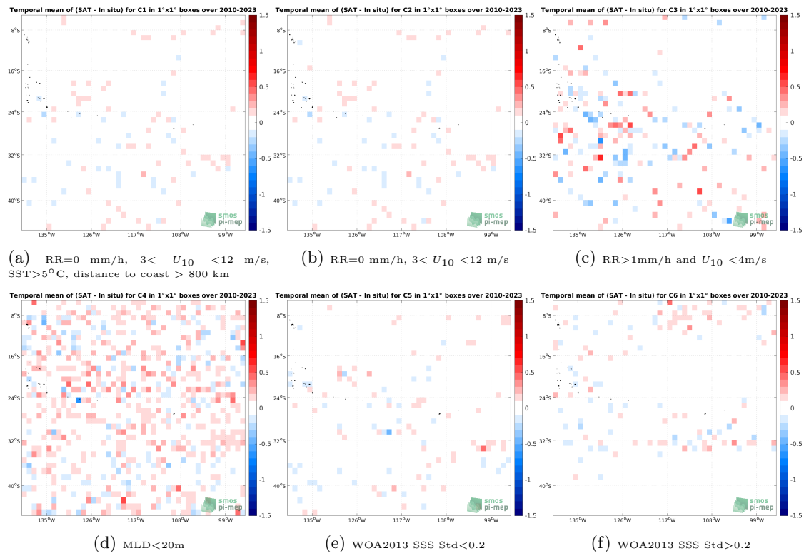
Figure 12: Temporal mean gridded over spatial boxes of size 1^\circ \times 1^\circ of \Delta SSS (SMOS SSS L3 v8 - 9 Days (CATDS-CECOS-LOCEAN) - Argo) for 6 different subdatasets corresponding to:RR=0 mm/h, 3 < U_{10} < 12 m/s, SST >5^\circ C, distance to coast > 800 km (a), RR=0 mm/h, 3 < U_{10} < 12 m/s (b), RR >1 mm/h and U_{10} < 4 m/s (c),MLD <20 m (d),WOA2013 SSS Std <0.2 (e),WOA2013 SSS Std >0.2 (f).
