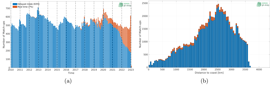
Figure 1: Number of match-ups between Argo and SMOS SSS L3 v8 - 9 Days (CATDS-CECOS-LOCEAN) SSS as a function of time (a) and as function of the distance to coast (b) over the OTT zone Pi-MEP region and for the full satellite product period.
