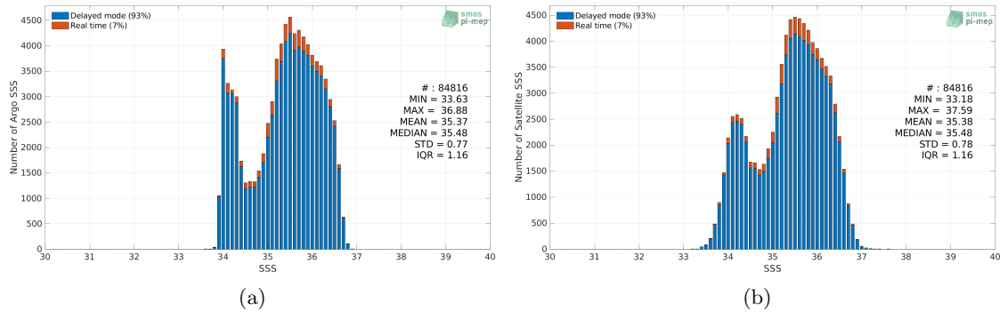
Figure 2: Histograms of SSS from Argo (a) and SMOS SSS L3 v8 - 9 Days (CATDS-CECOS-LOCEAN) (b) considering all match-up pairs per bins of 0.1 over the OTT zone Pi-MEP region and for the full satellite product period.
