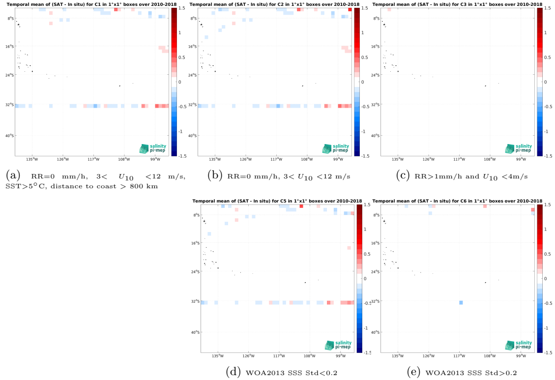
Figure 12: Temporal mean gridded over spatial boxes of size 1^{\circ}\times 1^{\circ} of \Delta\text{SSS} (SMOS SSS L3 v8 - 18 Days (CATDS-CEC-LOCEAN) - TSG (SAMOS)) for 5 different subdatasets corresponding to:RR=0 mm/h, 3 < U_{10} < 12 m/s, SST >5^{\circ}\text{C} , distance to coast > 800 km (a), RR=0 mm/h, 3 < U_{10} < 12 m/s (b), RR >1\text{mm/h} and U_{10} < 4\text{m/s} (c), WOA2013 SSS Std <0.2 (d), WOA2013 SSS Std >0.2 (e).
