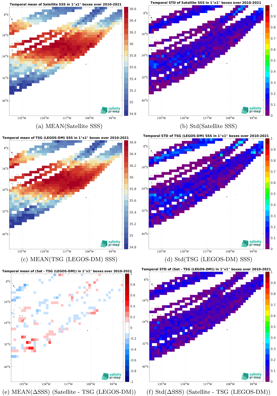
Figure 6: Temporal mean (left) and Std (right) of SSS from SMOS SSS L3 v8 - 18 Days (CATDS-CEC-LOCEAN) (top), TSG (LEGOS-DM) (middle), and of \Delta SSS (Satellite - TSG (LEGOS-DM)). Only match-up pairs are used to generate these maps.
