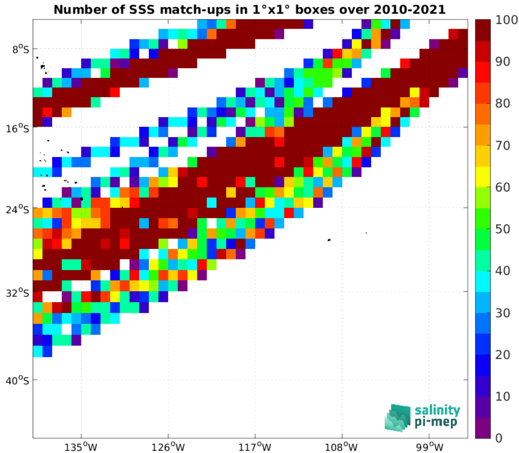
Figure 4: Number of SSS match-ups between TSG (LEGOS-DM) SSS and the SMOS SSS L3 v8 - 18 Days (CATDS-CEC-LOCEAN) SSS product for the OTT zone Pi-MEP region over 1^\circ \times 1^\circ boxes and for the full satellite product period.
