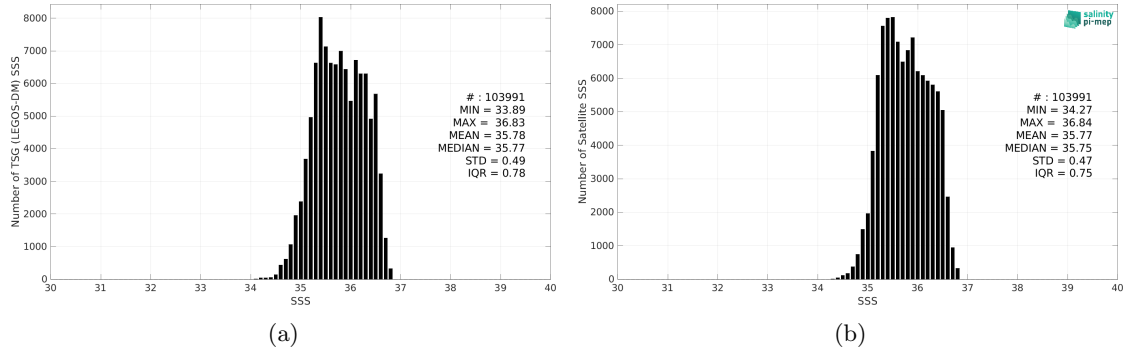
Figure 2: Histograms of SSS from TSG (LEGOS-DM) (a) and SMOS SSS L3 v8 - 18 Days (CATDS-CEC-LOCEAN) (b) considering all match-up pairs per bins of 0.1 over the OTT zone Pi-MEP region and for the full satellite product period.
