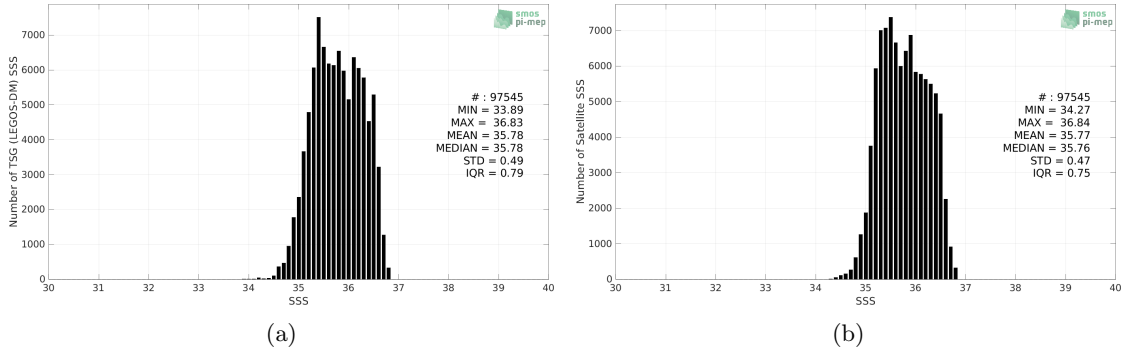
Figure 2: Histograms of SSS from TSG (LEGOS-DM) (a) and SMOS SSS L3 v8 - 18 Days (CATDS-CECOS-LOCEAN) (b) considering all match-up pairs per bins of 0.1 over the OTT zone Pi-MEP region and for the full satellite product period.
