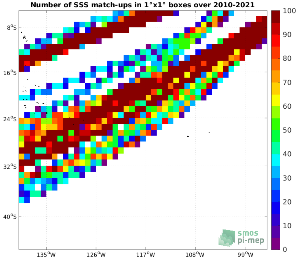
Figure 4: Number of SSS match-ups between TSG (LEGOS-DM) SSS and the SMOS SSS L3 v8 - 18 Days (CATDS-CECOS-LOCEAN) SSS product for the OTT zone Pi-MEP region over 1^\circ \times 1^\circ boxes and for the full satellite product period.
