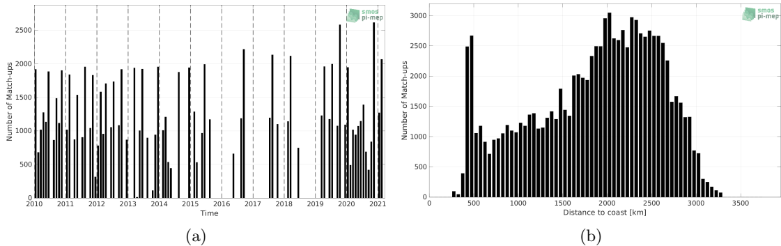
Figure 1: Number of match-ups between TSG (LEGOS-DM) and SMOS SSS L3 v8 - 18 Days (CATDS-CECOS-LOCEAN) SSS as a function of time (a) and as function of the distance to coast (b) over the OTT zone Pi-MEP region and for the full satellite product period.
