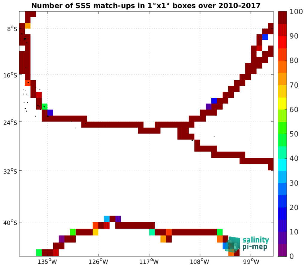
Figure 4: Number of SSS match-ups between TSG (GOSUD-Sailing-ship) SSS and the SMOS SSS L3 v8 - 18 Days (CATDS-CEC-LOCEAN) SSS product for the OTT zone Pi-MEP region over 1^\circ \times 1^\circ boxes and for the full satellite product period.
