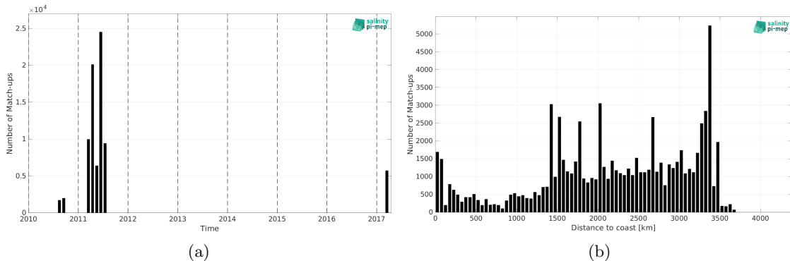
Figure 1: Number of match-ups between TSG (GOSUD-Sailing-ship) and SMOS SSS L3 v8 - 18 Days (CATDS-CEC-LOCEAN) SSS as a function of time (a) and as function of the distance to coast (b) over the OTT zone Pi-MEP region and for the full satellite product period.
