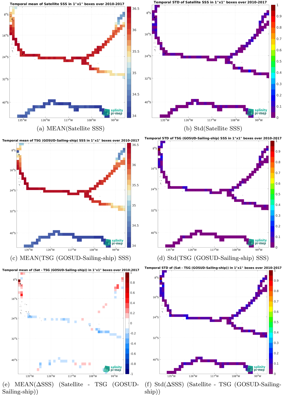
Figure 6: Temporal mean (left) and Std (right) of SSS from SMOS SSS L3 v8 - 18 Days (CATDS-CEC-LOCEAN) (top), TSG (GOSUD-Sailing-ship) (middle), and of \Delta SSS (Satellite - TSG (GOSUD-Sailing-ship)). Only match-up pairs are used to generate these maps.
