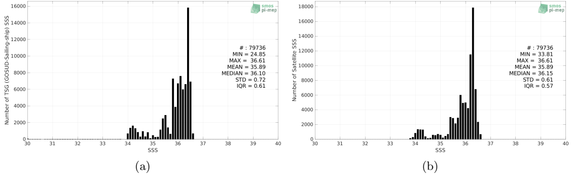
Figure 2: Histograms of SSS from TSG (GOSUD-Sailing-ship) (a) and SMOS SSS L3 v8 - 18 Days (CATDS-CECOS-LOCEAN) (b) considering all match-up pairs per bins of 0.1 over the OTT zone Pi-MEP region and for the full satellite product period.
