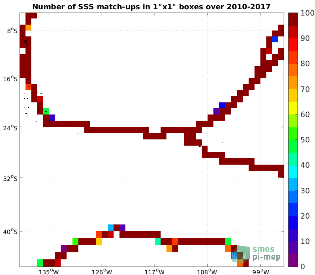
Figure 4: Number of SSS match-ups between TSG (GOSUD-Sailing-ship) SSS and the SMOS SSS L3 v8 - 18 Days (CATDS-CECOS-LOCEAN) SSS product for the OTT zone Pi-MEP region over 1^\circ \times 1^\circ boxes and for the full satellite product period.
