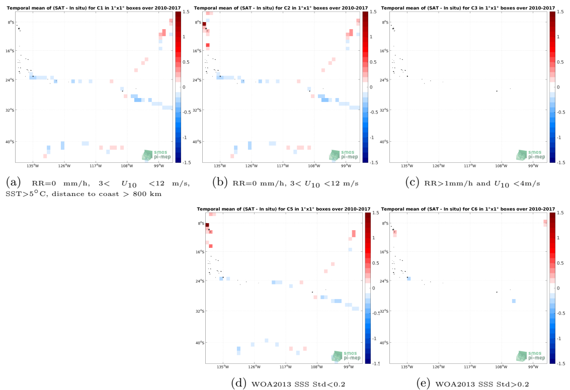
Figure 12: Temporal mean gridded over spatial boxes of size 1^\circ \times 1^\circ of \Delta SSS (SMOS SSS L3 v8 - 18 Days (CATDS-CECOS-LOCEAN) - TSG (GOSUD-Sailing-ship)) for 5 different subdatasets corresponding to:RR=0 mm/h, 3 < U_{10} < 12 m/s, SST >5^\circ C, distance to coast > 800 km (a), RR=0 mm/h, 3 < U_{10} < 12 m/s (b), RR >1 mm/h and U_{10} < 4 m/s (c), WOA2013 SSS Std <0.2 (d), WOA2013 SSS Std >0.2 (e).
