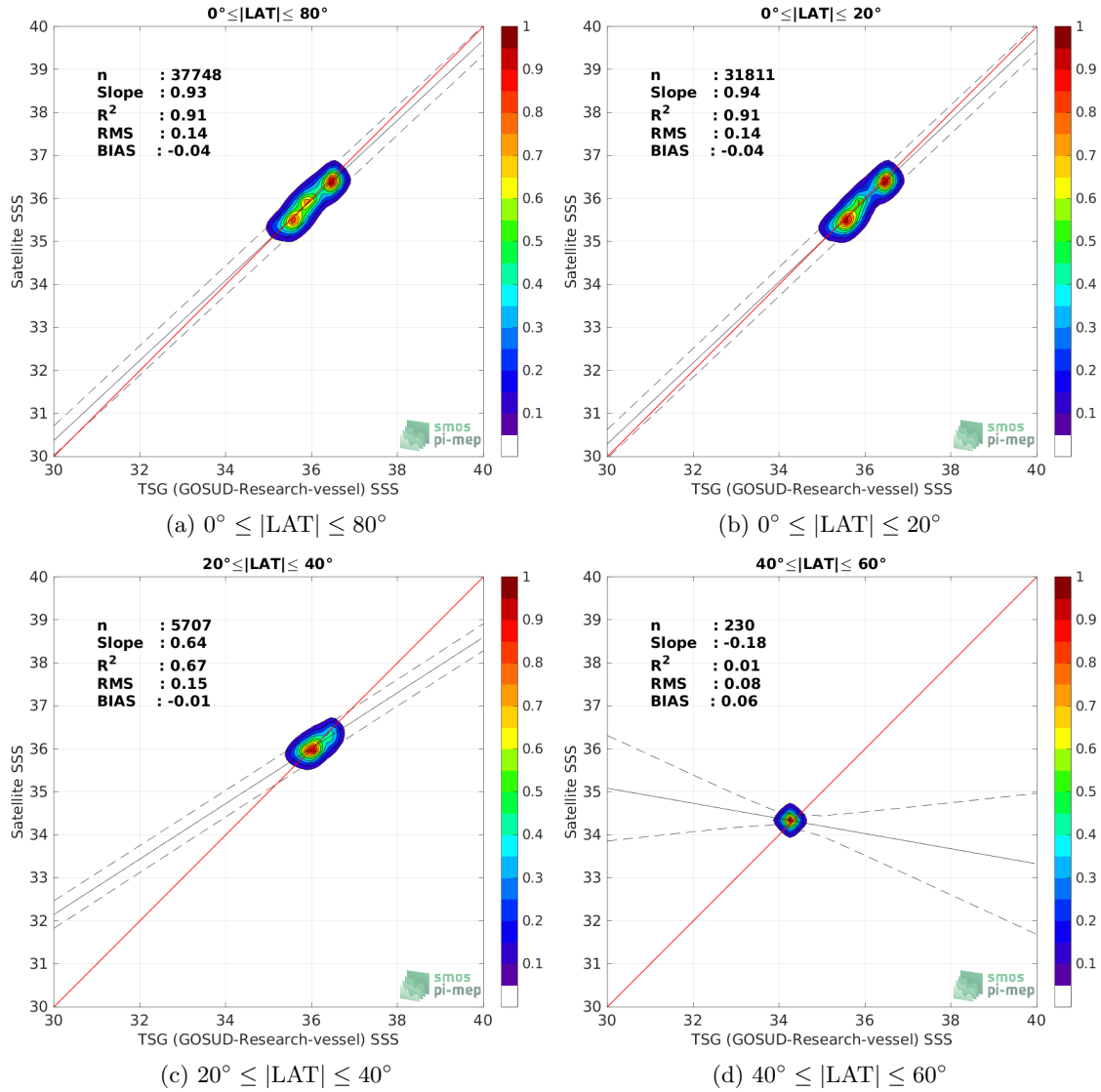
Figure 9: Contour maps of the concentration of SMOS SSS L3 v8 - 18 Days (CATDS-CECOS-LOCEAN) SSS ( y -axis) versus TSG (GOSUD-Research-vessel) SSS ( x -axis) at match-up pairs for different latitude bands. For each plot, the red line shows x=y . The black thin and dashed lines indicate a linear fit through the data cloud and the \pm 95\% confidence levels, respectively. The number match-up pairs n , the slope and R^2 coefficient of the linear fit, the root mean square (RMS) and the mean bias between satellite and in situ data are indicated for each latitude band in each plots.
