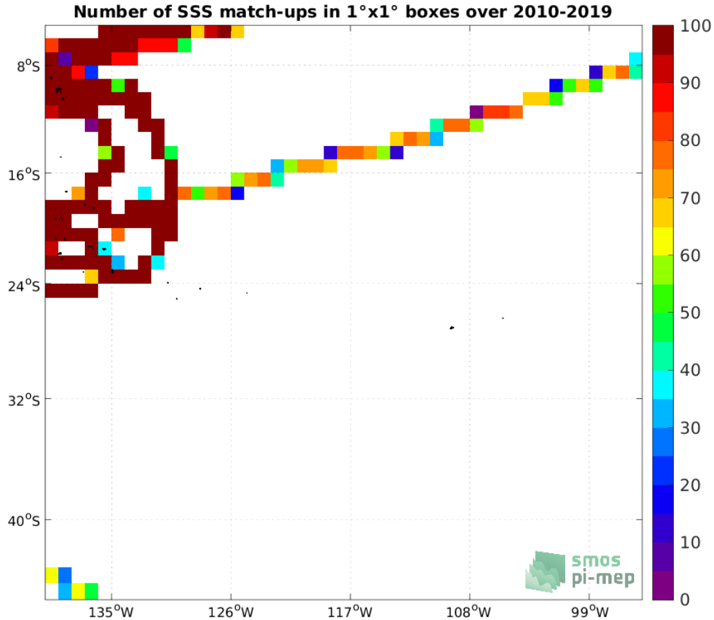
Figure 4: Number of SSS match-ups between TSG (GOSUD-Research-vessel) SSS and the SMOS SSS L3 v8 - 18 Days (CATDS-CECOS-LOCEAN) SSS product for the OTT zone Pi-MEP region over 1^\circ \times 1^\circ boxes and for the full satellite product period.
