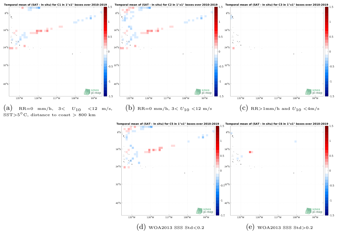
Figure 12: Temporal mean gridded over spatial boxes of size 1^\circ \times 1^\circ of \Delta SSS (SMOS SSS L3 v8 - 18 Days (CATDS-CECOS-LOCEAN) - TSG (GOSUD-Research-vessel)) for 5 different sub-datasets corresponding to:RR=0 mm/h, 3 < U_{10} < 12 m/s, SST>5°C, distance to coast > 800 km (a), RR=0 mm/h, 3 < U_{10} < 12 m/s (b), RR>1mm/h and U_{10} < 4 m/s (c), WOA2013 SSS Std<0.2 (d), WOA2013 SSS Std>0.2 (e).
