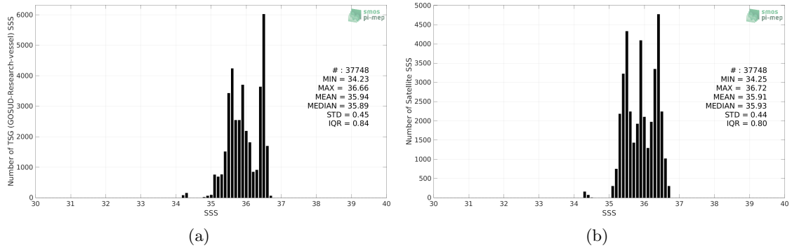
Figure 2: Histograms of SSS from TSG (GOSUD-Research-vessel) (a) and SMOS SSS L3 v8 - 18 Days (CATDS-CECOS-LOCEAN) (b) considering all match-up pairs per bins of 0.1 over the OTT zone Pi-MEP region and for the full satellite product period.
