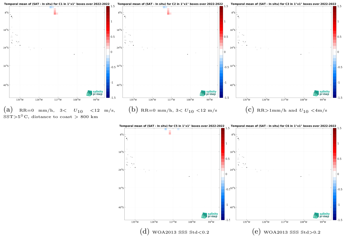
Figure 12: Temporal mean gridded over spatial boxes of size 1^\circ \times 1^\circ of \Delta SSS (SMOS SSS L3 v8 - 18 Days (CATDS-CEC-LOCEAN) - Sairdrone) for 5 different subdatasets corresponding to:RR=0 mm/h, 3 < U_{10} < 12 m/s, SST >5^\circ C, distance to coast > 800 km (a), RR=0 mm/h, 3 < U_{10} < 12 m/s (b), RR >1 mm/h and U_{10} < 4 m/s (c), WOA2013 SSS Std <0.2 (d), WOA2013 SSS Std >0.2 (e).
