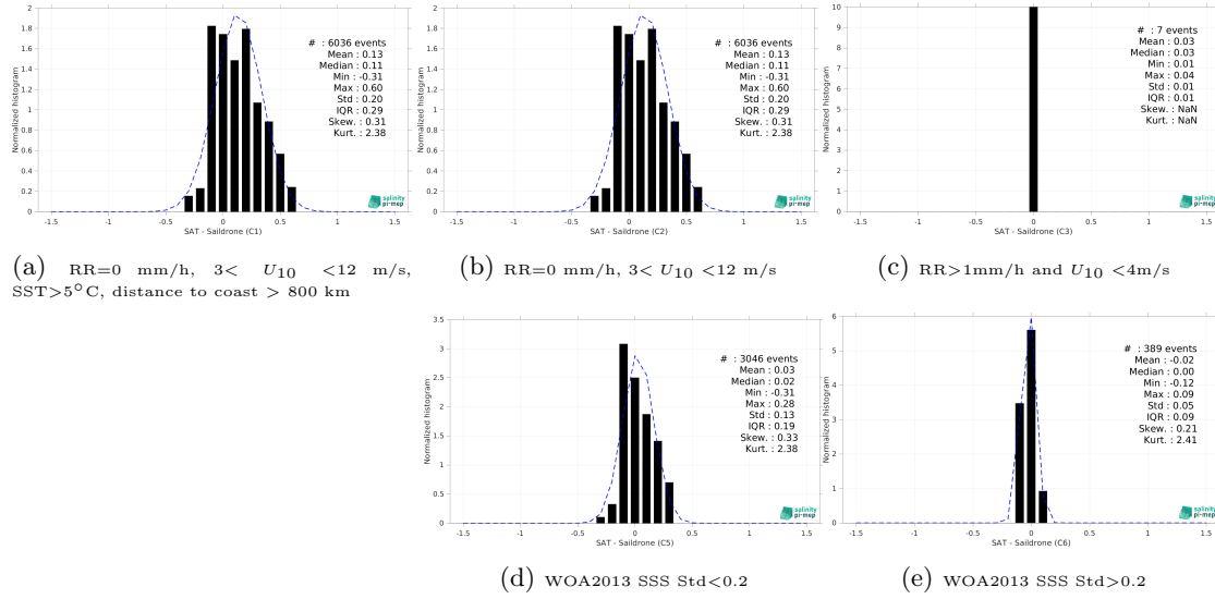
Figure 13: Normalized histogram of \Delta SSS (SMOS SSS L3 v8 - 18 Days (CATDS-CEC-LOCEAN) - Sairdronne) for 5 different subdatasets corresponding to: RR=0 mm/h, 3 < U_{10} < 12 m/s, SST > 5°C, distance to coast > 800 km (a), RR=0 mm/h, 3 < U_{10} < 12 m/s (b), RR > 1mm/h and U_{10} < 4 m/s (c), WOA2013 SSS Std < 0.2 (d), WOA2013 SSS Std > 0.2 (e).
