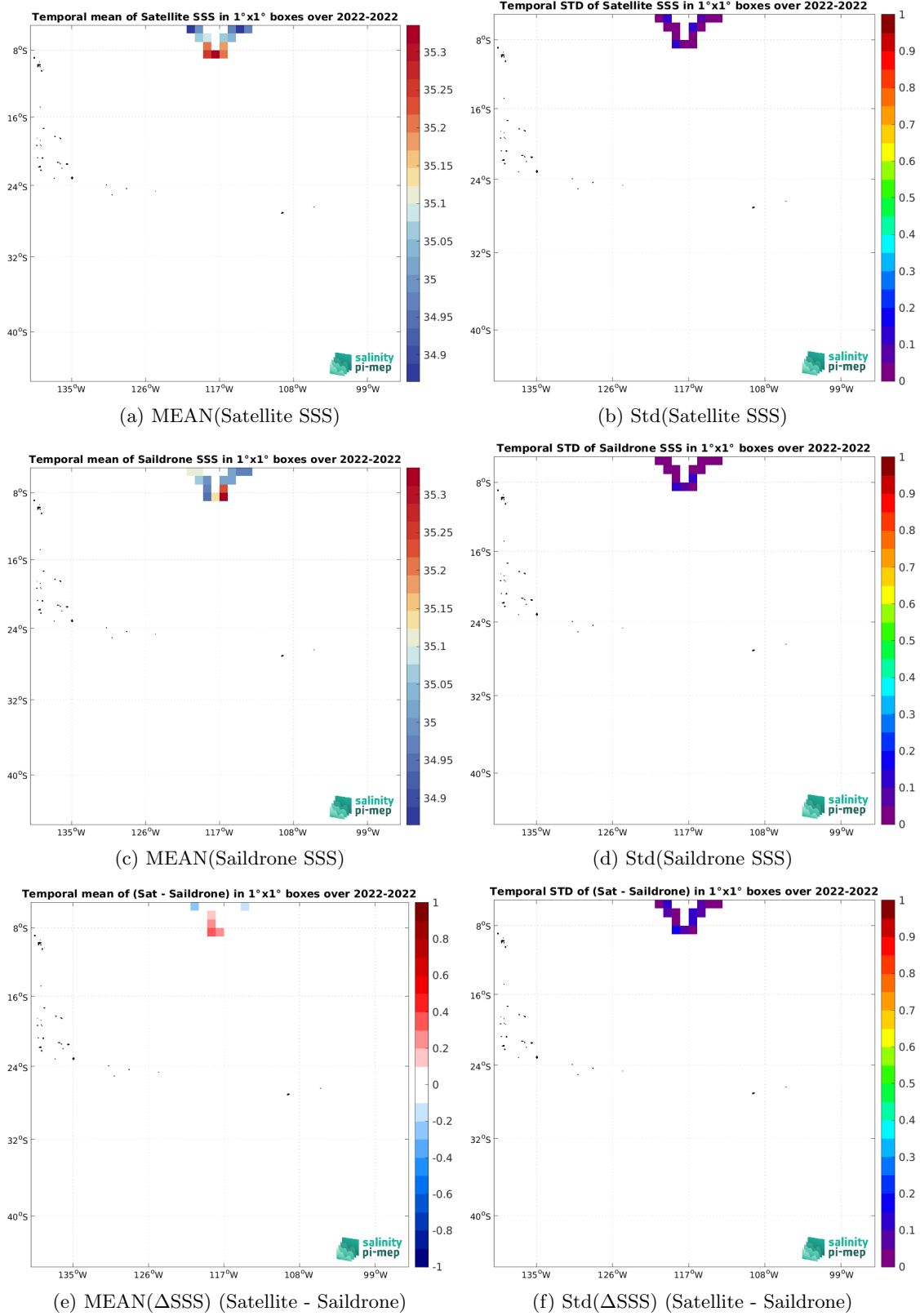
Figure 6: Temporal mean (left) and Std (right) of SSS from SMOS SSS L3 v8 - 18 Days (CATDS-CEC-LOCEAN) (top), Saildrone (middle), and of \Delta SSS (Satellite - Saildrone). Only match-up pairs are used to generate these maps.
