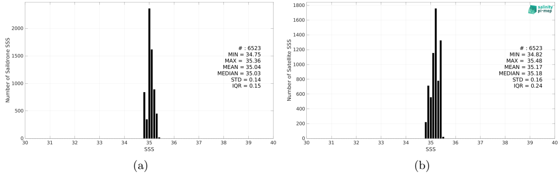
Figure 2: Histograms of SSS from Saildrone (a) and SMOS SSS L3 v8 - 18 Days (CATDS-CEC-LOCEAN) (b) considering all match-up pairs per bins of 0.1 over the OTT zone Pi-MEP region and for the full satellite product period.
