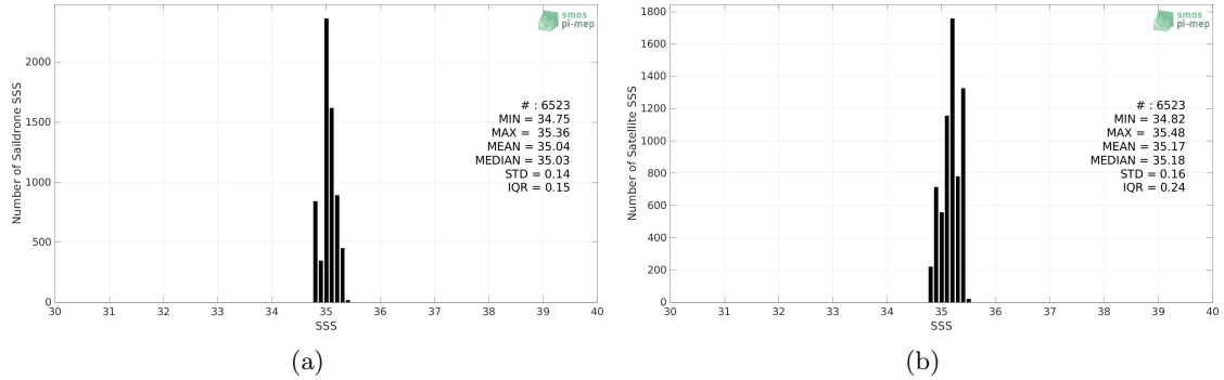
Figure 2: Histograms of SSS from Saildrone (a) and SMOS SSS L3 v8 - 18 Days (CATDS-CECOS-LOCEAN) (b) considering all match-up pairs per bins of 0.1 over the OTT zone Pi-MEP region and for the full satellite product period.
