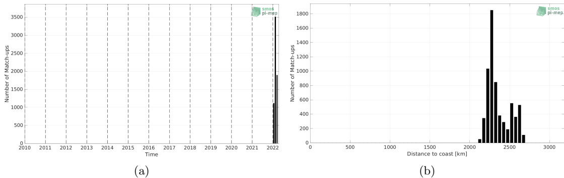
Figure 1: Number of match-ups between Saildrone and SMOS SSS L3 v8 - 18 Days (CATDS-CECOS-LOCEAN) SSS as a function of time (a) and as function of the distance to coast (b) over the OTT zone Pi-MEP region and for the full satellite product period.
