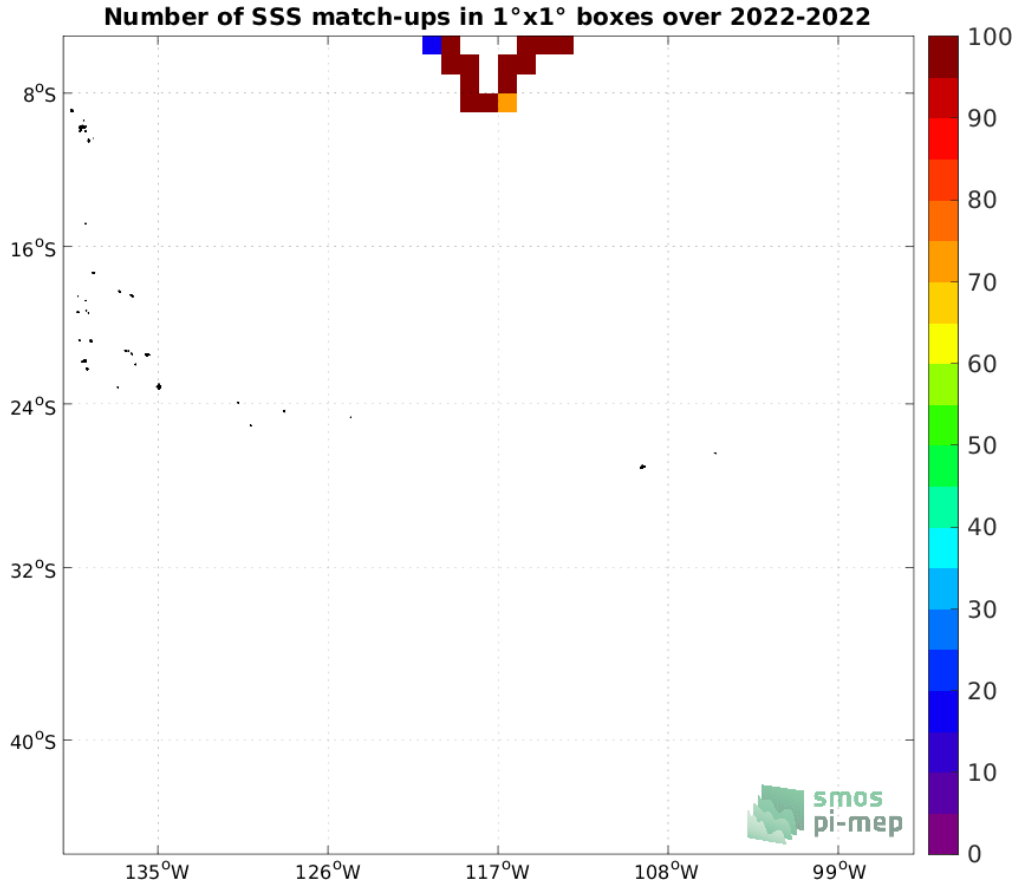
Figure 4: Number of SSS match-ups between Saildrone SSS and the SMOS SSS L3 v8 - 18 Days (CATDS-CECOS-LOCEAN) SSS product for the OTT zone Pi-MEP region over 1^\circ \times 1^\circ boxes and for the full satellite product period.
