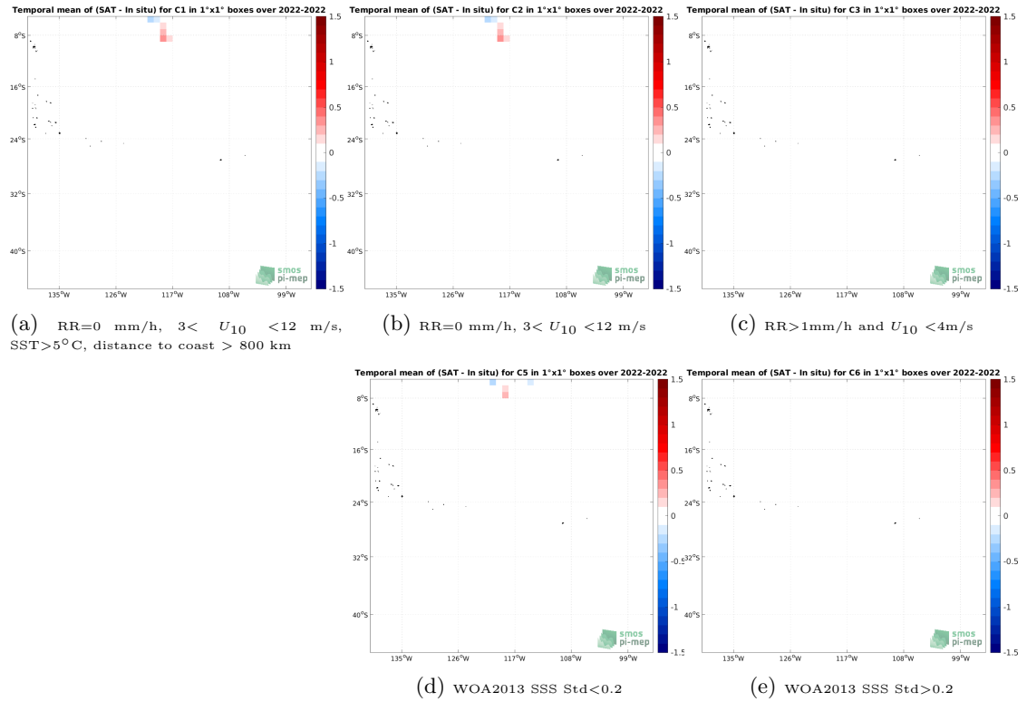
Figure 12: Temporal mean gridded over spatial boxes of size 1^\circ \times 1^\circ of \Delta SSS (SMOS SSS L3 v8 - 18 Days (CATDS-CECOS-LOCEAN) - Sairdrone) for 5 different subdatasets corresponding to:RR=0 mm/h, 3 < U_{10} < 12 m/s, SST >5^\circ C, distance to coast > 800 km (a), RR=0 mm/h, 3 < U_{10} < 12 m/s (b), RR >1 mm/h and U_{10} < 4 m/s (c), WOA2013 SSS Std <0.2 (d), WOA2013 SSS Std >0.2 (e).
