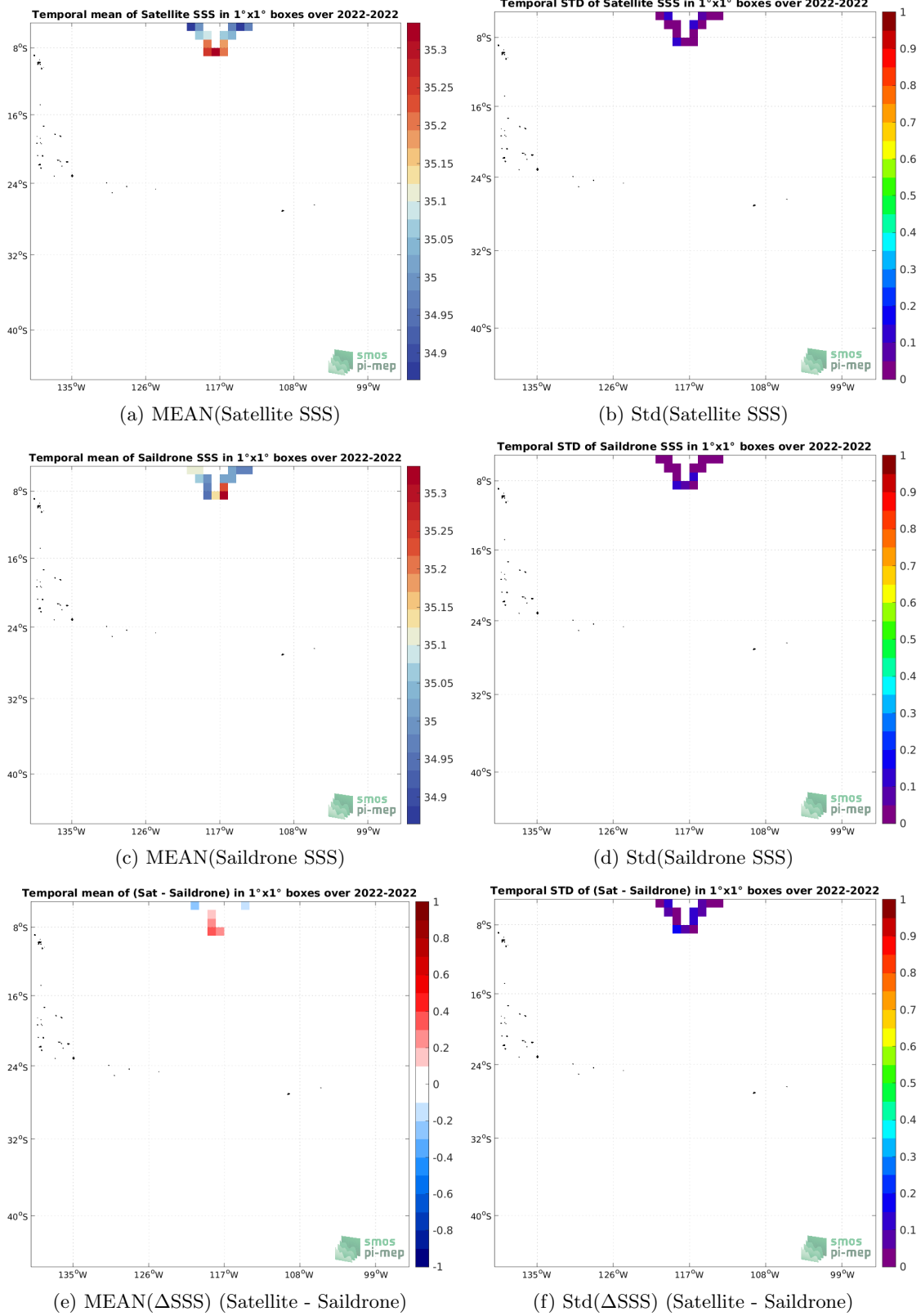
Figure 6: Temporal mean (left) and Std (right) of SSS from SMOS SSS L3 v8 - 18 Days (CATDS-CECOS-LOCEAN) (top), Saildrone (middle), and of \Delta SSS (Satellite - Saildrone). Only match-pairs are used to generate these maps.
