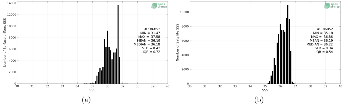
Figure 2: Histograms of SSS from Surface drifters (a) and SMOS SSS L3 v8 - 18 Days (CATDS-CECOS-LOCEAN) (b) considering all match-up pairs per bins of 0.1 over the OTT zone Pi-MEP region and for the full satellite product period.
