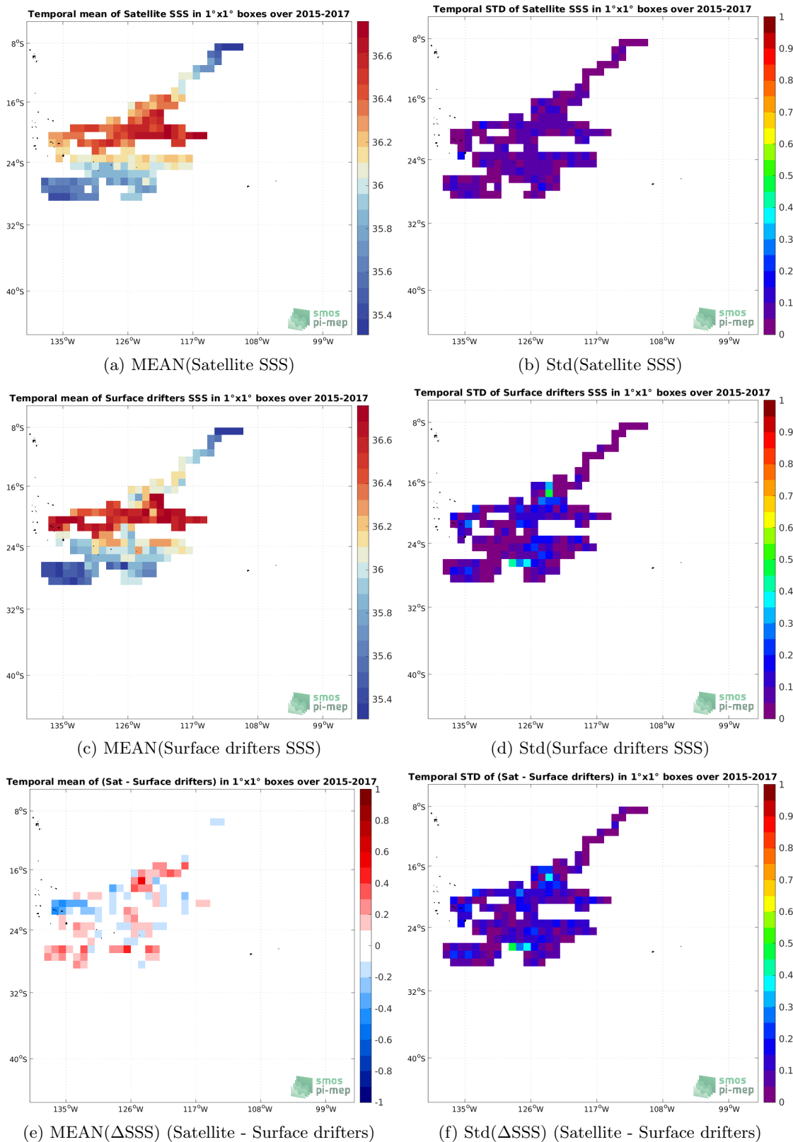
Figure 5: Temporal mean (left) and Std (right) of SSS from SMOS SSS L3 v8 - 18 Days (CATDS-CECOS-LOCEAN) (top), Surface drifters (middle), and of \Delta SSS (Satellite - Surface drifters). Only match-up pairs are used to generate these maps.
