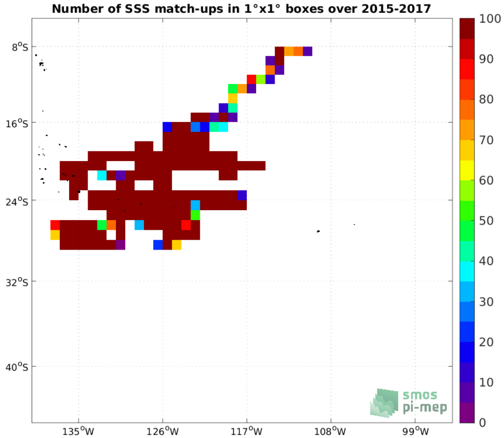
Figure 3: Number of SSS match-ups between Surface drifters SSS and the SMOS SSS L3 v8 - 18 Days (CATDS-CECOS-LOCEAN) SSS product for the OTT zone Pi-MEP region over 1°x1° boxes and for the full satellite product period.
