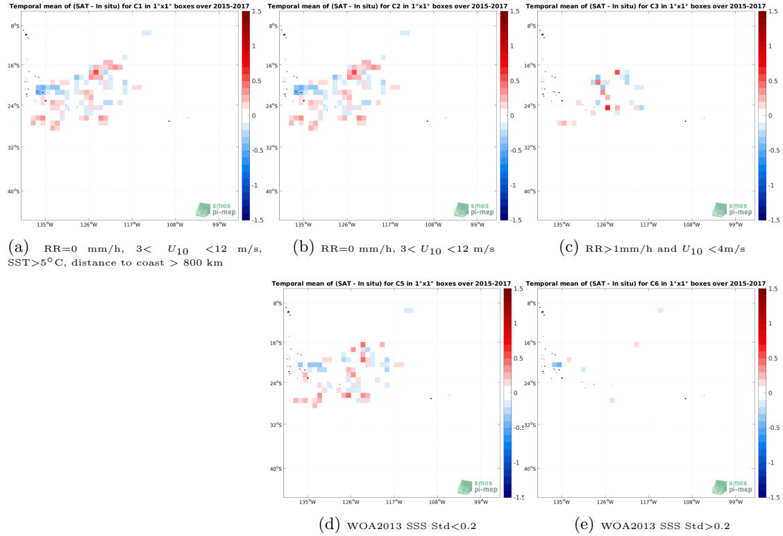
Figure 11: Temporal mean gridded over spatial boxes of size 1^{\circ}\times 1^{\circ} of \Delta\text{SSS} (SMOS SSS L3 v8 - 18 Days (CATDS-CECOS-LOCEAN) - Surface drifters) for 5 different subdatasets corresponding to:RR=0 mm/h, 3 < U_{10} < 12 m/s, SST >5^{\circ}\text{C} , distance to coast > 800 km (a), RR=0 mm/h, 3 < U_{10} < 12 m/s (b), RR >1 mm/h and U_{10} < 4 m/s (c), WOA2013 SSS Std <0.2 (d), WOA2013 SSS Std >0.2 (e).
