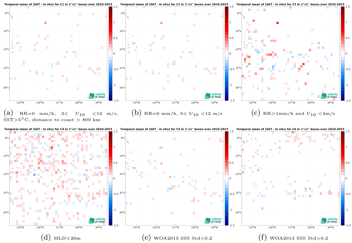
Figure 12: Temporal mean gridded over spatial boxes of size 1^\circ \times 1^\circ of \Delta SSS (SMOS SSS L3 v8 - 18 Days (CATDS-CEC-LOCEAN) - Argo) for 6 different subdatasets corresponding to:RR=0 mm/h, 3 < U_{10} < 12 m/s, SST >5^\circ C, distance to coast > 800 km (a), RR=0 mm/h, 3 < U_{10} < 12 m/s (b), RR >1 mm/h and U_{10} < 4 m/s (c),MLD <20 m (d),WOA2013 SSS Std <0.2 (e),WOA2013 SSS Std >0.2 (f).
