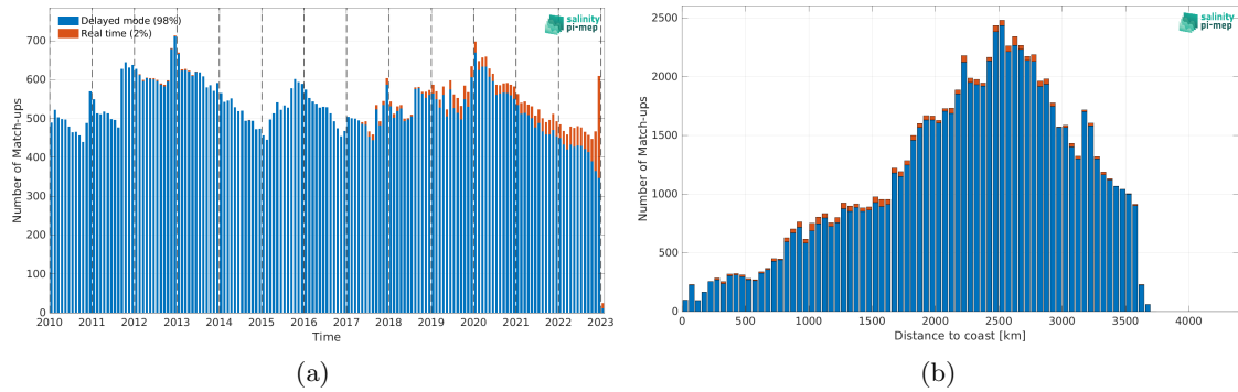
Figure 1: Number of match-ups between Argo and SMOS SSS L3 v8 - 18 Days (CATDS-CEC-LOCEAN) SSS as a function of time (a) and as function of the distance to coast (b) over the OTT zone Pi-MEP region and for the full satellite product period.
