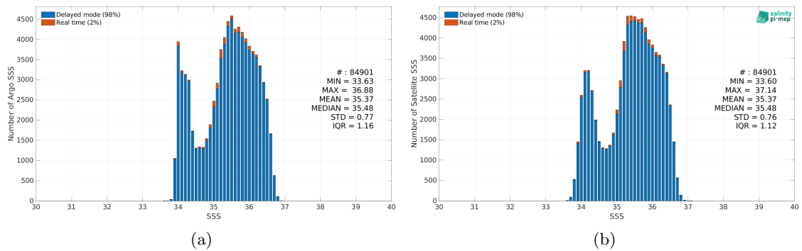
Figure 2: Histograms of SSS from Argo (a) and SMOS SSS L3 v8 - 18 Days (CATDS-CEC-LOCEAN) (b) considering all match-up pairs per bins of 0.1 over the OTT zone Pi-MEP region and for the full satellite product period.
