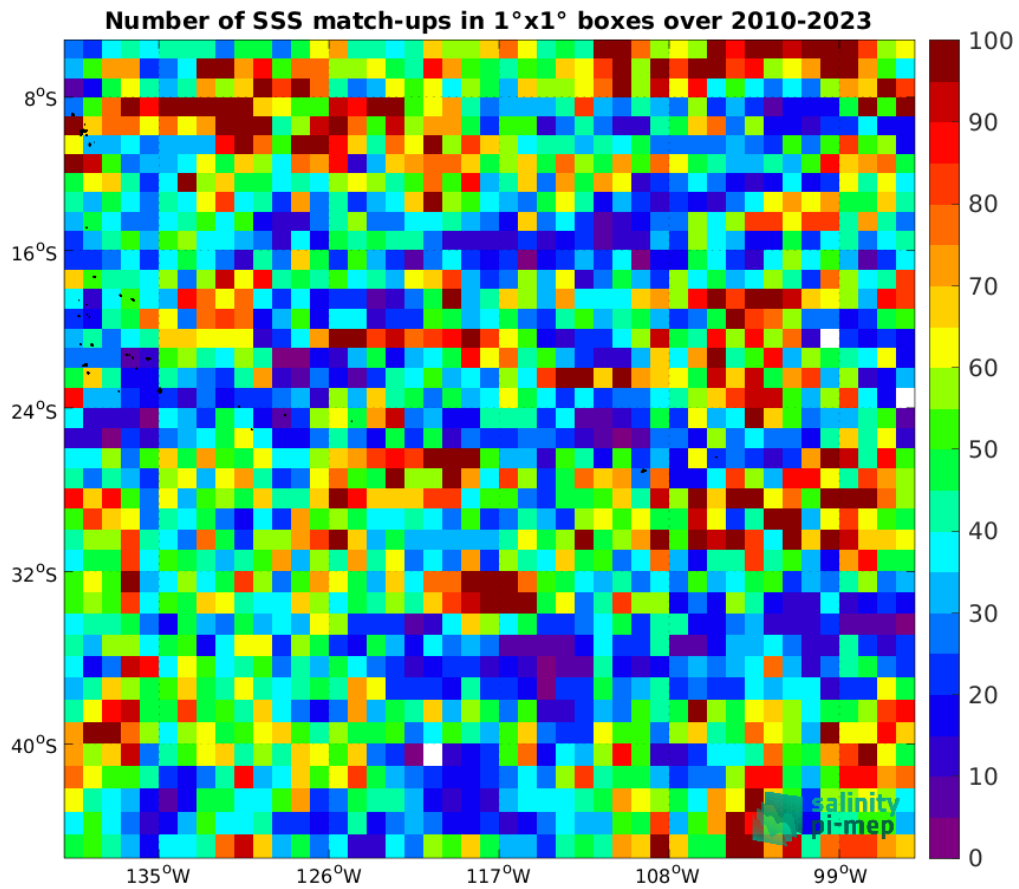
Figure 4: Number of SSS match-ups between Argo SSS and the SMOS SSS L3 v8 - 18 Days (CATDS-CEC-LOCEAN) SSS product for the OTT zone Pi-MEP region over 1°x1° boxes and for the full satellite product period.
