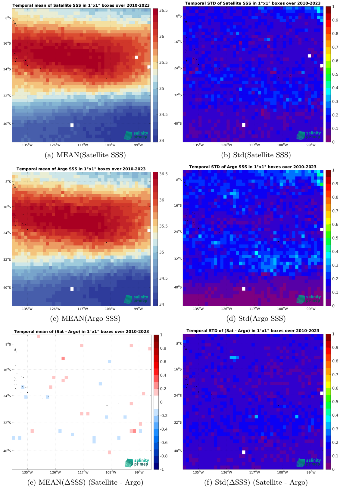
Figure 6: Temporal mean (left) and Std (right) of SSS from SMOS SSS L3 v8 - 18 Days (CATDS-CEC-LOCEAN) (top), Argo (middle), and of \Delta SSS (Satellite - Argo). Only match-up pairs are used to generate these maps.
