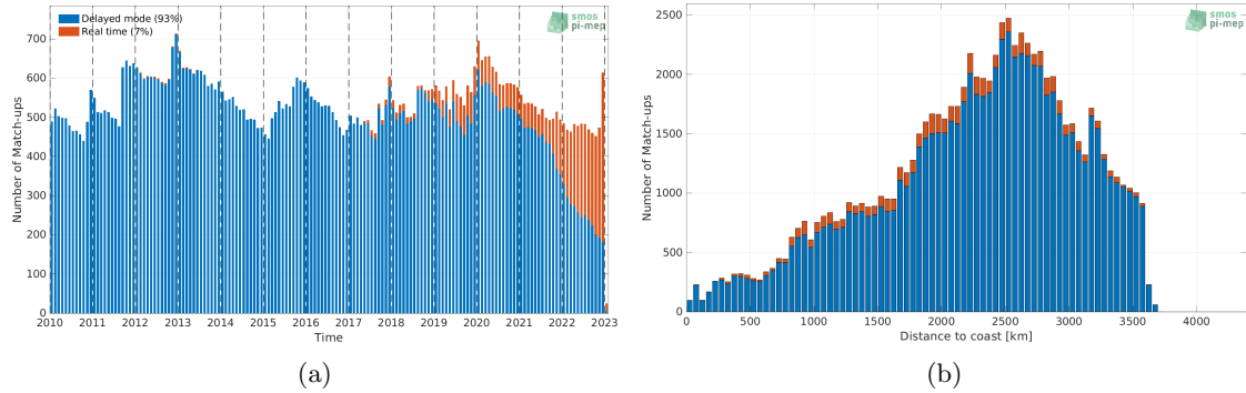
Figure 1: Number of match-ups between Argo and SMOS SSS L3 v8 - 18 Days (CATDS-CECOS-LOCEAN) SSS as a function of time (a) and as function of the distance to coast (b) over the OTT zone Pi-MEP region and for the full satellite product period.
