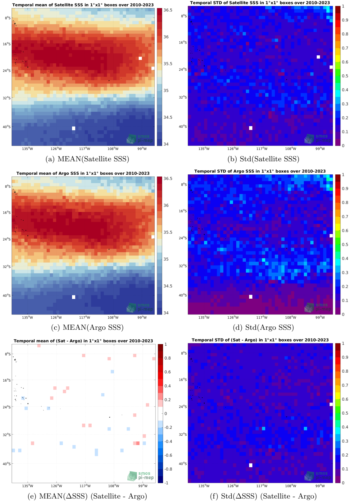
Figure 6: Temporal mean (left) and Std (right) of SSS from SMOS SSS L3 v8 - 18 Days (CATDS-CECOS-LOCEAN) (top), Argo (middle), and of \Delta SSS (Satellite - Argo). Only match-up pairs are used to generate these maps.
