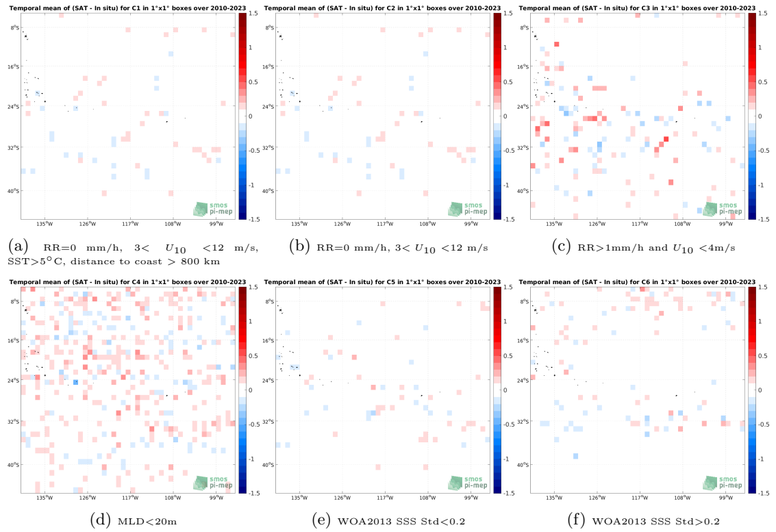
Figure 12: Temporal mean gridded over spatial boxes of size 1^\circ \times 1^\circ of \Delta SSS (SMOS SSS L3 v8 - 18 Days (CATDS-CECOS-LOCEAN) - Argo) for 6 different subdatasets corresponding to:RR=0 mm/h, 3 < U_{10} < 12 m/s, SST >5^\circ C, distance to coast > 800 km (a), RR=0 mm/h, 3 < U_{10} < 12 m/s (b), RR >1 mm/h and U_{10} < 4 m/s (c),MLD <20 m (d),WOA2013 SSS Std <0.2 (e),WOA2013 SSS Std >0.2 (f).
