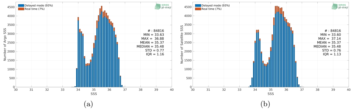
Figure 2: Histograms of SSS from Argo (a) and SMOS SSS L3 v8 - 18 Days (CATDS-CECOS-LOCEAN) (b) considering all match-up pairs per bins of 0.1 over the OTT zone Pi-MEP region and for the full satellite product period.
