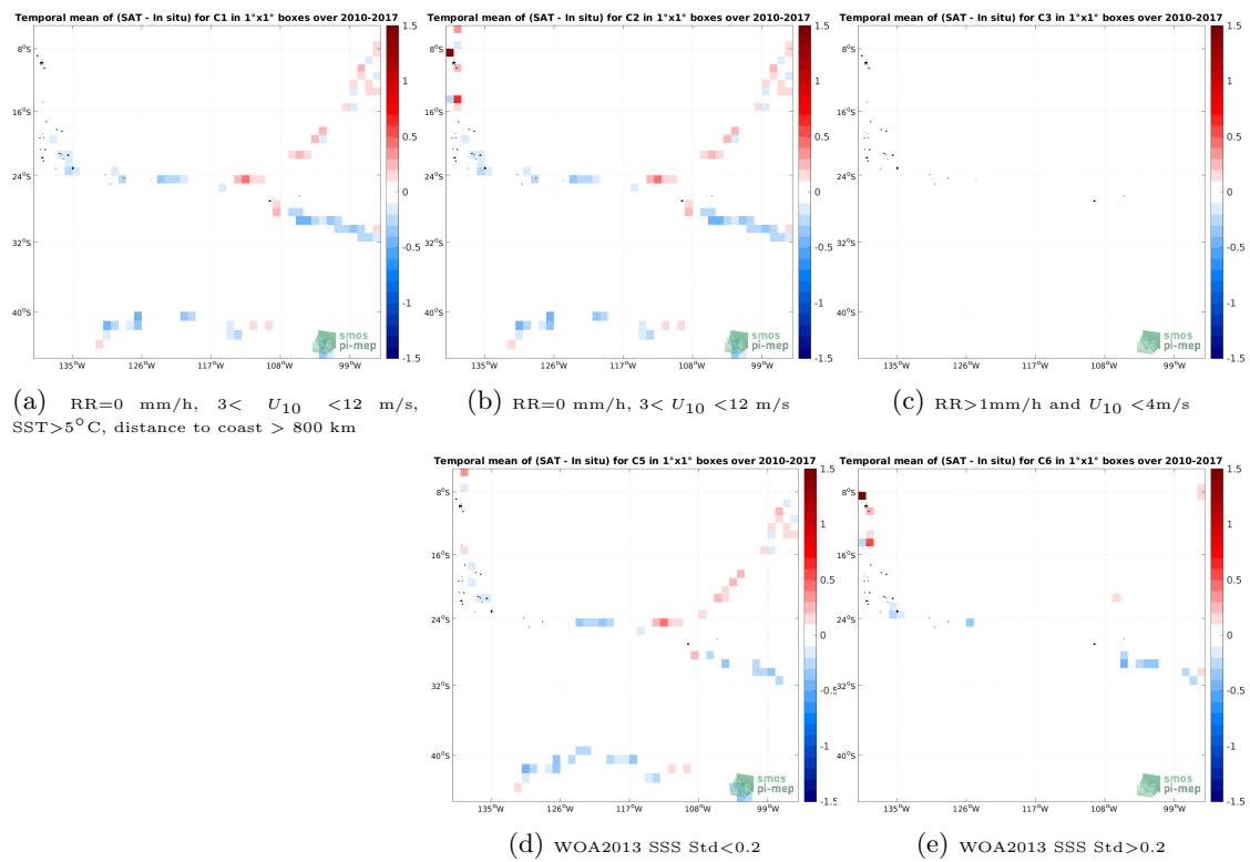
Figure 12: Temporal mean gridded over spatial boxes of size 1^\circ \times 1^\circ of \Delta SSS (SMOS SSS L3 v7 - 9 Days (CATDS-CECOS-LOCEAN) - TSG (GOSUD-Sailing-ship)) for 5 different subdatasets corresponding to:RR=0 mm/h, 3 < U_{10} < 12 m/s, SST > 5^\circ C , distance to coast > 800 km (a), RR=0 mm/h, 3 < U_{10} < 12 m/s (b), RR > 1 mm/h and U_{10} < 4 m/s (c), WOA2013 SSS Std < 0.2 (d), WOA2013 SSS Std > 0.2 (e).
