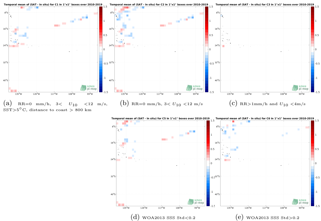
Figure 12: Temporal mean gridded over spatial boxes of size 1^\circ \times 1^\circ of \Delta\text{SSS} (SMOS SSS L3 v7 - 9 Days (CATDS-CECOS-LOCEAN) - TSG (GOSUD-Research-vessel)) for 5 different subdatasets corresponding to:RR=0 mm/h, 3 < U_{10} < 12 m/s, \text{SST} > 5^\circ\text{C} , distance to coast > 800 km (a), RR=0 mm/h, 3 < U_{10} < 12 m/s (b), RR >1 mm/h and U_{10} < 4 m/s (c), WOA2013 SSS Std <0.2 (d), WOA2013 SSS Std >0.2 (e).
