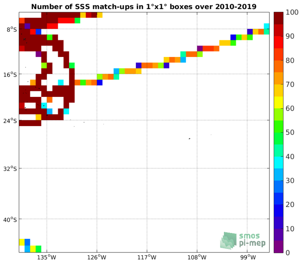
Figure 4: Number of SSS match-ups between TSG (GOSUD-Research-vessel) SSS and the SMOS SSS L3 v7 - 9 Days (CATDS-CECOS-LOCEAN) SSS product for the OTT zone Pi-MEP region over 1^\circ \times 1^\circ boxes and for the full satellite product period.
