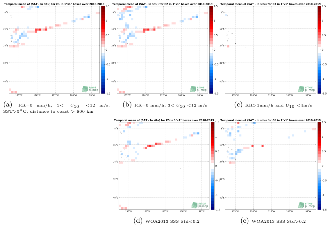
Figure 12: Temporal mean gridded over spatial boxes of size 1^\circ \times 1^\circ of \Delta\text{SSS} (SMOS SSS L3 v7 - 9 Days (CATDS-CECOS-LOCEAN) - TSG (GOSUD-Research-vessel)) for 5 different subdatasets corresponding to: \text{RR}=0 \text{ mm/h} , 3 < U_{10} < 12 \text{ m/s} , \text{SST} > 5^\circ\text{C} , distance to coast > 800 \text{ km} (a), \text{RR}=0 \text{ mm/h} , 3 < U_{10} < 12 \text{ m/s} (b), \text{RR} > 1 \text{ mm/h} and U_{10} < 4 \text{ m/s} (c), WOA2013 SSS Std < 0.2 (d), WOA2013 SSS Std > 0.2 (e).
