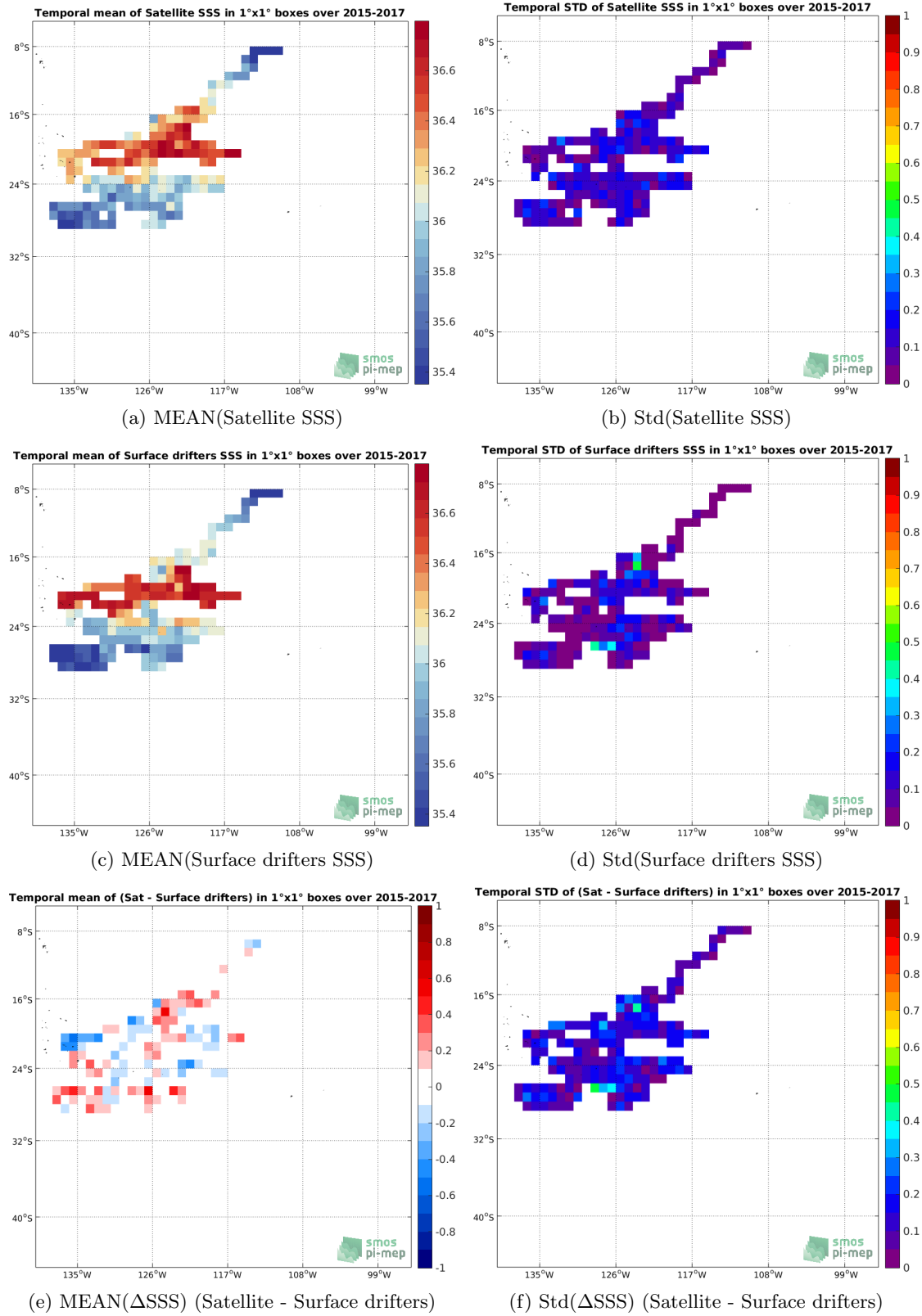
Figure 5: Temporal mean (left) and Std (right) of SSS from SMOS SSS L3 v7 - 9 Days (CATDS-CECOS-LOCEAN) (top), Surface drifters (middle), and of \Delta SSS (Satellite - Surface drifters). Only match-up pairs are used to generate these maps.
