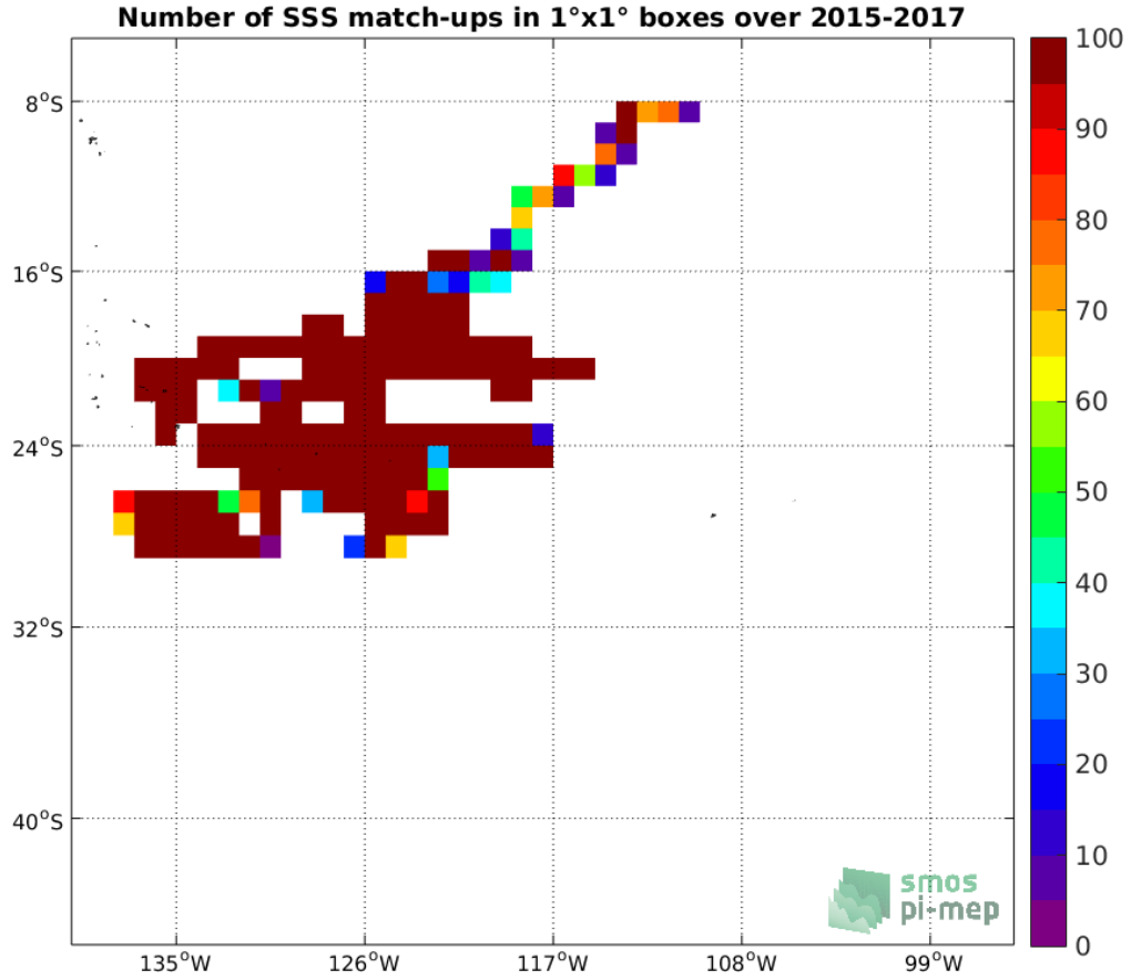
Figure 3: Number of SSS match-ups between Surface drifters SSS and the SMOS SSS L3 v7 - 9 Days (CATDS-CECOS-LOCEAN) SSS product for the OTT zone Pi-MEP region over 1^\circ \times 1^\circ boxes and for the full satellite product period.
