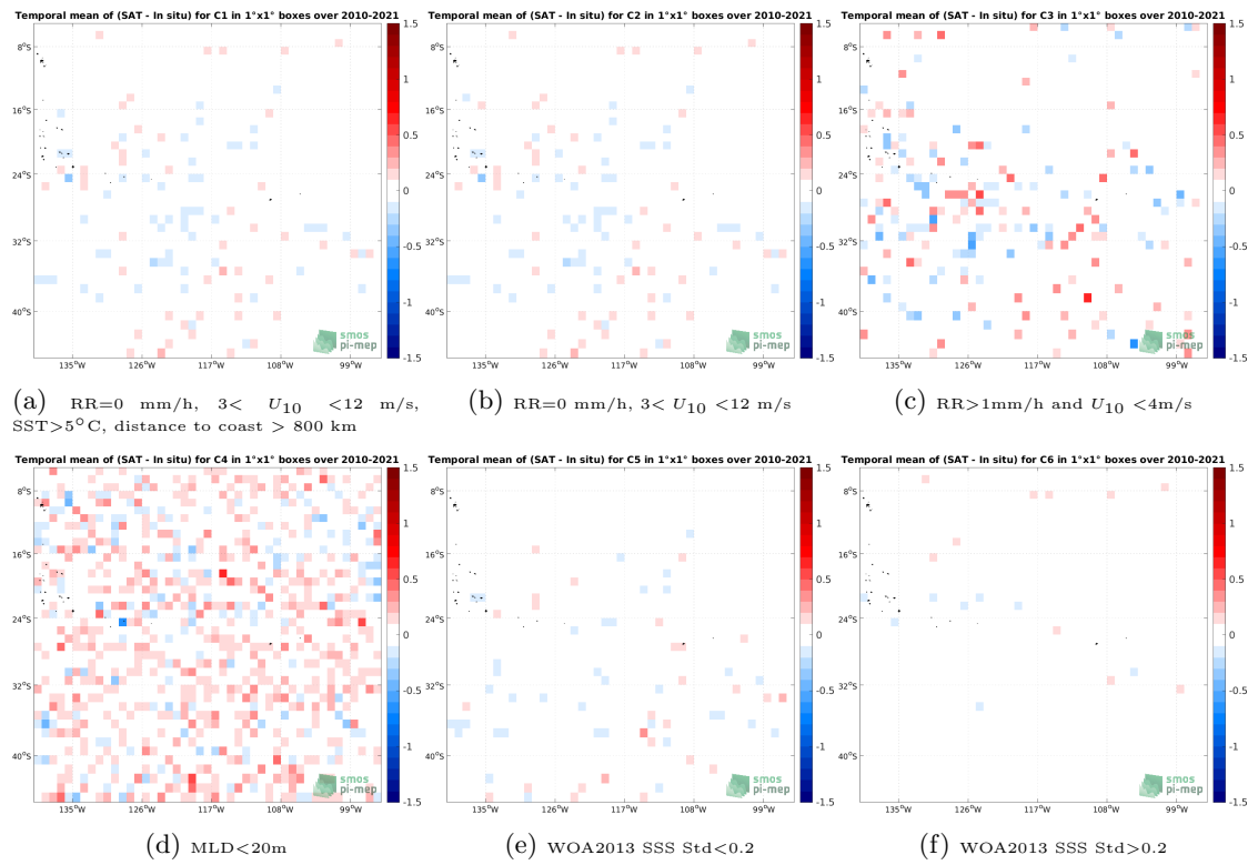
Figure 12: Temporal mean gridded over spatial boxes of size 1^\circ \times 1^\circ of \Delta SSS (SMOS SSS L3 v7 - 9 Days (CATDS-CECOS-LOCEAN) - Argo) for 6 different subdatasets corresponding to:RR=0 mm/h, 3 < U_{10} < 12 m/s, SST >5^\circ C, distance to coast > 800 km (a), RR=0 mm/h, 3 < U_{10} < 12 m/s (b), RR >1 mm/h and U_{10} < 4 m/s (c),MLD <20 m (d),WOA2013 SSS Std <0.2 (e),WOA2013 SSS Std >0.2 (f).
