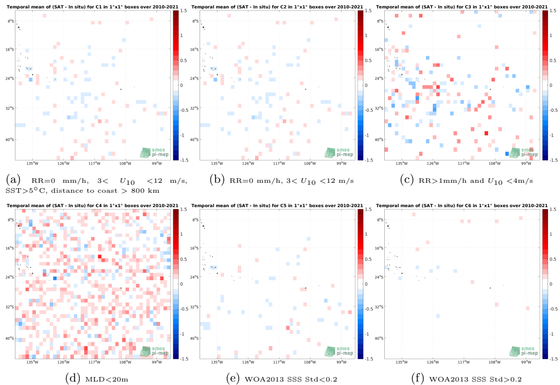
Figure 12: Temporal mean gridded over spatial boxes of size 1^\circ \times 1^\circ of \Delta SSS (SMOS SSS L3 v7 - 9 Days (CATDS-CECOS-LOCEAN) - Argo) for 6 different subdatasets corresponding to:RR=0 mm/h, 3 < U_{10} < 12 m/s, SST >5^\circ C, distance to coast > 800 km (a), RR=0 mm/h, 3 < U_{10} < 12 m/s (b), RR >1 mm/h and U_{10} < 4 m/s (c),MLD <20 m (d),WOA2013 SSS Std <0.2 (e),WOA2013 SSS Std >0.2 (f).
