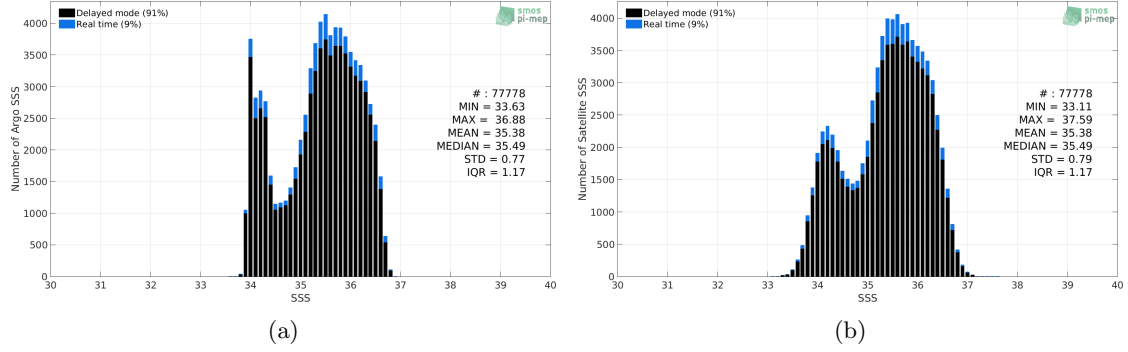
Figure 2: Histograms of SSS from Argo (a) and SMOS SSS L3 v7 - 9 Days (CATDS-CECOS-LOCEAN) (b) considering all match-up pairs per bins of 0.1 over the OTT zone Pi-MEP region and for the full satellite product period.
