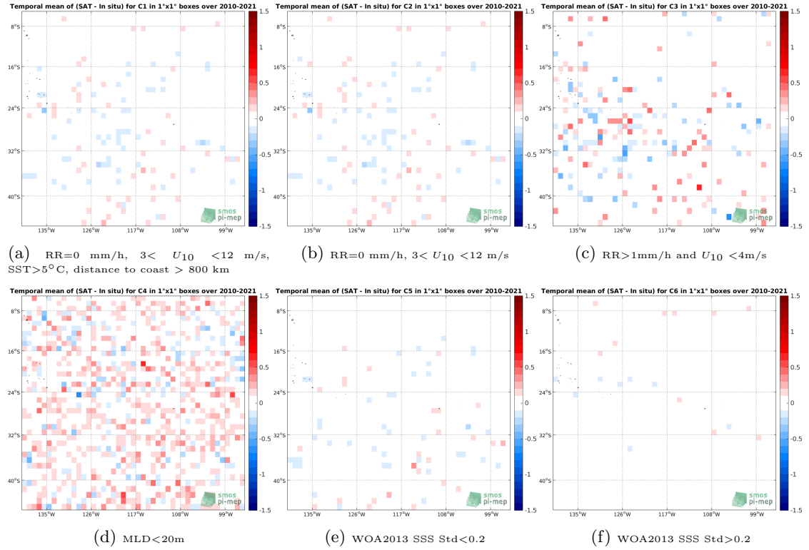
Figure 12: Temporal mean gridded over spatial boxes of size 1^\circ \times 1^\circ of \Delta SSS (SMOS SSS L3 v7 - 9 Days (CATDS-CECOS-LOCEAN) - Argo) for 6 different subdatasets corresponding to: RR=0 mm/h, 3 < U_{10} < 12 m/s, SST > 5^\circ C , distance to coast > 800 km (a), RR=0 mm/h, 3 < U_{10} < 12 m/s (b), RR > 1 mm/h and U_{10} < 4 m/s (c), MLD < 20 m (d), WOA2013 SSS Std < 0.2 (e), WOA2013 SSS Std > 0.2 (f).
