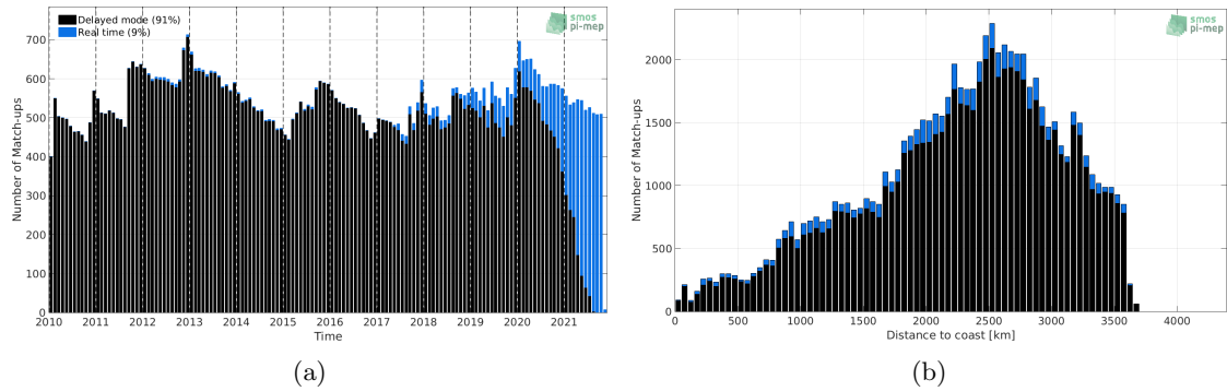
Figure 1: Number of match-ups between Argo and SMOS SSS L3 v7 - 9 Days (CATDS-CECOS-LOCEAN) SSS as a function of time (a) and as function of the distance to coast (b) over the OTT zone Pi-MEP region and for the full satellite product period.
