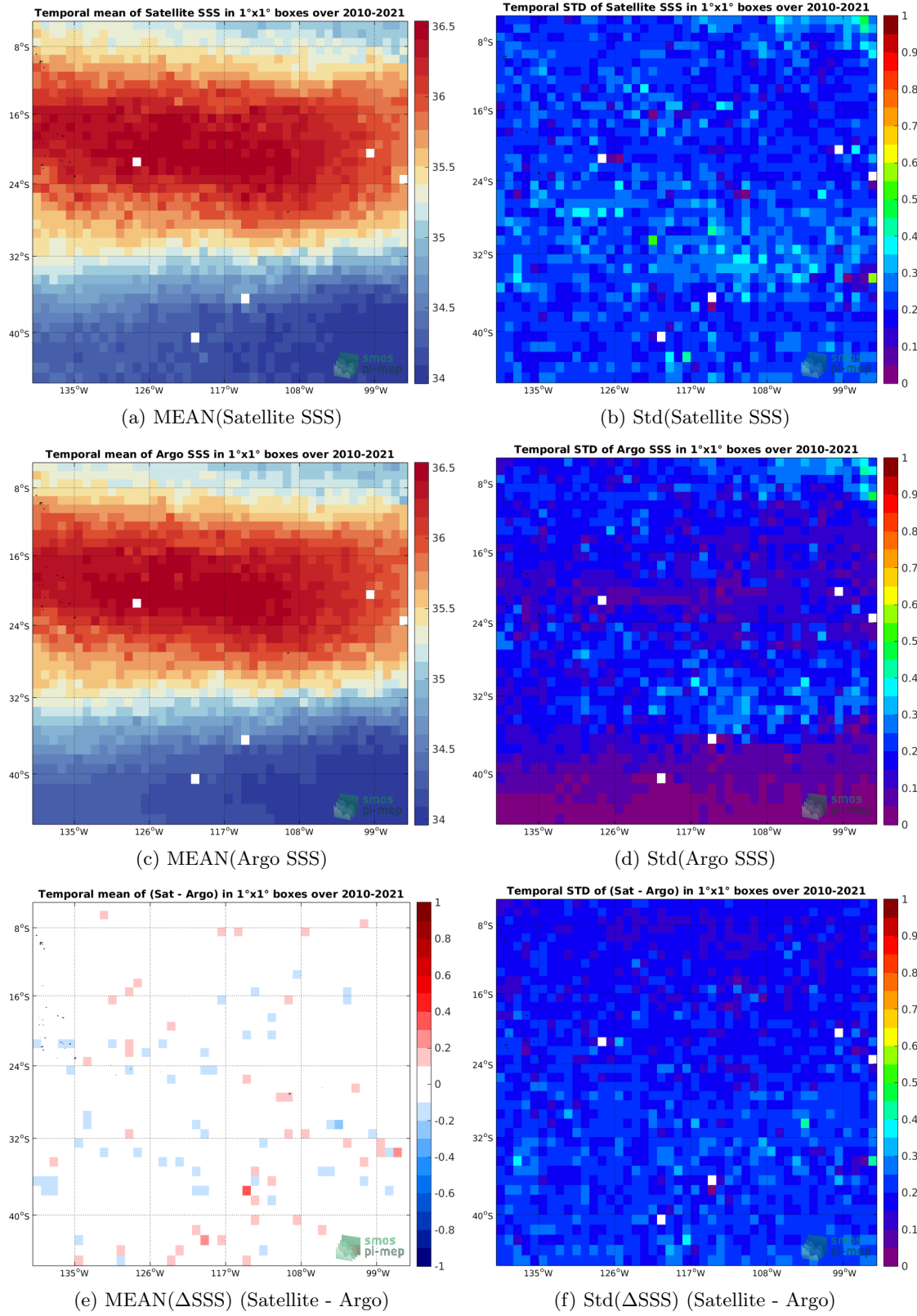
Figure 6: Temporal mean (left) and Std (right) of SSS from SMOS SSS L3 v7 - 9 Days (CATDS-CECOS-LOCEAN) (top), Argo (middle), and of \Delta SSS (Satellite - Argo). Only match-up pairs are used to generate these maps.
