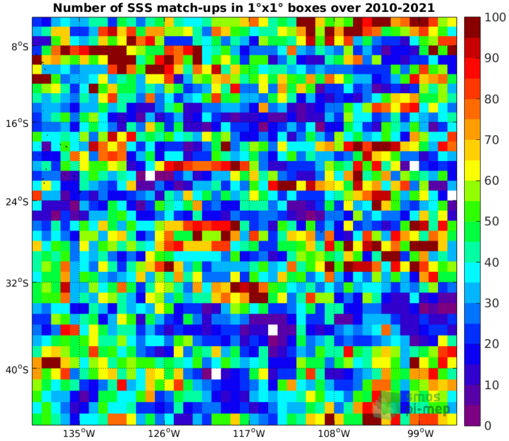
Figure 4: Number of SSS match-ups between Argo SSS and the SMOS SSS L3 v7 - 9 Days (CATDS-CECOS-LOCEAN) SSS product for the OTT zone Pi-MEP region over 1°x1° boxes and for the full satellite product period.
