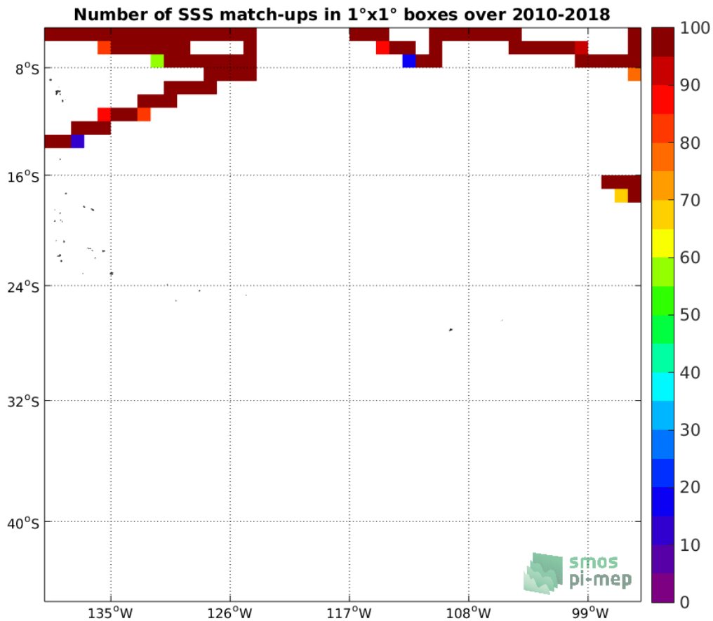
Figure 4: Number of SSS match-ups between TSG (SAMOS) SSS and the SMOS SSS L3 v7 - 18 Days (CATDS-CECOS-LOCEAN) SSS product for the OTT zone Pi-MEP region over 1^\circ \times 1^\circ boxes and for the full satellite product period.
