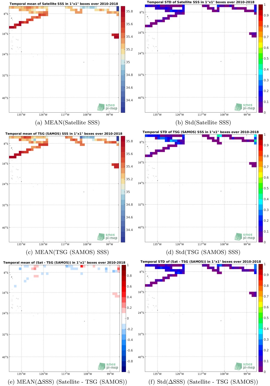
Figure 6: Temporal mean (left) and Std (right) of SSS from SMOS SSS L3 v7 - 18 Days (CATDS-CECOS-LOCEAN) (top), TSG (SAMOS) (middle), and of \Delta SSS (Satellite - TSG (SAMOS)). Only match-up pairs are used to generate these maps.
