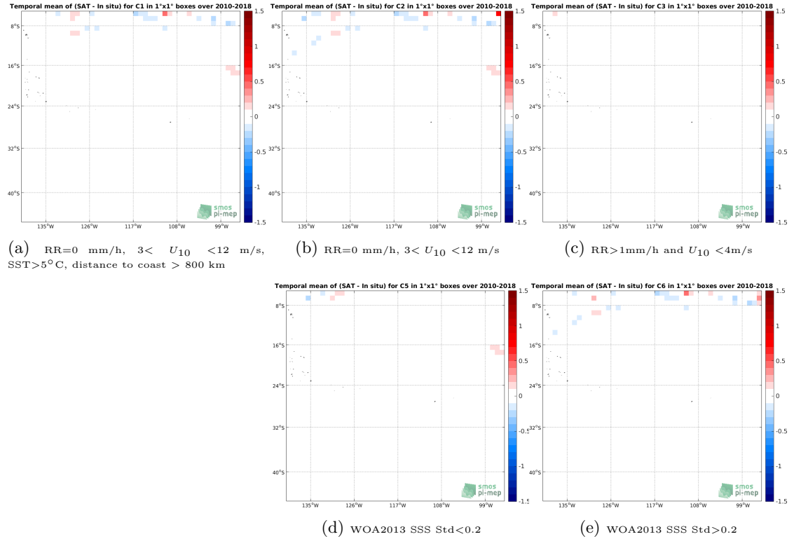
Figure 12: Temporal mean gridded over spatial boxes of size 1^{\circ}\times 1^{\circ} of \Delta\text{SSS} (SMOS SSS L3 v7 - 18 Days (CATDS-CECOS-LOCEAN) - TSG (SAMOS)) for 5 different subdatasets corresponding to:RR=0 mm/h, 3 < U_{10} < 12 m/s, SST >5^{\circ}\text{C} , distance to coast > 800 km (a), RR=0 mm/h, 3 < U_{10} < 12 m/s (b), RR >1 mm/h and U_{10} < 4 m/s (c), WOA2013 SSS Std <0.2 (d), WOA2013 SSS Std >0.2 (e).
