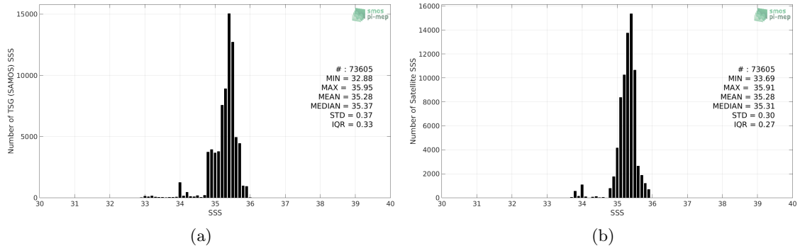
Figure 2: Histograms of SSS from TSG (SAMOS) (a) and SMOS SSS L3 v7 - 18 Days (CATDS-CECOS-LOCEAN) (b) considering all match-up pairs per bins of 0.1 over the OTT zone Pi-MEP region and for the full satellite product period.
