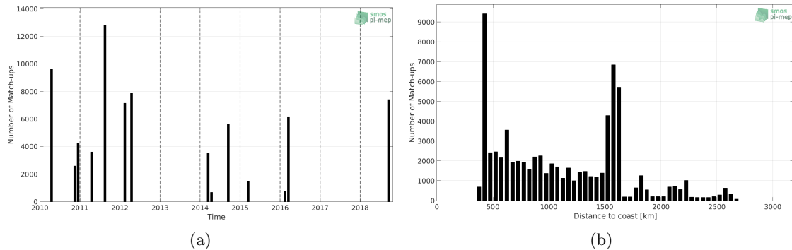
Figure 1: Number of match-ups between TSG (SAMOS) and SMOS SSS L3 v7 - 18 Days (CATDS-CECOS-LOCEAN) SSS as a function of time (a) and as function of the distance to coast (b) over the OTT zone Pi-MEP region and for the full satellite product period.
