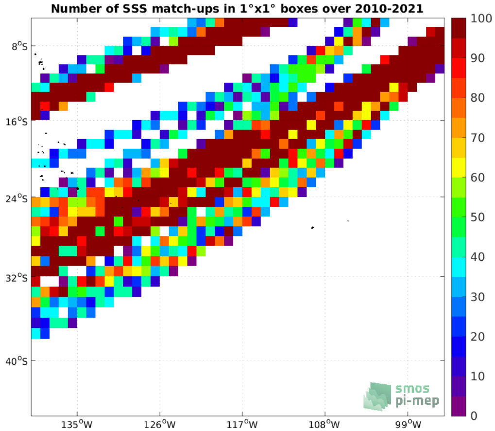
Figure 4: Number of SSS match-ups between TSG (LEGOS-DM) SSS and the SMOS SSS L3 v7 - 18 Days (CATDS-CECOS-LOCEAN) SSS product for the OTT zone Pi-MEP region over 1°x1° boxes and for the full satellite product period.
