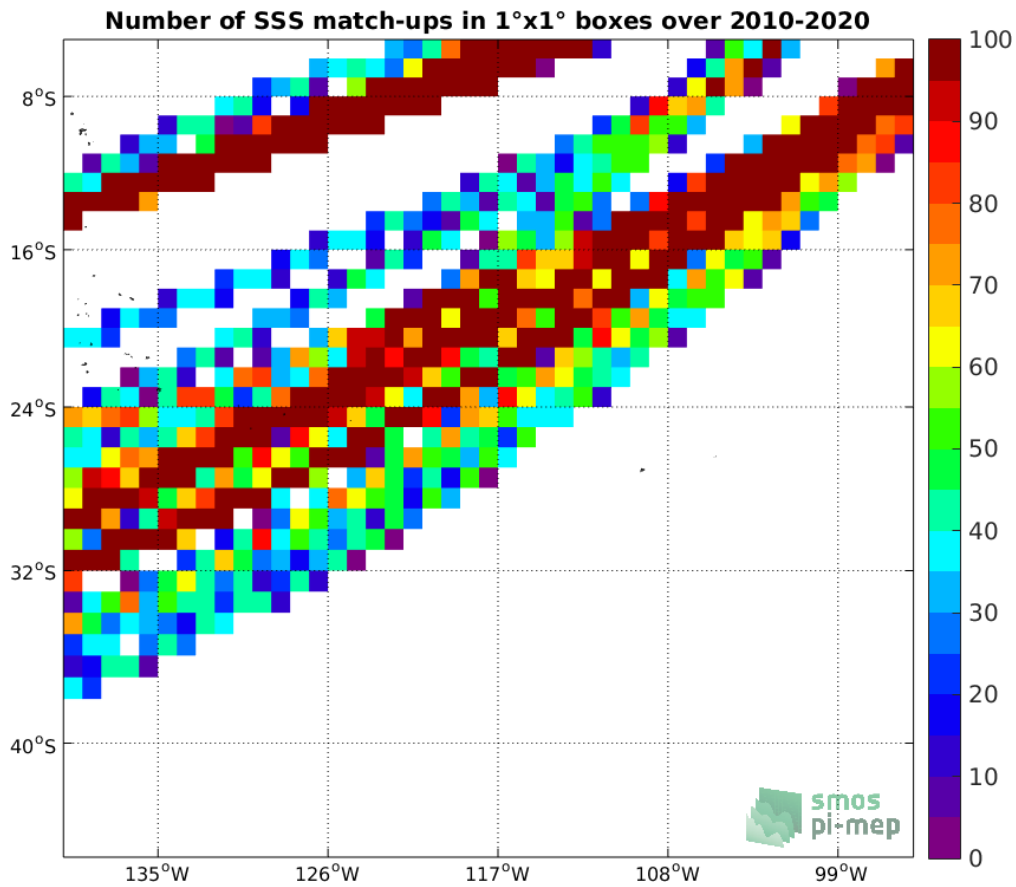
Figure 4: Number of SSS match-ups between TSG (LEGOS-DM) SSS and the SMOS SSS L3 v7 - 18 Days (CATDS-CECOS-LOCEAN) SSS product for the OTT zone Pi-MEP region over 1^\circ \times 1^\circ boxes and for the full satellite product period.
