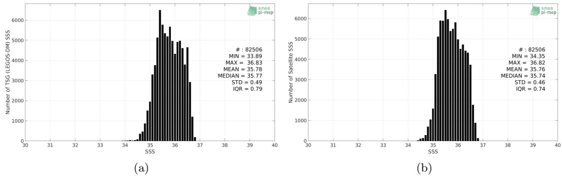
Figure 2: Histograms of SSS from TSG (LEGOS-DM) (a) and SMOS SSS L3 v7 - 18 Days (CATDS-CECOS-LOCEAN) (b) considering all match-up pairs per bins of 0.1 over the OTT zone Pi-MEP region and for the full satellite product period.
