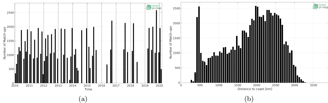
Figure 1: Number of match-ups between TSG (LEGOS-DM) and SMOS SSS L3 v7 - 18 Days (CATDS-CECOS-LOCEAN) SSS as a function of time (a) and as function of the distance to coast (b) over the OTT zone Pi-MEP region and for the full satellite product period.
