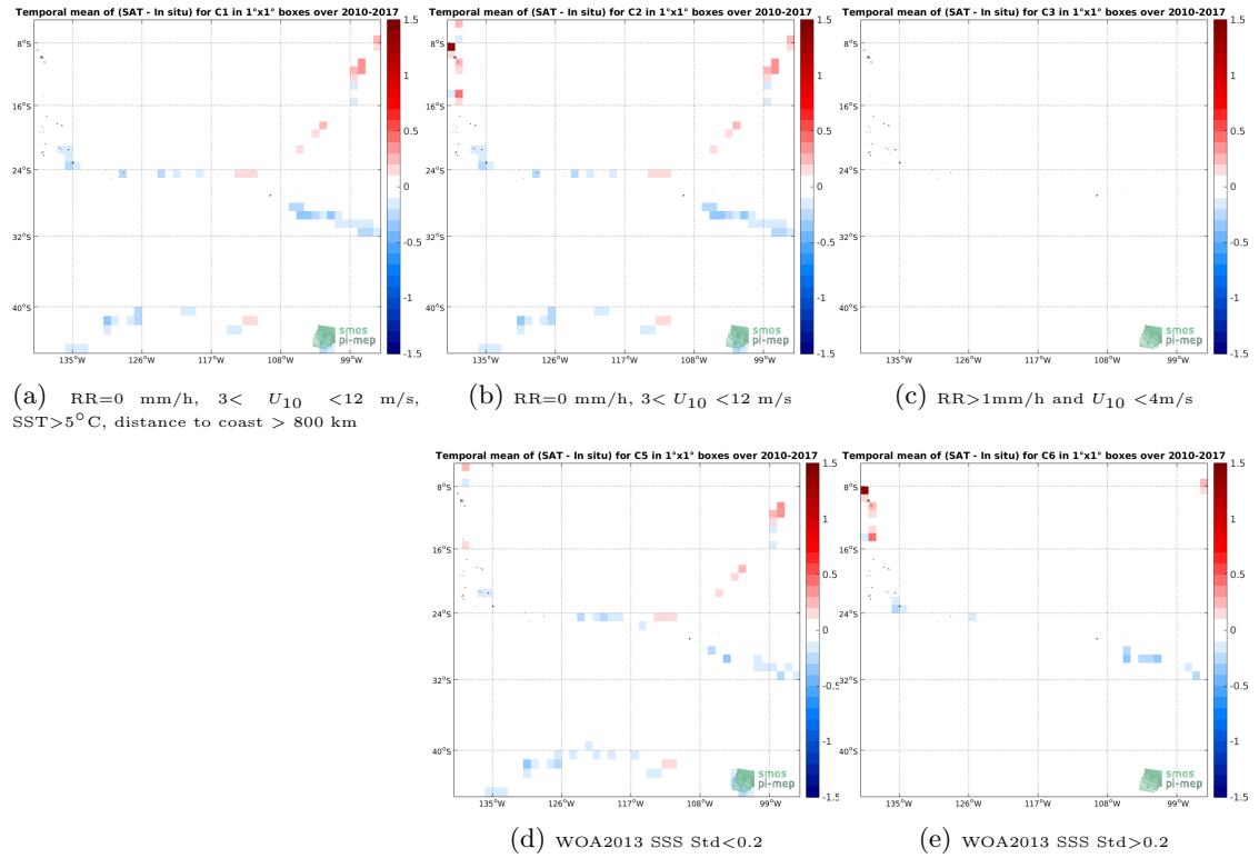
Figure 12: Temporal mean gridded over spatial boxes of size 1^\circ \times 1^\circ of \Delta\text{SSS} (SMOS SSS L3 v7 - 18 Days (CATDS-CECOS-LOCEAN) - TSG (GOSUD-Sailing-ship)) for 5 different subdatasets corresponding to: \text{RR}=0 \text{ mm/h} , 3 < U_{10} < 12 \text{ m/s} , \text{SST} > 5^\circ\text{C} , distance to coast > 800 \text{ km} (a), \text{RR}=0 \text{ mm/h} , 3 < U_{10} < 12 \text{ m/s} (b), \text{RR} > 1\text{mm/h} and U_{10} < 4\text{m/s} (c), WOA2013 SSS Std < 0.2 (d), WOA2013 SSS Std > 0.2 (e).
