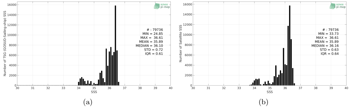
Figure 2: Histograms of SSS from TSG (GOSUD-Sailing-ship) (a) and SMOS SSS L3 v7 - 18 Days (CATDS-CECOS-LOCEAN) (b) considering all match-up pairs per bins of 0.1 over the OTT zone Pi-MEP region and for the full satellite product period.
