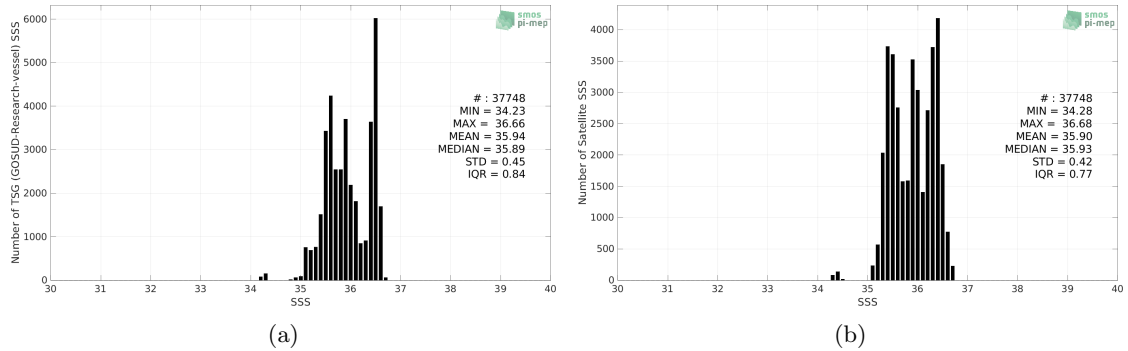
Figure 2: Histograms of SSS from TSG (GOSUD-Research-vessel) (a) and SMOS SSS L3 v7 - 18 Days (CATDS-CECOS-LOCEAN) (b) considering all match-up pairs per bins of 0.1 over the OTT zone Pi-MEP region and for the full satellite product period.
