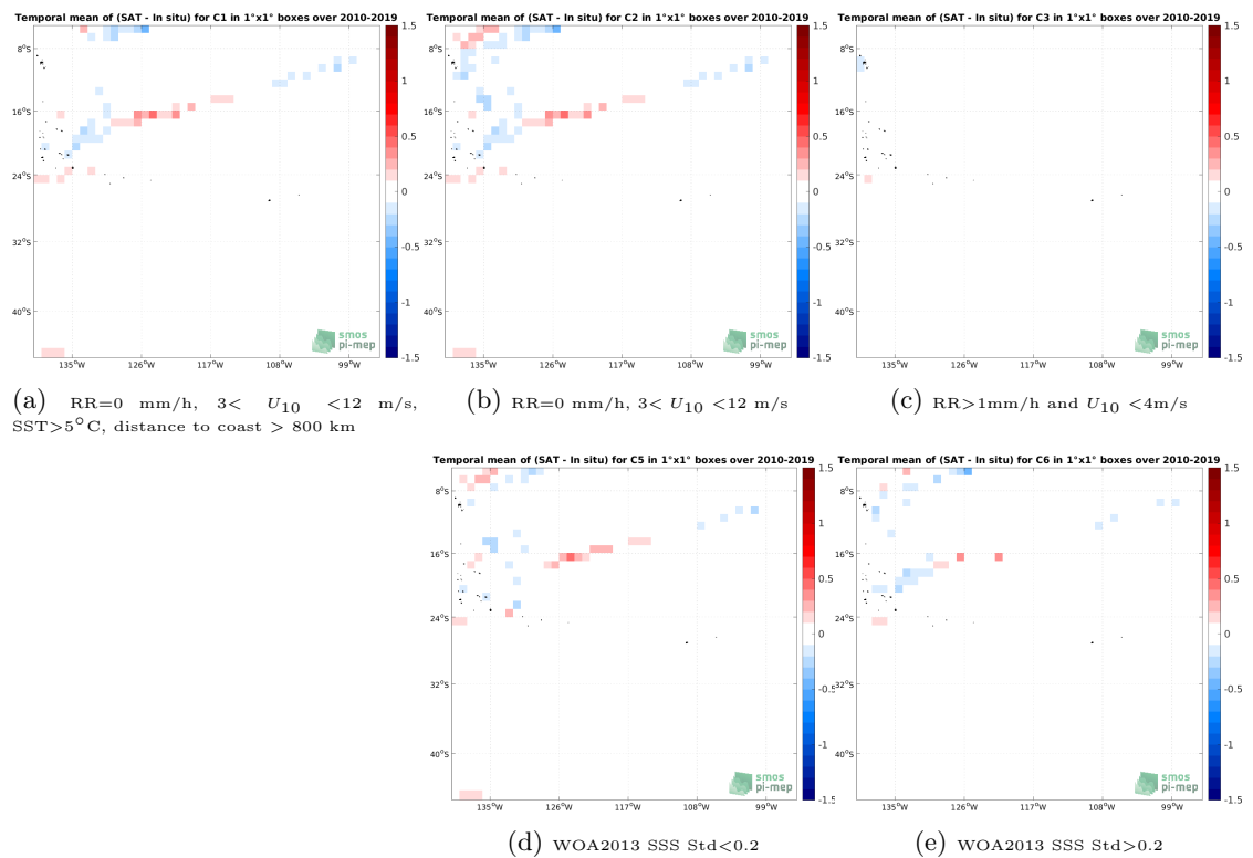
Figure 12: Temporal mean gridded over spatial boxes of size 1^\circ \times 1^\circ of \Delta SSS (SMOS SSS L3 v7 - 18 Days (CATDS-CECOS-LOCEAN) - TSG (GOSUD-Research-vessel)) for 5 different sub-datasets corresponding to:RR=0 mm/h, 3 < U_{10} < 12 m/s, SST >5^\circ\text{C} , distance to coast > 800 km (a), RR=0 mm/h, 3 < U_{10} < 12 m/s (b), RR >1 mm/h and U_{10} < 4 m/s (c), WOA2013 SSS Std <0.2 (d), WOA2013 SSS Std >0.2 (e).
