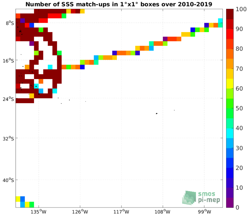
Figure 4: Number of SSS match-ups between TSG (GOSUD-Research-vessel) SSS and the SMOS SSS L3 v7 - 18 Days (CATDS-CECOS-LOCEAN) SSS product for the OTT zone Pi-MEP region over 1°x1° boxes and for the full satellite product period.
