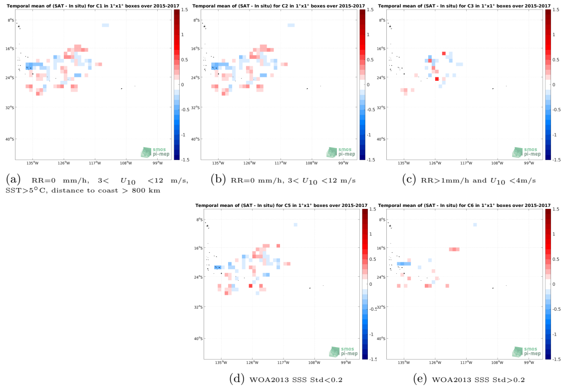
Figure 11: Temporal mean gridded over spatial boxes of size 1^{\circ}\times 1^{\circ} of \Delta\text{SSS} (SMOS SSS L3 v7 - 18 Days (CATDS-CECOS-LOCEAN) - Surface drifters) for 5 different subdatasets corresponding to:RR=0 mm/h, 3 < U_{10} < 12 m/s, SST >5^{\circ}\text{C} , distance to coast > 800 km (a), RR=0 mm/h, 3 < U_{10} < 12 m/s (b), RR >1 mm/h and U_{10} < 4 m/s (c), WOA2013 SSS Std <0.2 (d), WOA2013 SSS Std >0.2 (e).
