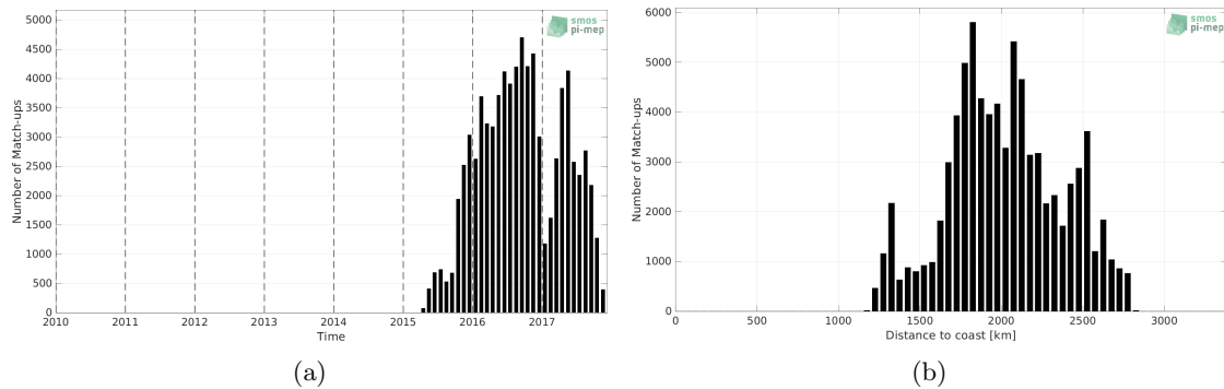
Figure 1: Number of match-ups between Surface drifters and SMOS SSS L3 v7 - 18 Days (CATDS-CECOS-LOCEAN) SSS as a function of time (a) and as function of the distance to coast (b) over the OTT zone Pi-MEP region and for the full satellite product period.
