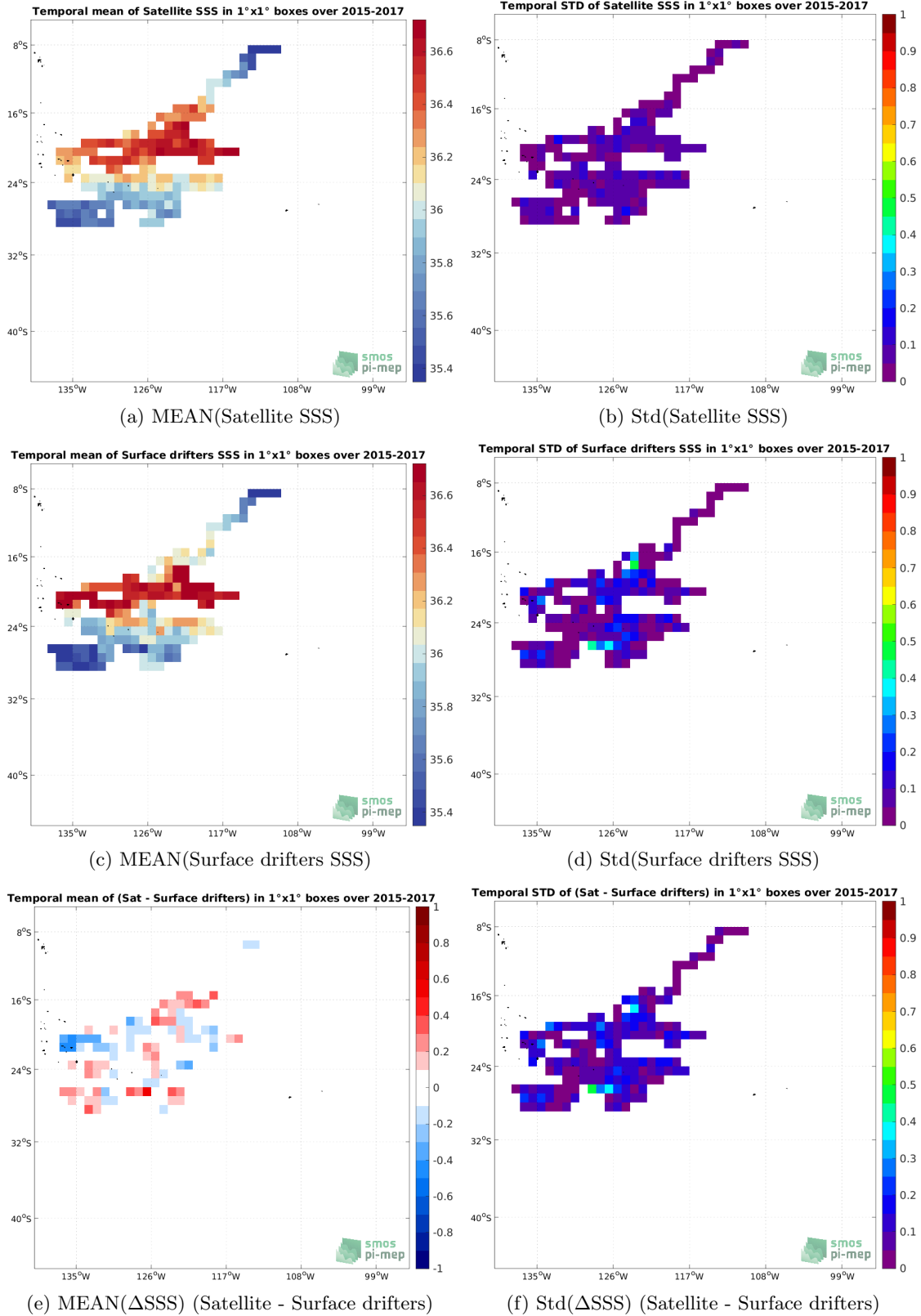
Figure 5: Temporal mean (left) and Std (right) of SSS from SMOS SSS L3 v7 - 18 Days (CATDS-CECOS-LOCEAN) (top), Surface drifters (middle), and of \Delta SSS (Satellite - Surface drifters). Only match-up pairs are used to generate these maps.
