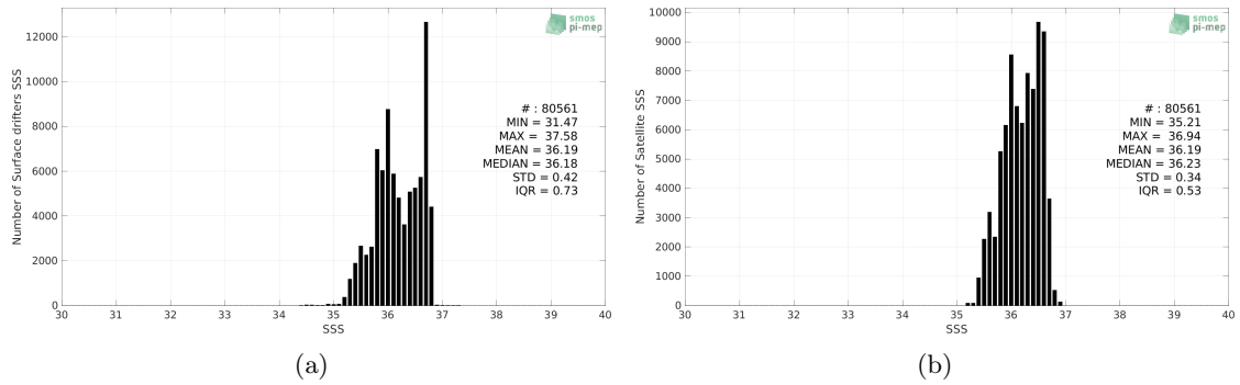
Figure 2: Histograms of SSS from Surface drifters (a) and SMOS SSS L3 v7 - 18 Days (CATDS-CECOS-LOCEAN) (b) considering all match-up pairs per bins of 0.1 over the OTT zone Pi-MEP region and for the full satellite product period.
