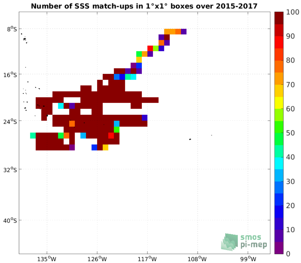
Figure 3: Number of SSS match-ups between Surface drifters SSS and the SMOS SSS L3 v7 - 18 Days (CATDS-CECOS-LOCEAN) SSS product for the OTT zone Pi-MEP region over 1°x1° boxes and for the full satellite product period.
