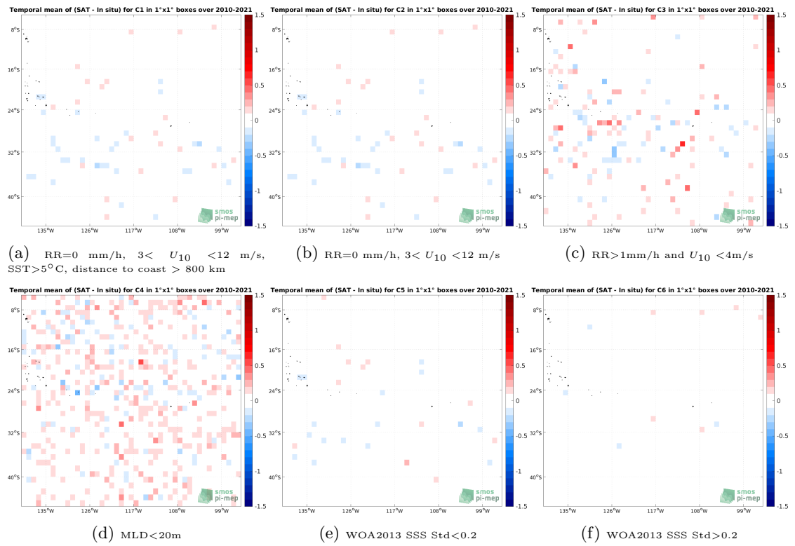
Figure 12: Temporal mean gridded over spatial boxes of size 1^\circ \times 1^\circ of \Delta SSS (SMOS SSS L3 v7 - 18 Days (CATDS-CECOS-LOCEAN) - Argo) for 6 different subdatasets corresponding to:RR=0 mm/h, 3 < U_{10} < 12 m/s, SST >5^\circ C, distance to coast > 800 km (a), RR=0 mm/h, 3 < U_{10} < 12 m/s (b), RR >1 mm/h and U_{10} < 4 m/s (c),MLD <20 m (d),WOA2013 SSS Std <0.2 (e),WOA2013 SSS Std >0.2 (f).
