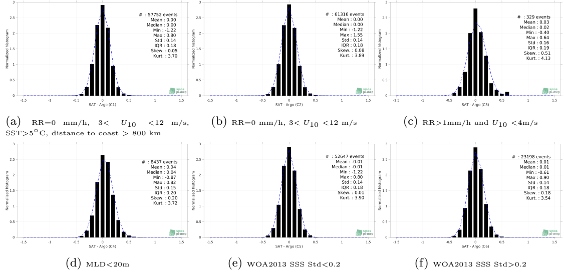
Figure 13: Normalized histogram of \Delta SSS (SMOS SSS L3 v7 - 18 Days (CATDS-CECOS-LOCEAN) - Argo) for 6 different subdatasets corresponding to: RR=0 mm/h, 3 < U_{10} < 12 m/s, SST > 5°C, distance to coast > 800 km (a), RR=0 mm/h, 3 < U_{10} < 12 m/s (b), RR > 1mm/h and U_{10} < 4 m/s (c), MLD < 20m (d), WOA2013 SSS Std < 0.2 (e), WOA2013 SSS Std > 0.2 (f).
