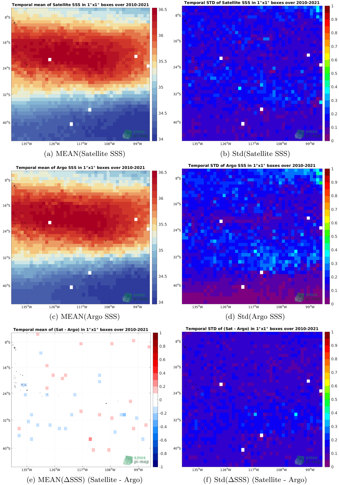
Figure 6: Temporal mean (left) and Std (right) of SSS from SMOS SSS L3 v7 - 18 Days (CATDS-CECOS-LOCEAN) (top), Argo (middle), and of \Delta SSS (Satellite - Argo). Only match-up pairs are used to generate these maps.
