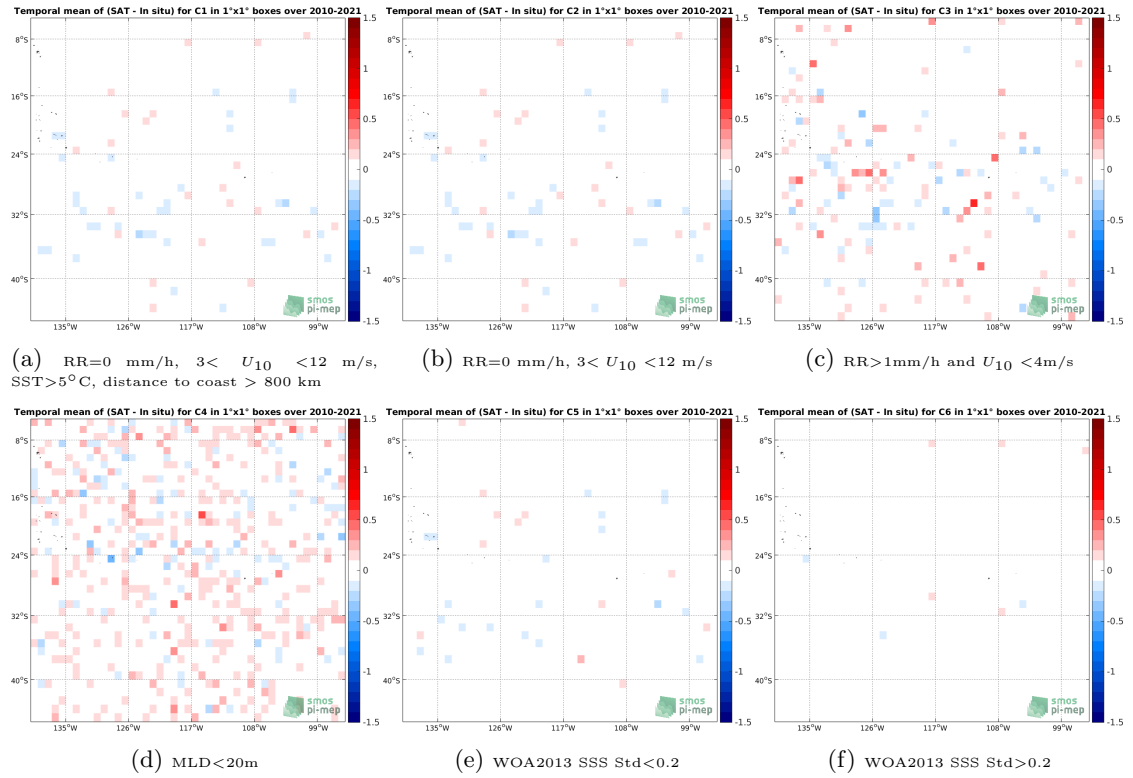
Figure 12: Temporal mean gridded over spatial boxes of size 1^\circ \times 1^\circ of \Delta SSS (SMOS SSS L3 v7 - 18 Days (CATDS-CECOS-LOCEAN) - Argo) for 6 different subdatasets corresponding to:RR=0 mm/h, 3 < U_{10} < 12 m/s, SST >5^\circ C, distance to coast > 800 km (a), RR=0 mm/h, 3 < U_{10} < 12 m/s (b), RR >1 mm/h and U_{10} < 4 m/s (c),MLD <20 m (d),WOA2013 SSS Std <0.2 (e),WOA2013 SSS Std >0.2 (f).
