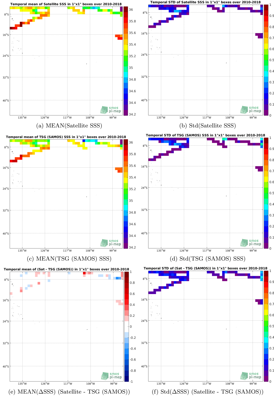
Figure 6: Temporal mean (left) and Std (right) of SSS from SMOS SSS L3 v5 - 9 Days (CATDS-CECOS-LOCEAN) (top), TSG (SAMOS) (middle), and of \Delta SSS (Satellite - TSG (SAMOS)). Only match-up pairs are used to generate these maps.
