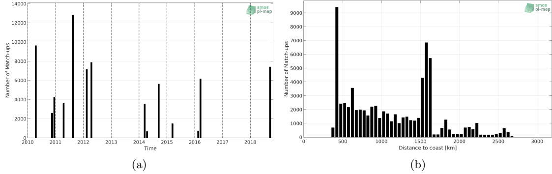
Figure 1: Number of match-ups between TSG (SAMOS) and SMOS SSS L3 v5 - 9 Days (CATDS-CECOS-LOCEAN) SSS as a function of time (a) and as function of the distance to coast (b) over the OTT zone Pi-MEP region and for the full satellite product period.
