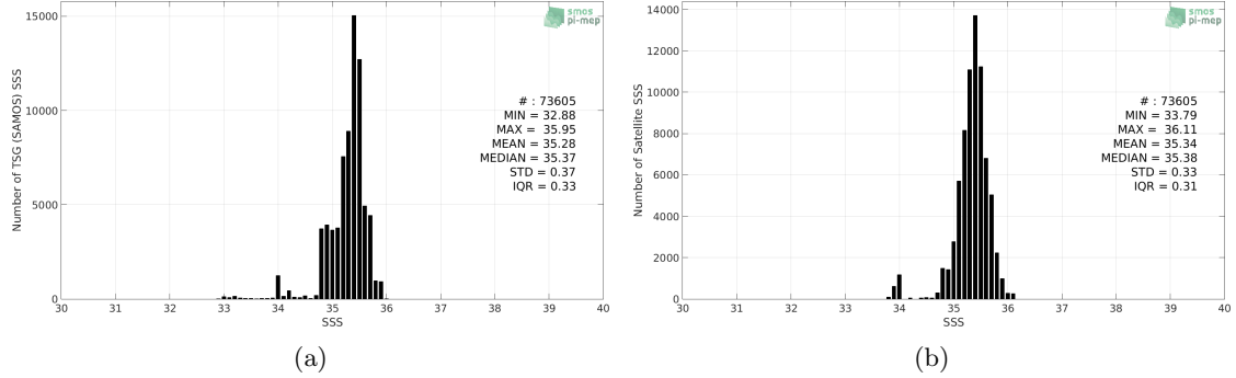
Figure 2: Histograms of SSS from TSG (SAMOS) (a) and SMOS SSS L3 v5 - 9 Days (CATDS-CECOS-LOCEAN) (b) considering all match-up pairs per bins of 0.1 over the OTT zone Pi-MEP region and for the full satellite product period.
