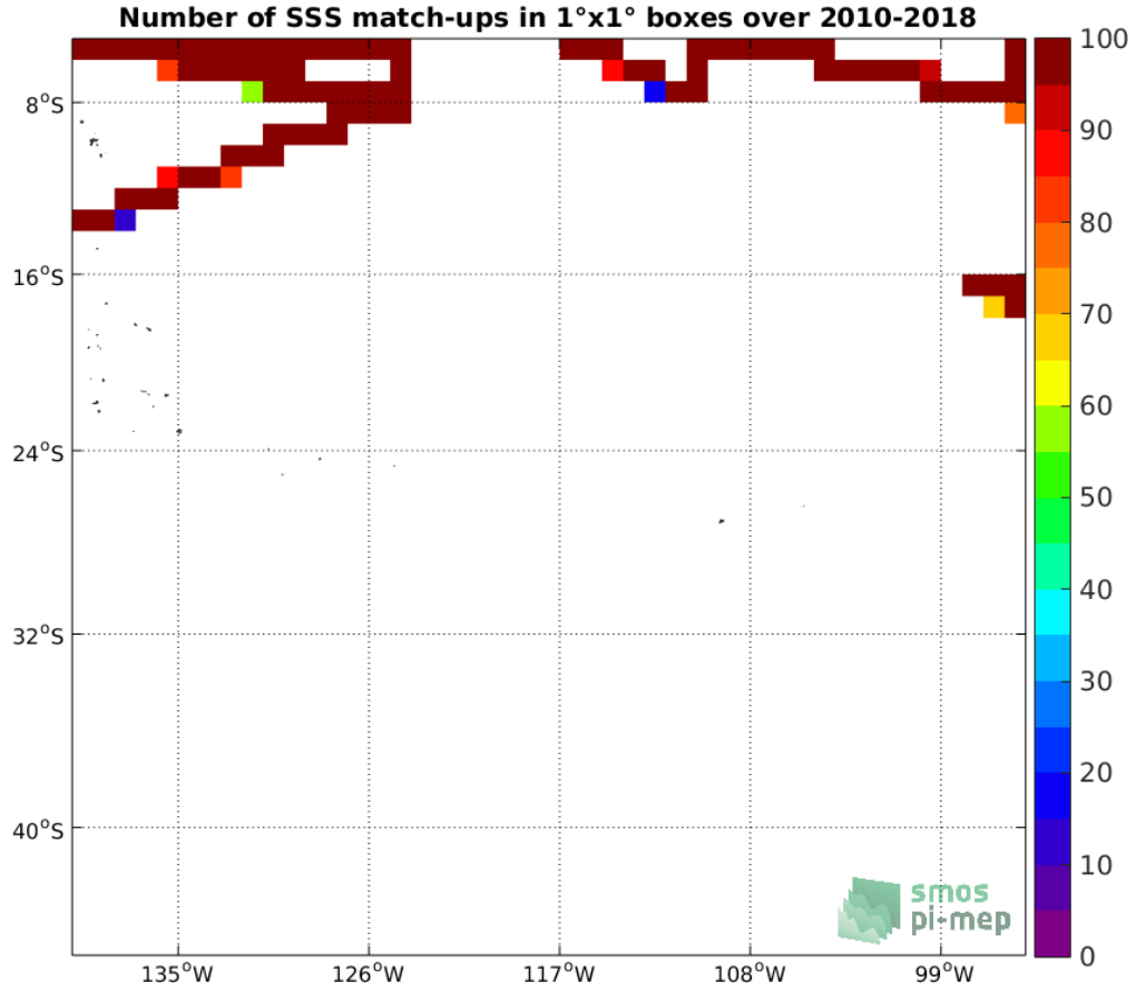
Figure 4: Number of SSS match-ups between TSG (SAMOS) SSS and the SMOS SSS L3 v5 - 9 Days (CATDS-CECOS-LOCEAN) SSS product for the OTT zone Pi-MEP region over 1^\circ \times 1^\circ boxes and for the full satellite product period.
