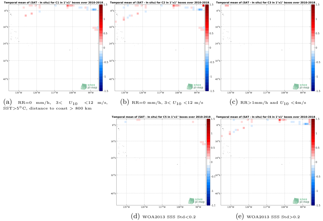
Figure 12: Temporal mean gridded over spatial boxes of size 1^{\circ}\times 1^{\circ} of \Delta\text{SSS} (SMOS SSS L3 v5 - 9 Days (CATDS-CECOS-LOCEAN) - TSG (SAMOS)) for 5 different subdatasets corresponding to: RR=0 mm/h, 3 < U_{10} < 12 m/s, SST >5^{\circ}\text{C} , distance to coast > 800 km (a), RR=0 mm/h, 3 < U_{10} < 12 m/s (b), RR >1 mm/h and U_{10} < 4 m/s (c), WOA2013 SSS Std <0.2 (d), WOA2013 SSS Std >0.2 (e).
