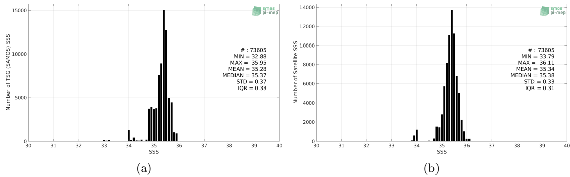
Figure 2: Histograms of SSS from TSG (SAMOS) (a) and SMOS SSS L3 v5 - 9 Days (CATDS-CECOS-LOCEAN) (b) considering all match-up pairs per bins of 0.1 over the OTT zone Pi-MEP region and for the full satellite product period.
