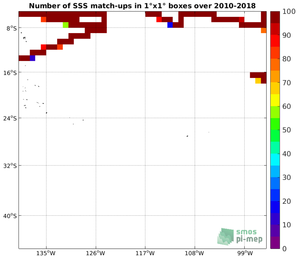
Figure 4: Number of SSS match-ups between TSG (SAMOS) SSS and the SMOS SSS L3 v5 - 9 Days (CATDS-CECOS-LOCEAN) SSS product for the OTT zone Pi-MEP region over 1°x1° boxes and for the full satellite product period.
