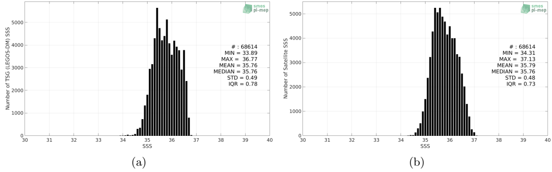
Figure 2: Histograms of SSS from TSG (LEGOS-DM) (a) and SMOS SSS L3 v5 - 9 Days (CATDS-CECOS-LOCEAN) (b) considering all match-up pairs per bins of 0.1 over the OTT zone Pi-MEP region and for the full satellite product period.
