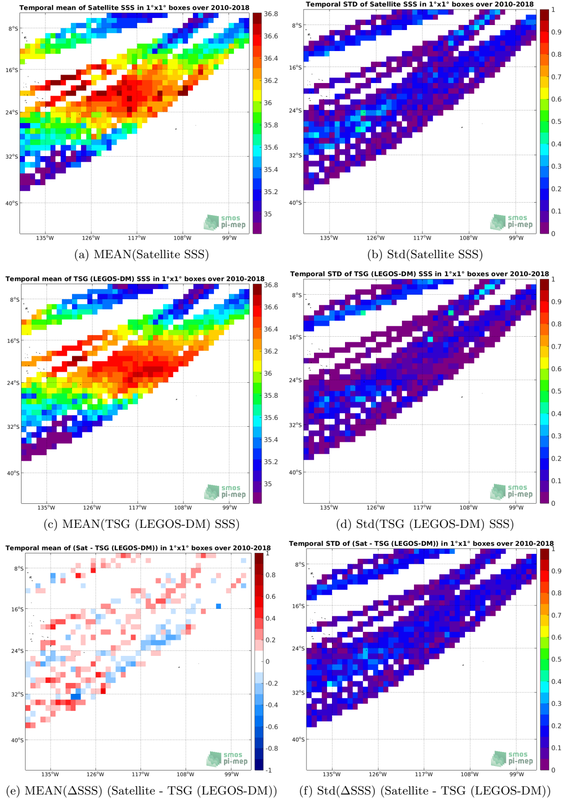
Figure 6: Temporal mean (left) and Std (right) of SSS from SMOS SSS L3 v5 - 9 Days (CATDS-CECOS-LOCEAN) (top), TSG (LEGOS-DM) (middle), and of \Delta SSS (Satellite - TSG (LEGOS-DM)). Only match-up pairs are used to generate these maps.
