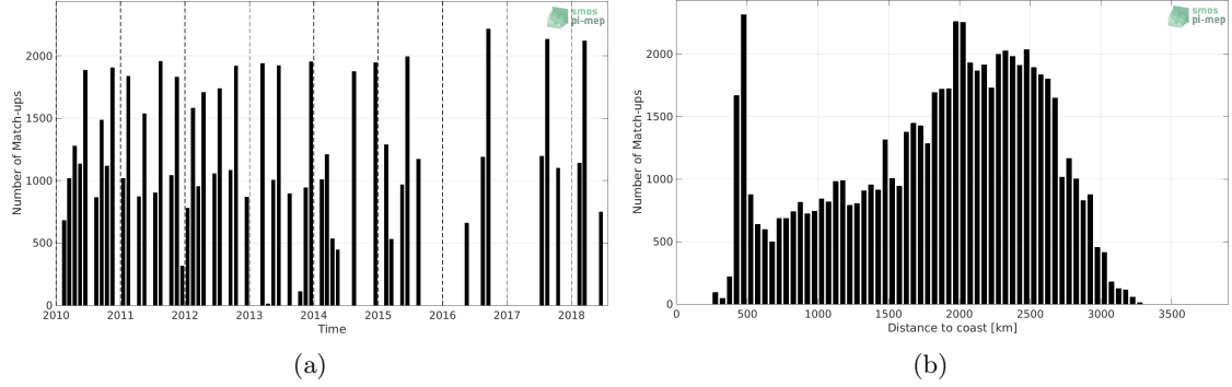
Figure 1: Number of match-ups between TSG (LEGOS-DM) and SMOS SSS L3 v5 - 9 Days (CATDS-CECOS-LOCEAN) SSS as a function of time (a) and as function of the distance to coast (b) over the OTT zone Pi-MEP region and for the full satellite product period.
