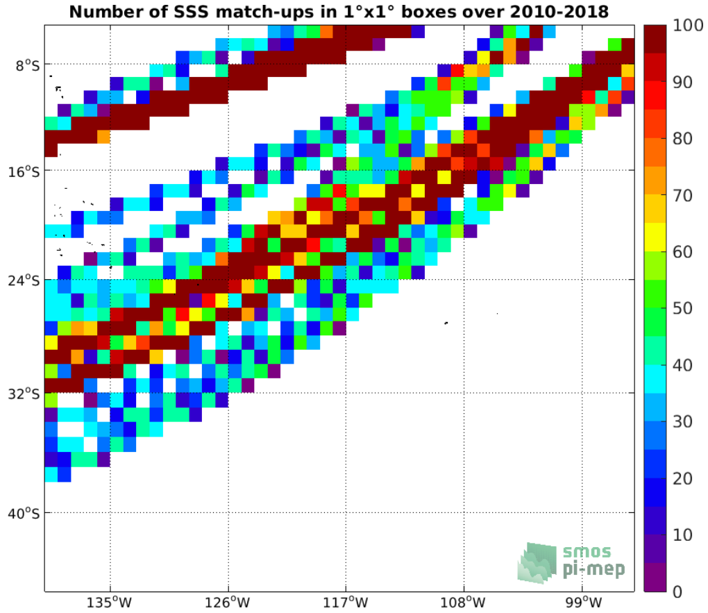
Figure 4: Number of SSS match-ups between TSG (LEGOS-DM) SSS and the SMOS SSS L3 v5 - 9 Days (CATDS-CECOS-LOCEAN) SSS product for the OTT zone Pi-MEP region over 1°x1° boxes and for the full satellite product period.
