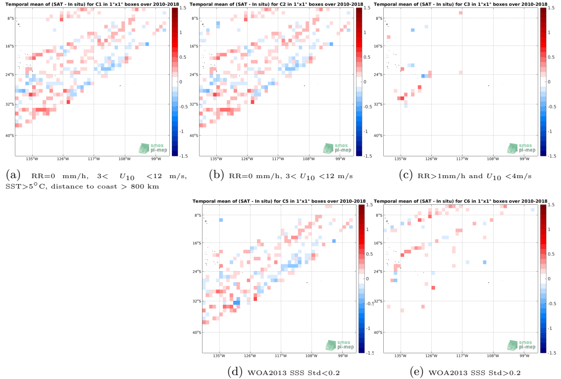
Figure 12: Temporal mean gridded over spatial boxes of size 1^{\circ}\times 1^{\circ} of \Delta\text{SSS} (SMOS SSS L3 v5 - 9 Days (CATDS-CECOS-LOCEAN) - TSG (LEGOS-DM)) for 5 different subdatasets corresponding to: RR=0 mm/h, 3 < U_{10} < 12 m/s, SST >5^{\circ}\text{C} , distance to coast > 800 km (a), RR=0 mm/h, 3 < U_{10} < 12 m/s (b), RR >1 mm/h and U_{10} < 4 m/s (c), WOA2013 SSS Std <0.2 (d), WOA2013 SSS Std >0.2 (e).
