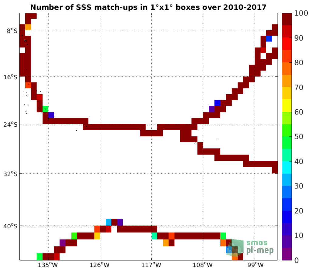
Figure 4: Number of SSS match-ups between TSG (GOSUD-Sailing-ship) SSS and the SMOS SSS L3 v5 - 9 Days (CATDS-CECOS-LOCEAN) SSS product for the OTT zone Pi-MEP region over 1°x1° boxes and for the full satellite product period.
