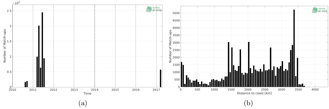
Figure 1: Number of match-ups between TSG (GOSUD-Sailing-ship) and SMOS SSS L3 v5 - 9 Days (CATDS-CECOS-LOCEAN) SSS as a function of time (a) and as function of the distance to coast (b) over the OTT zone Pi-MEP region and for the full satellite product period.
