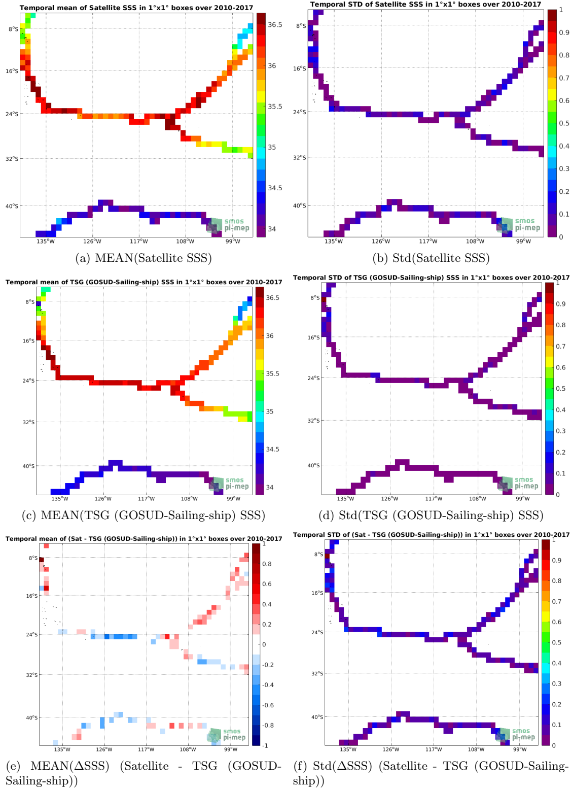
Figure 6: Temporal mean (left) and Std (right) of SSS from SMOS SSS L3 v5 - 9 Days (CATDS-CECOS-LOCEAN) (top), TSG (GOSUD-Sailing-ship) (middle), and of \Delta SSS (Satellite - TSG (GOSUD-Sailing-ship)). Only match-up pairs are used to generate these maps.
