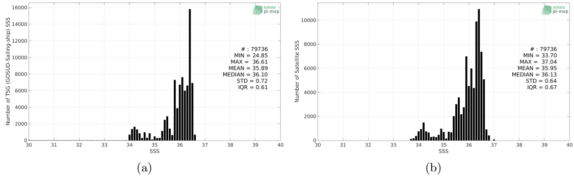
Figure 2: Histograms of SSS from TSG (GOSUD-Sailing-ship) (a) and SMOS SSS L3 v5 - 9 Days (CATDS-CECOS-LOCEAN) (b) considering all match-up pairs per bins of 0.1 over the OTT zone Pi-MEP region and for the full satellite product period.
