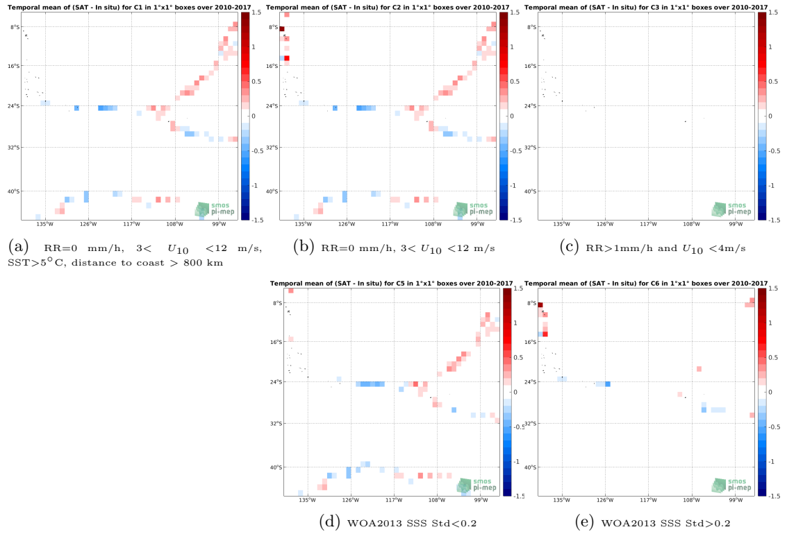
Figure 12: Temporal mean gridded over spatial boxes of size 1^\circ \times 1^\circ of \Delta SSS (SMOS SSS L3 v5 - 9 Days (CATDS-CECOS-LOCEAN) - TSG (GOSUD-Sailing-ship)) for 5 different subdatasets corresponding to: RR=0 mm/h, 3 < U_{10} < 12 m/s, SST > 5^\circ C , distance to coast > 800 km (a), RR=0 mm/h, 3 < U_{10} < 12 m/s (b), RR > 1 mm/h and U_{10} < 4 m/s (c), WOA2013 SSS Std < 0.2 (d), WOA2013 SSS Std > 0.2 (e).
