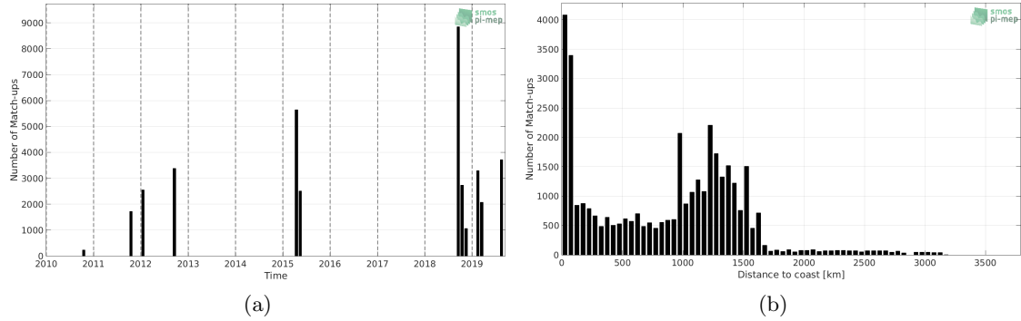
Figure 1: Number of match-ups between TSG (GOSUD-Research-vessel) and SMOS SSS L3 v5 - 9 Days (CATDS-CECOS-LOCEAN) SSS as a function of time (a) and as function of the distance to coast (b) over the OTT zone Pi-MEP region and for the full satellite product period.
