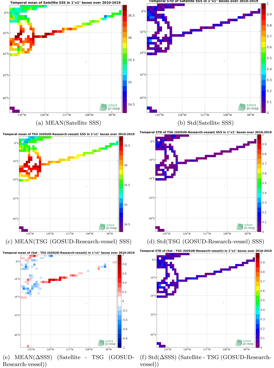
Figure 6: Temporal mean (left) and Std (right) of SSS from SMOS SSS L3 v5 - 9 Days (CATDS-CECOS-LOCEAN) (top), TSG (GOSUD-Research-vessel) (middle), and of \Delta SSS (Satellite - TSG (GOSUD-Research-vessel)). Only match-up pairs are used to generate these maps.
