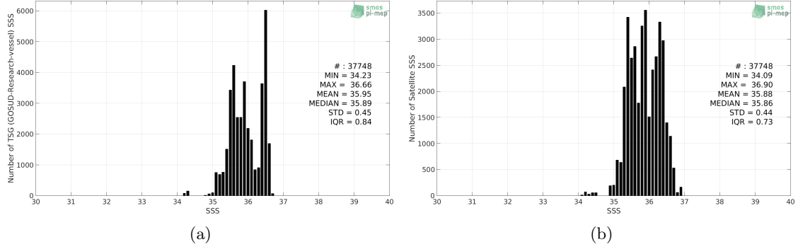
Figure 2: Histograms of SSS from TSG (GOSUD-Research-vessel) (a) and SMOS SSS L3 v5 - 9 Days (CATDS-CECOS-LOCEAN) (b) considering all match-up pairs per bins of 0.1 over the OTT zone Pi-MEP region and for the full satellite product period.
