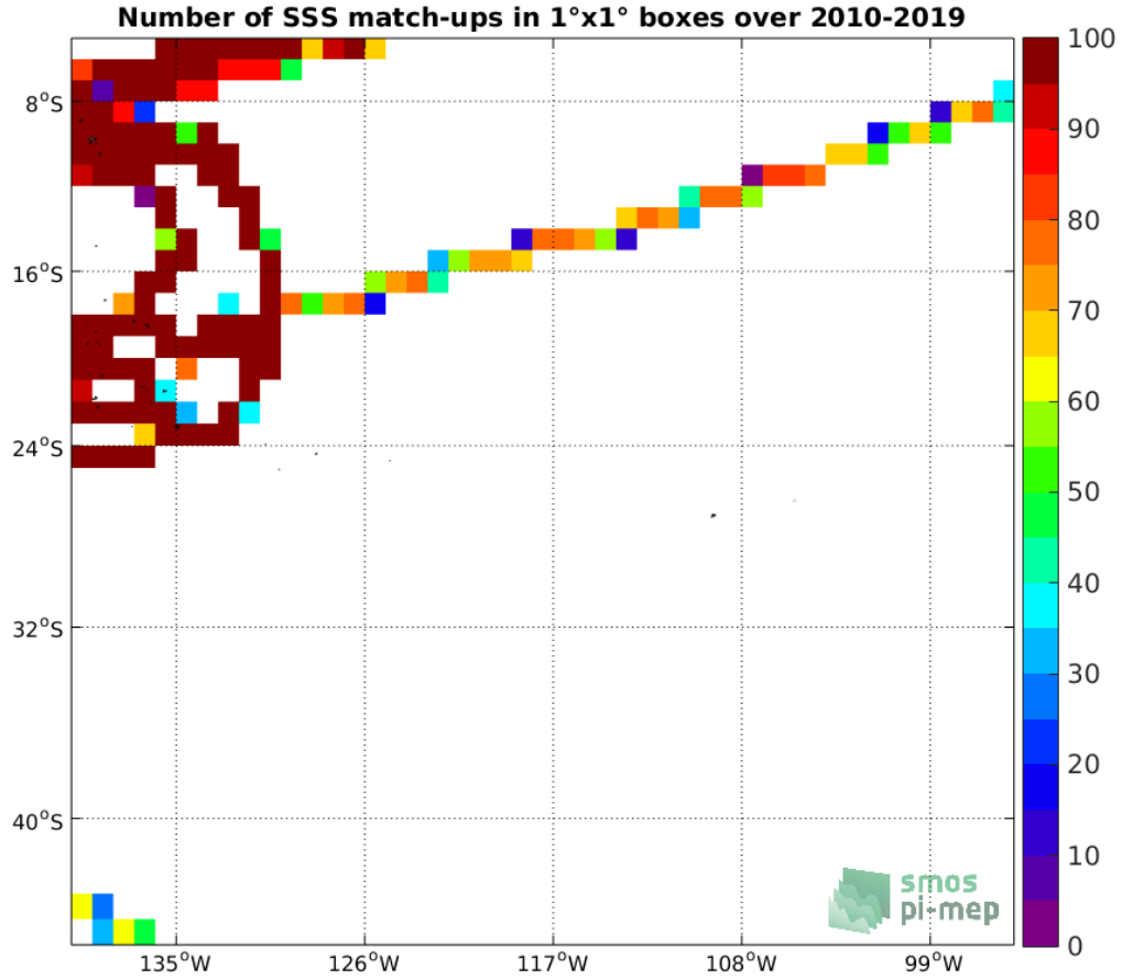
Figure 4: Number of SSS match-ups between TSG (GOSUD-Research-vessel) SSS and the SMOS SSS L3 v5 - 9 Days (CATDS-CECOS-LOCEAN) SSS product for the OTT zone Pi-MEP region over 1°x1° boxes and for the full satellite product period.
