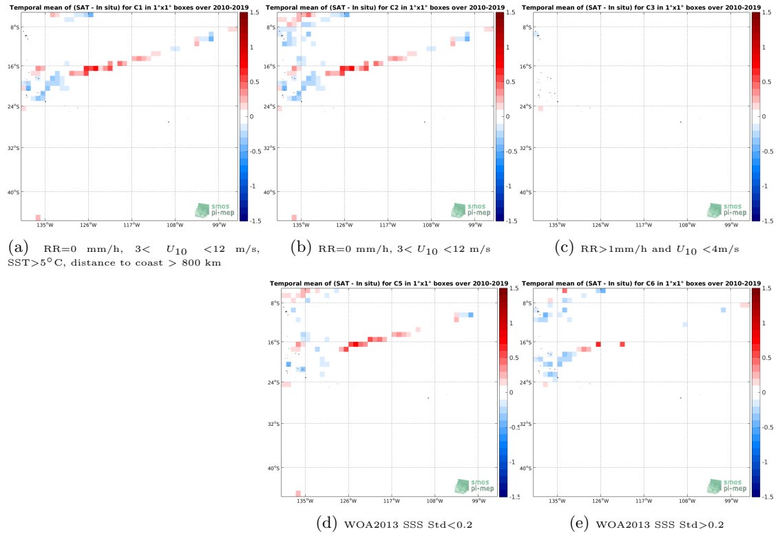
Figure 12: Temporal mean gridded over spatial boxes of size 1^\circ \times 1^\circ of \Delta SSS (SMOS SSS L3 v5 - 9 Days (CATDS-CECOS-LOCEAN) - TSG (GOSUD-Research-vessel)) for 5 different subdatasets corresponding to: RR=0 mm/h, 3 < U_{10} < 12 m/s, SST > 5^\circ C , distance to coast > 800 km (a), RR=0 mm/h, 3 < U_{10} < 12 m/s (b), RR > 1 mm/h and U_{10} < 4 m/s (c), WOA2013 SSS Std < 0.2 (d), WOA2013 SSS Std > 0.2 (e).
