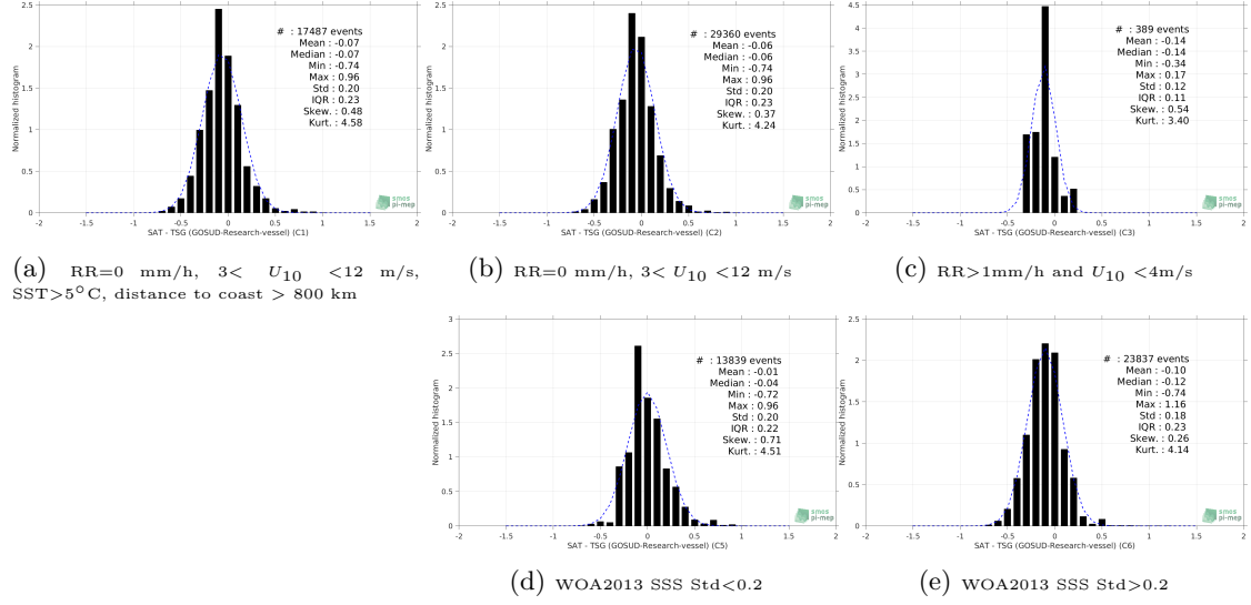
Figure 13: Normalized histogram of \Delta\text{SSS} (SMOS SSS L3 v5 - 9 Days (CATDS-CECOS-LOCEAN) - TSG (GOSUD-Research-vessel)) for 5 different subdatasets corresponding to: RR=0 mm/h, 3 < U_{10} < 12 m/s, SST > 5^\circ\text{C} , distance to coast > 800 km (a), RR=0 mm/h, 3 < U_{10} < 12 m/s (b), RR > 1 mm/h and U_{10} < 4 m/s (c), WOA2013 SSS Std < 0.2 (d), WOA2013 SSS Std > 0.2 (e).
