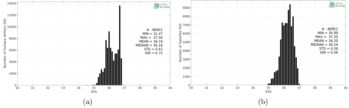
Figure 2: Histograms of SSS from Surface drifters (a) and SMOS SSS L3 v5 - 9 Days (CATDS-CECOS-LOCEAN) (b) considering all match-up pairs per bins of 0.1 over the OTT zone Pi-MEP region and for the full satellite product period.
