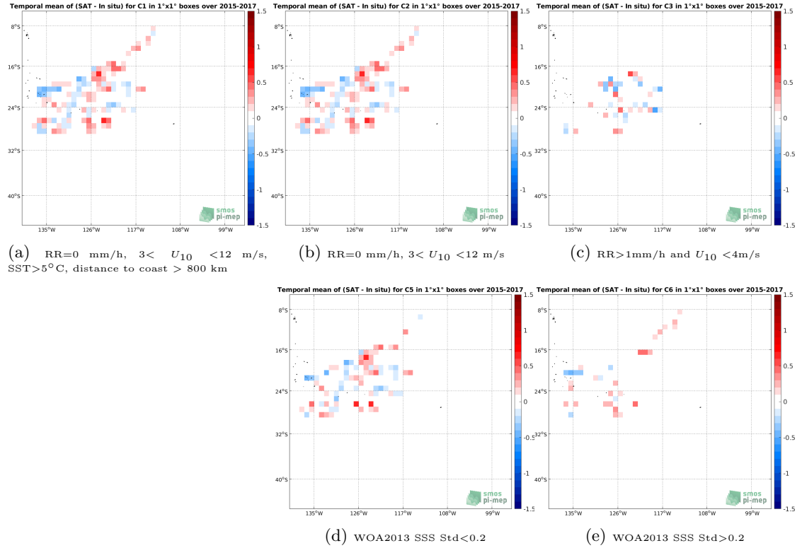
Figure 11: Temporal mean gridded over spatial boxes of size 1^{\circ}\times 1^{\circ} of \Delta\text{SSS} (SMOS SSS L3 v5 - 9 Days (CATDS-CECOS-LOCEAN) - Surface drifters) for 5 different subdatasets corresponding to: RR=0 mm/h, 3 < U_{10} < 12 m/s, SST >5^{\circ}\text{C} , distance to coast > 800 km (a), RR=0 mm/h, 3 < U_{10} < 12 m/s (b), RR >1 mm/h and U_{10} < 4 m/s (c), WOA2013 SSS Std <0.2 (d), WOA2013 SSS Std >0.2 (e).
