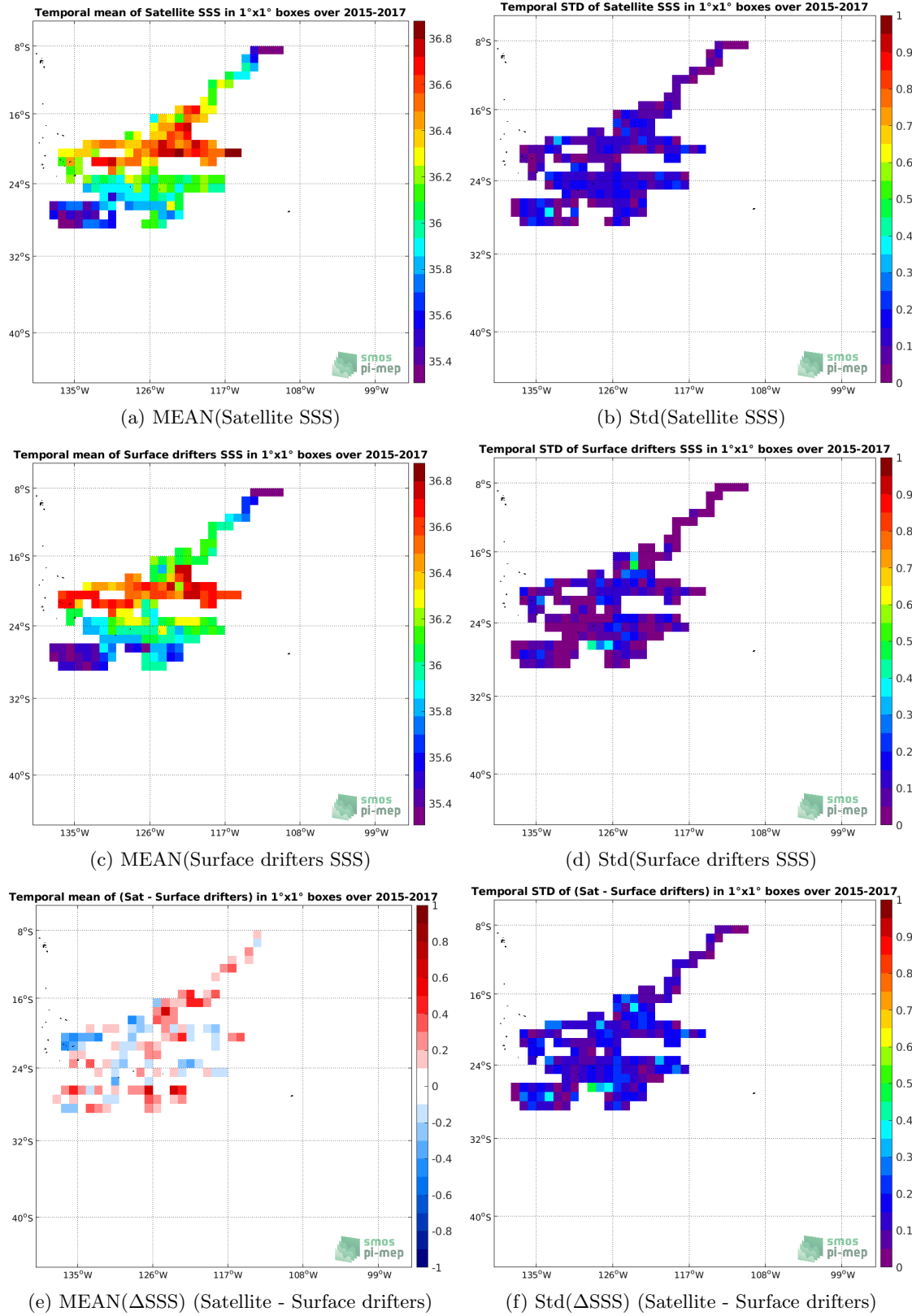
Figure 5: Temporal mean (left) and Std (right) of SSS from SMOS SSS L3 v5 - 9 Days (CATDS-CECOS-LOCEAN) (top), Surface drifters (middle), and of \Delta SSS (Satellite - Surface drifters). Only match-up pairs are used to generate these maps.
