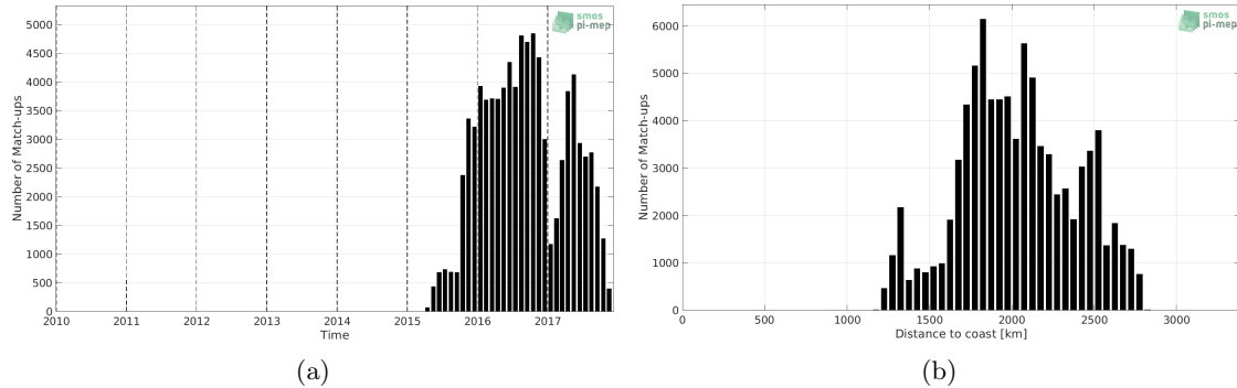
Figure 1: Number of match-ups between Surface drifters and SMOS SSS L3 v5 - 9 Days (CATDS-CECOS-LOCEAN) SSS as a function of time (a) and as function of the distance to coast (b) over the OTT zone Pi-MEP region and for the full satellite product period.
