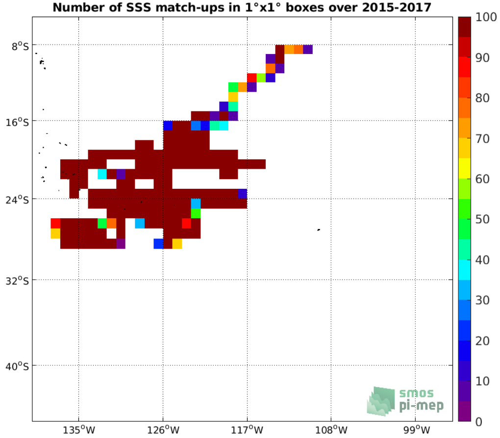
Figure 3: Number of SSS match-ups between Surface drifters SSS and the SMOS SSS L3 v5 - 9 Days (CATDS-CECOS-LOCEAN) SSS product for the OTT zone Pi-MEP region over 1^\circ \times 1^\circ boxes and for the full satellite product period.
