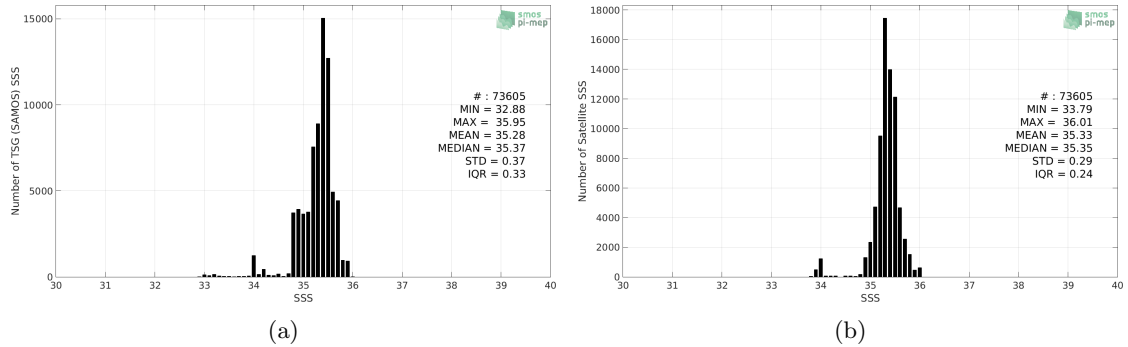
Figure 2: Histograms of SSS from TSG (SAMOS) (a) and SMOS SSS L3 v5 - 18 Days (CATDS-CECOS-LOCEAN) (b) considering all match-up pairs per bins of 0.1 over the OTT zone Pi-MEP region and for the full satellite product period.
