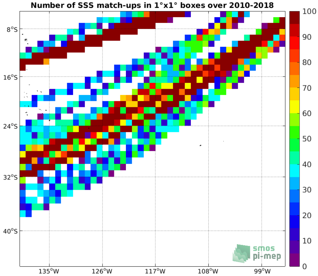
Figure 4: Number of SSS match-ups between TSG (LEGOS-DM) SSS and the SMOS SSS L3 v5 - 18 Days (CATDS-CECOS-LOCEAN) SSS product for the OTT zone Pi-MEP region over 1°x1° boxes and for the full satellite product period.
