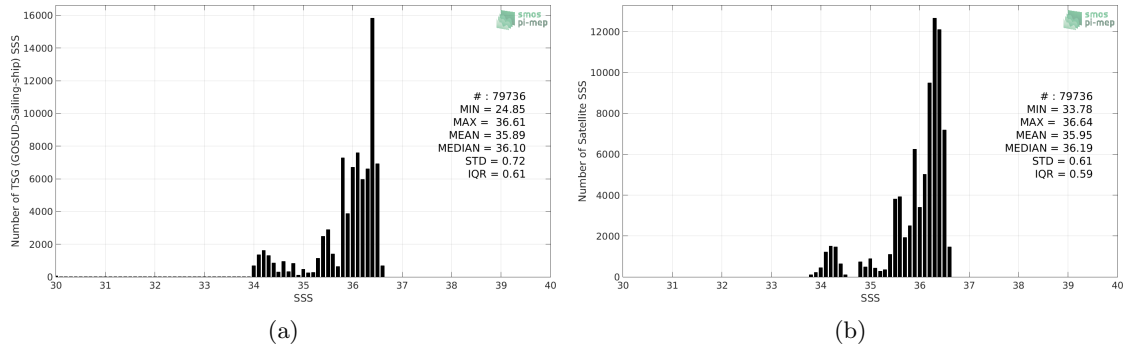
Figure 2: Histograms of SSS from TSG (GOSUD-Sailing-ship) (a) and SMOS SSS L3 v5 - 18 Days (CATDS-CECOS-LOCEAN) (b) considering all match-up pairs per bins of 0.1 over the OTT zone Pi-MEP region and for the full satellite product period.
