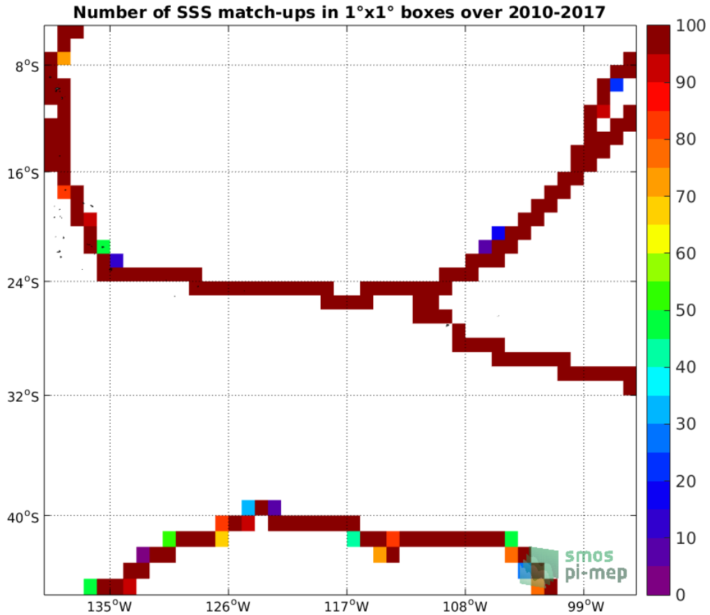
Figure 4: Number of SSS match-ups between TSG (GOSUD-Sailing-ship) SSS and the SMOS SSS L3 v5 - 18 Days (CATDS-CECOS-LOCEAN) SSS product for the OTT zone Pi-MEP region over 1^{\circ} \times 1^{\circ} boxes and for the full satellite product period.
