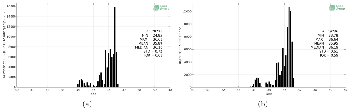
Figure 2: Histograms of SSS from TSG (GOSUD-Sailing-ship) (a) and SMOS SSS L3 v5 - 18 Days (CATDS-CECOS-LOCEAN) (b) considering all match-up pairs per bins of 0.1 over the OTT zone Pi-MEP region and for the full satellite product period.
