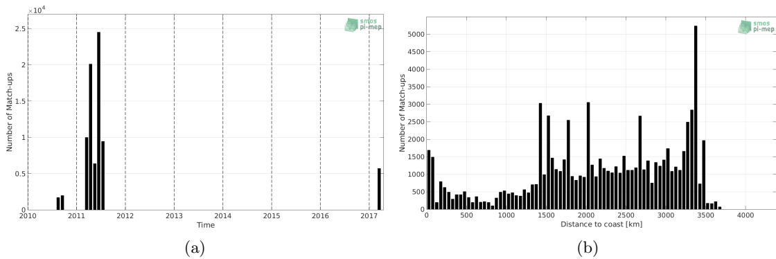
Figure 1: Number of match-ups between TSG (GOSUD-Sailing-ship) and SMOS SSS L3 v5 - 18 Days (CATDS-CECOS-LOCEAN) SSS as a function of time (a) and as function of the distance to coast (b) over the OTT zone Pi-MEP region and for the full satellite product period.
