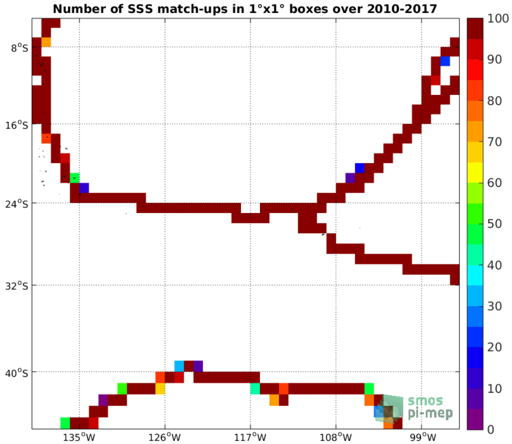
Figure 4: Number of SSS match-ups between TSG (GOSUD-Sailing-ship) SSS and the SMOS SSS L3 v5 - 18 Days (CATDS-CECOS-LOCEAN) SSS product for the OTT zone Pi-MEP region over 1^\circ \times 1^\circ boxes and for the full satellite product period.
