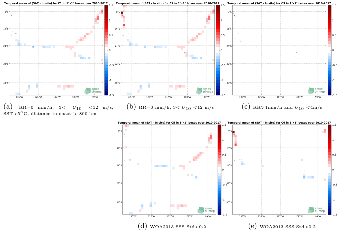
Figure 12: Temporal mean gridded over spatial boxes of size 1^\circ \times 1^\circ of \Delta\text{SSS} (SMOS SSS L3 v5 - 18 Days (CATDS-CECOS-LOCEAN) - TSG (GOSUD-Sailing-ship)) for 5 different subdatasets corresponding to: \text{RR}=0 \text{ mm/h} , 3 < U_{10} < 12 \text{ m/s} , \text{SST} > 5^\circ\text{C} , distance to coast > 800 \text{ km} (a), \text{RR}=0 \text{ mm/h} , 3 < U_{10} < 12 \text{ m/s} (b), \text{RR} > 1 \text{ mm/h} and U_{10} < 4 \text{ m/s} (c), WOA2013 SSS Std < 0.2 (d), WOA2013 SSS Std > 0.2 (e).
